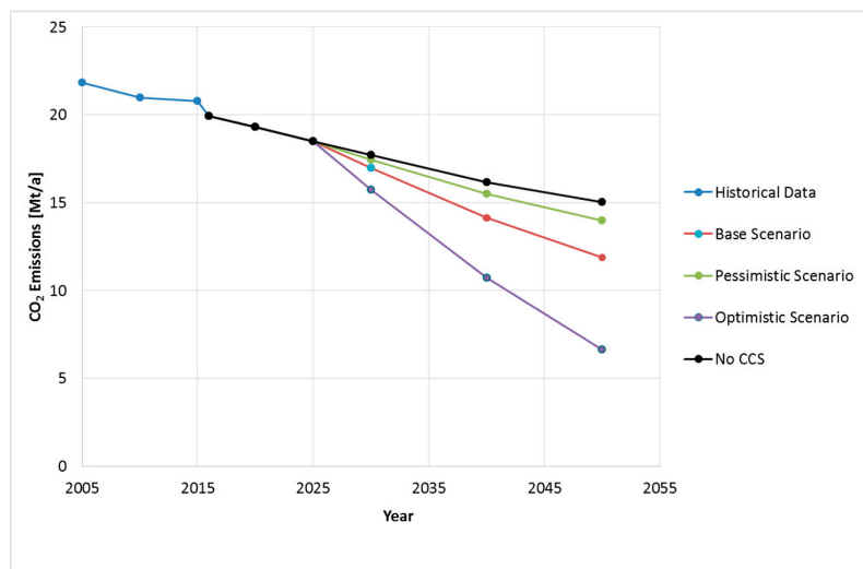
Figure 8. CCUS Germany: CO 2 emission projections for base clinker production (historical data from UBA/VDZ [21,51]).
