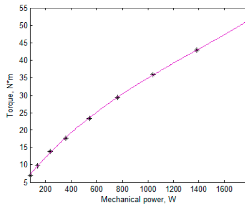
Figure 3. Loading torque of the wind turbine.
