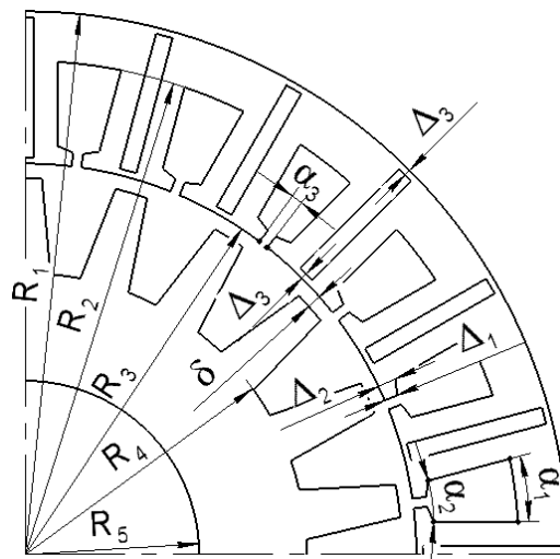
Figure 4. Optimization parameters.
