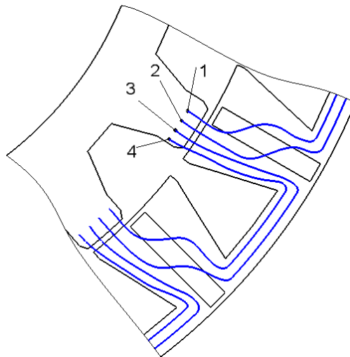
Figure 8. Flux flow in a flux-switching machine (FSM).
