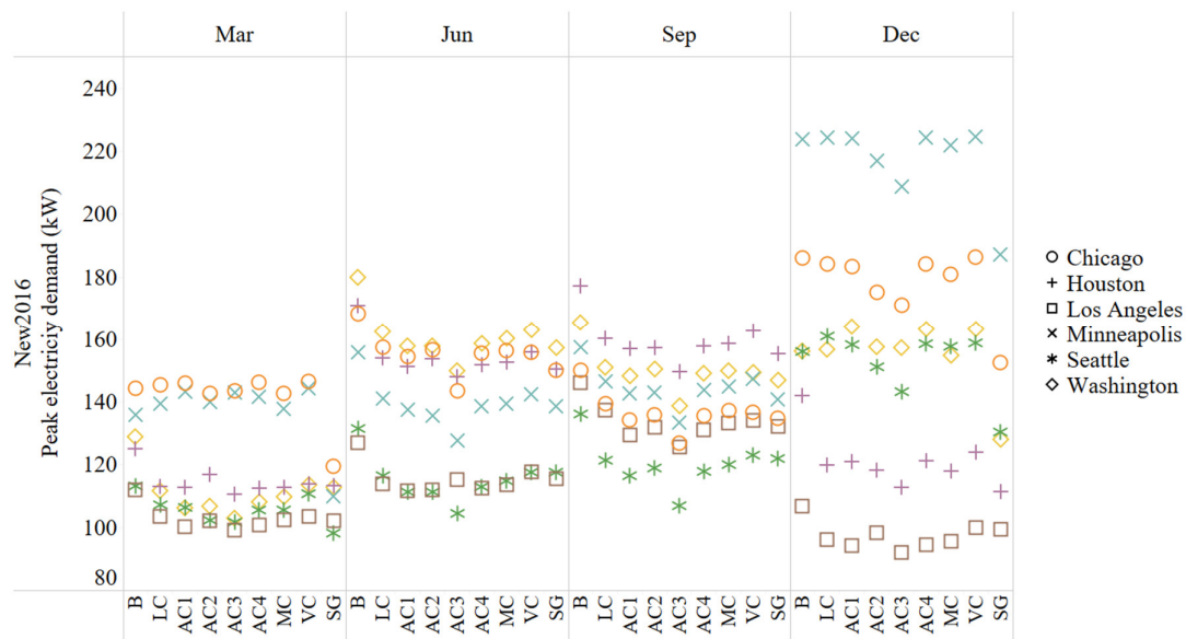
Figure 5. Peak demand for New2016 vintage.
