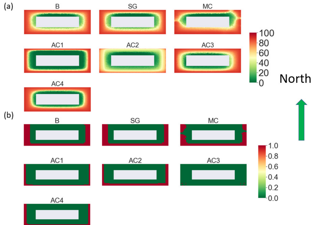
Figure 6. Daylight grid heat map for Chicago: (a) daylight autonomy, (b) annual sunlight exposure.
