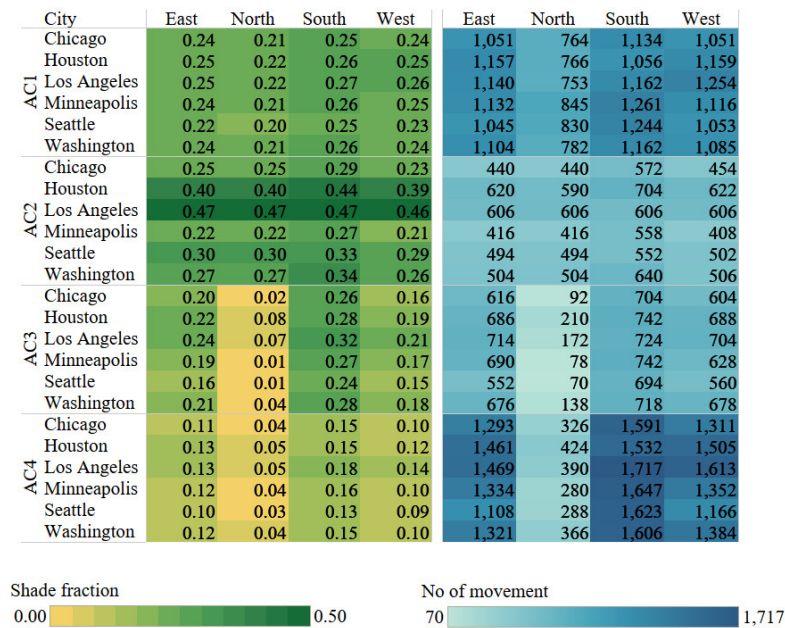
Figure 8. Fraction of window shaded by shading device and number of movements of shades for four different automated control strategies of roller shades, in different orientations at six different US locations.
