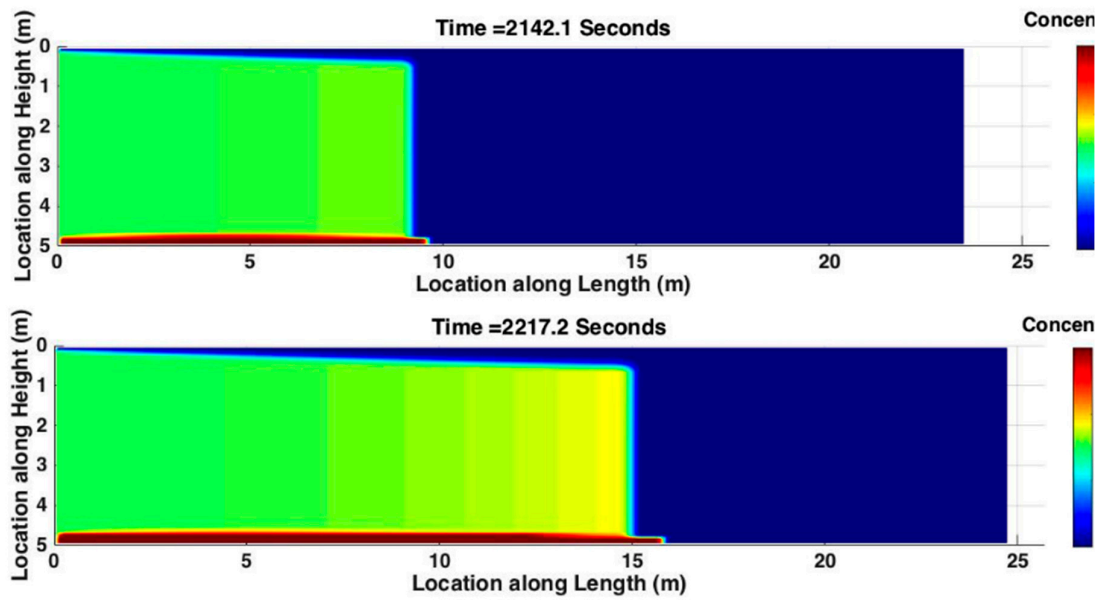
Figure 16. Proppant Concentration Distribution at Different Injection Times.
