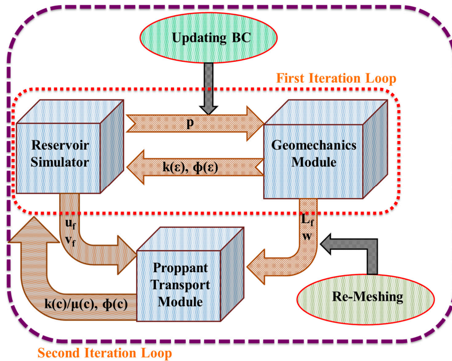
Figure 11. Information Transfer between the Modules.
