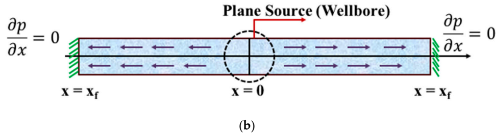
Figure 8. Geometry of the Verification Model: (a) Reservoir, (b) Fracture.
