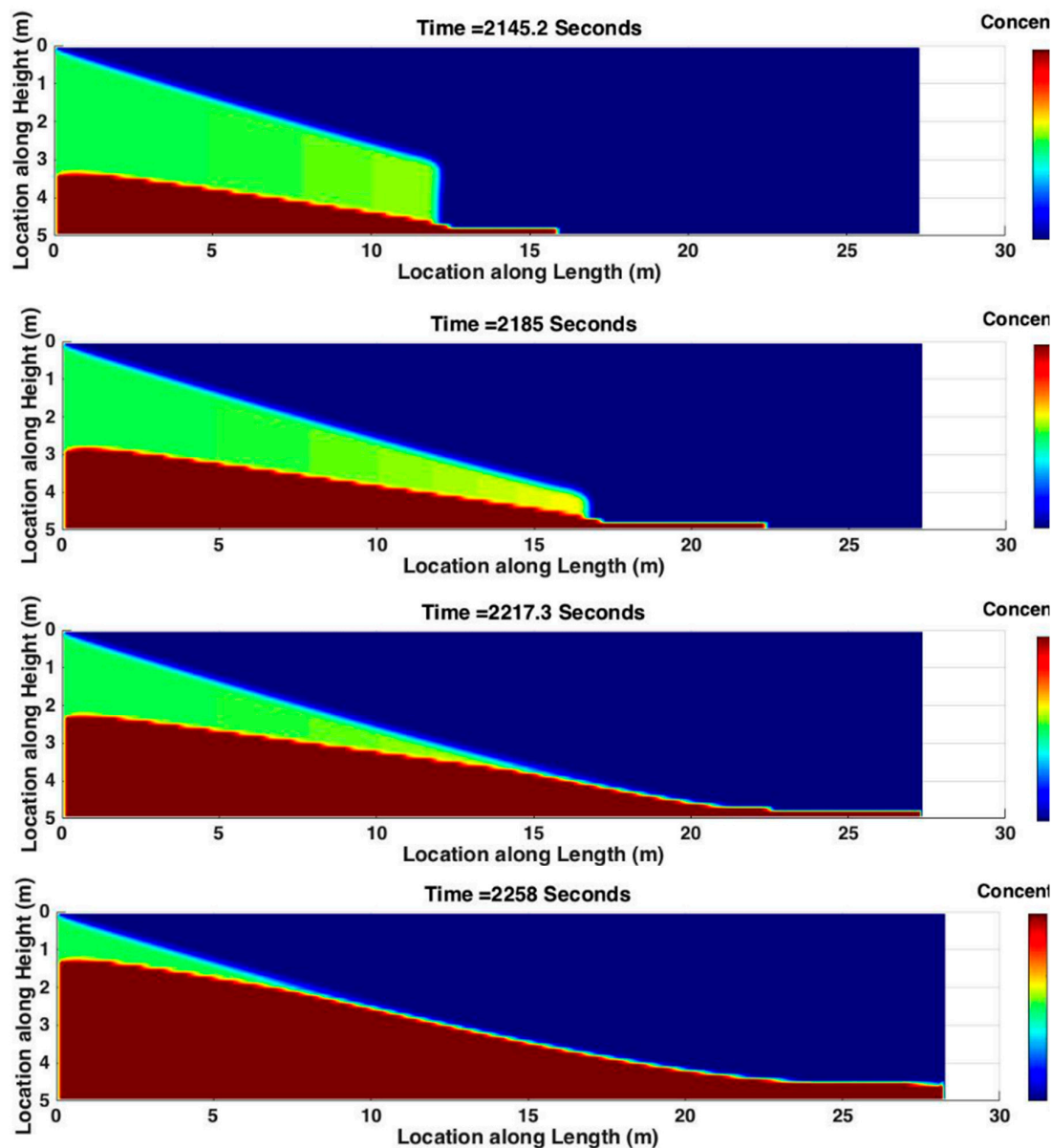
Figure 26. Tip Screen-out in Low Viscosity Fluid.
