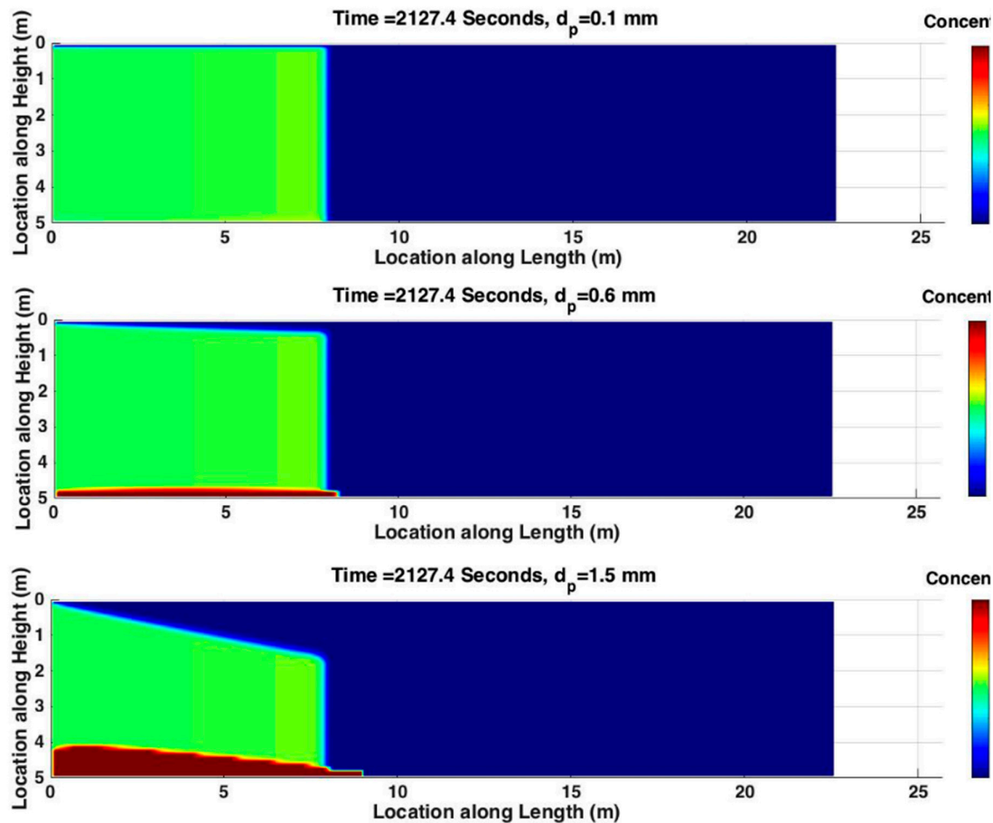
Figure 22. Proppant Distribution Concentration for Different Proppant Diameters.
