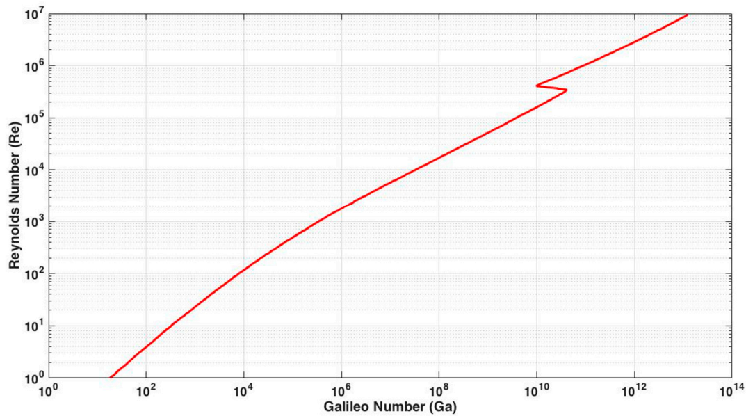
Figure 20. Standard Drag Curve.
