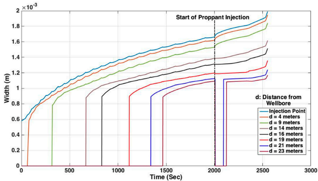
Figure 15. Fracture Width Variation through Time.
