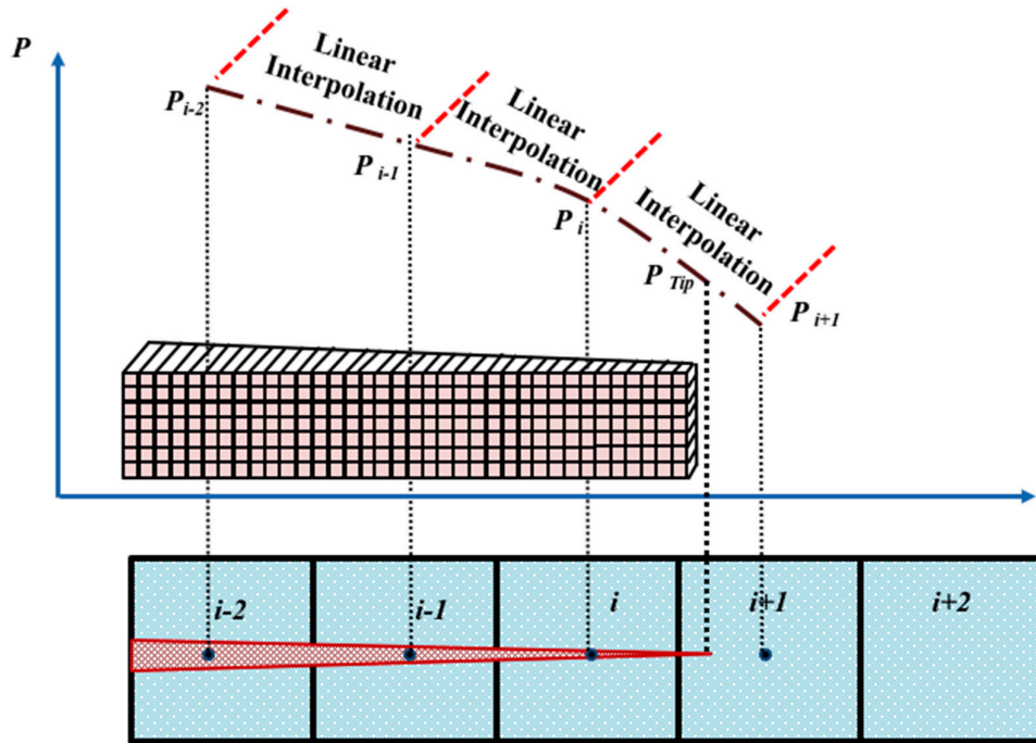
Figure 4. Linear Interpolation of Pressure at the Fracture Tip.
