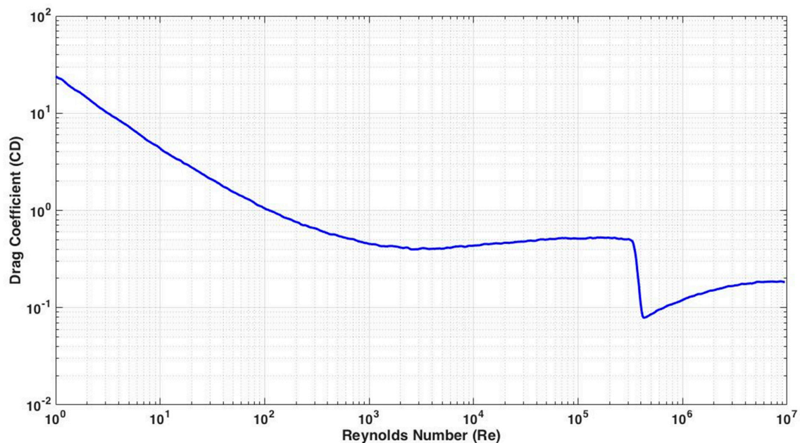
Figure 19. Standard Drag Curve.
