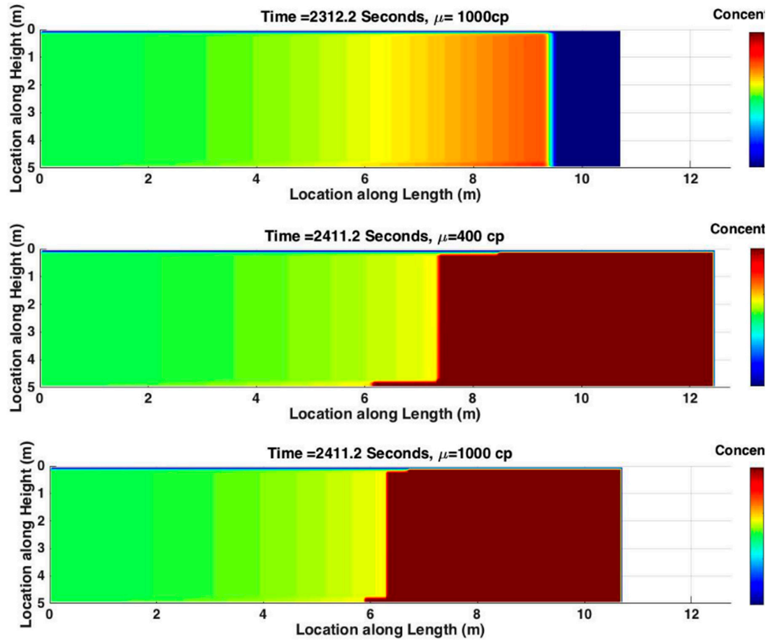
Figure 24. Proppant Distribution Concentration for Different Carrying Fluid Viscosities.
