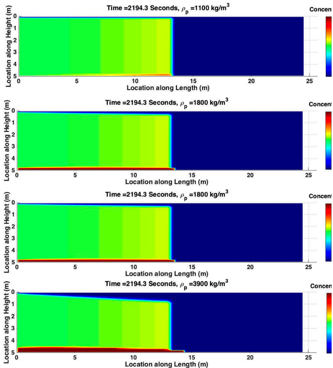
Figure 21. Proppant Distribution Concentration for Different Proppant Densities.
