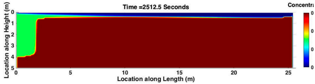
Figure 17. Proppant Concentration Distribution at Different Injection Times.
