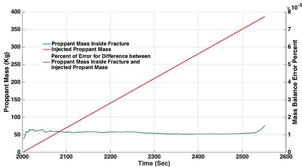
Figure 18. Global Mass Balance Check.
