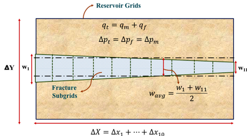
Figure 6. Averaging Mobility of Reservoir Grids.
