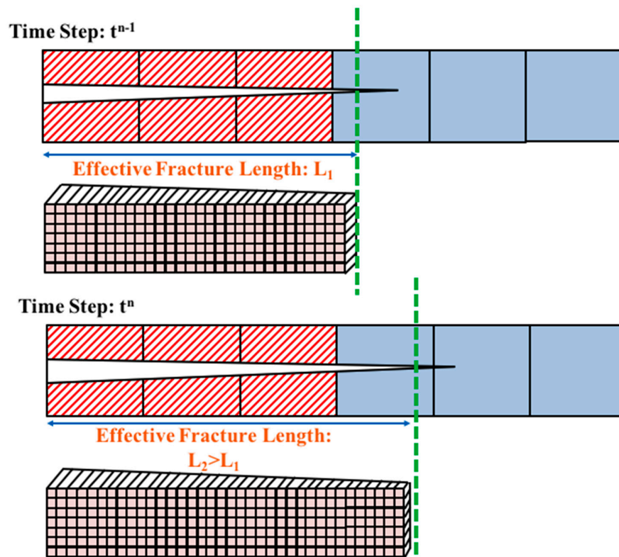
Figure 3. Fracture Propagation and Adaptive Re-meshing.
