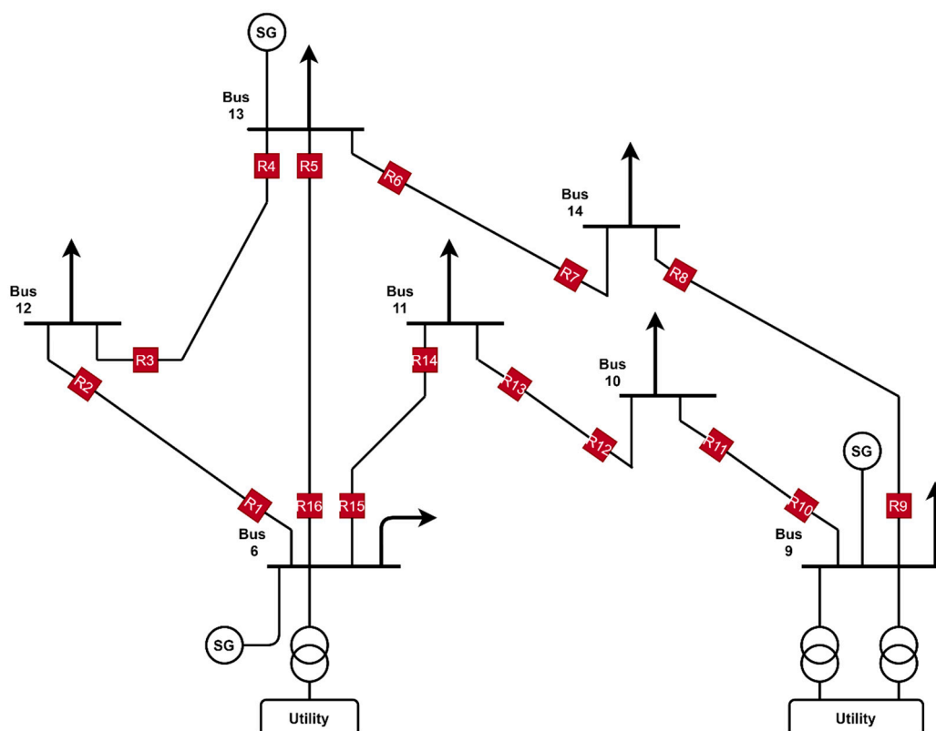
Figure 2. Schematic view of modified 14 bus microgrid.
