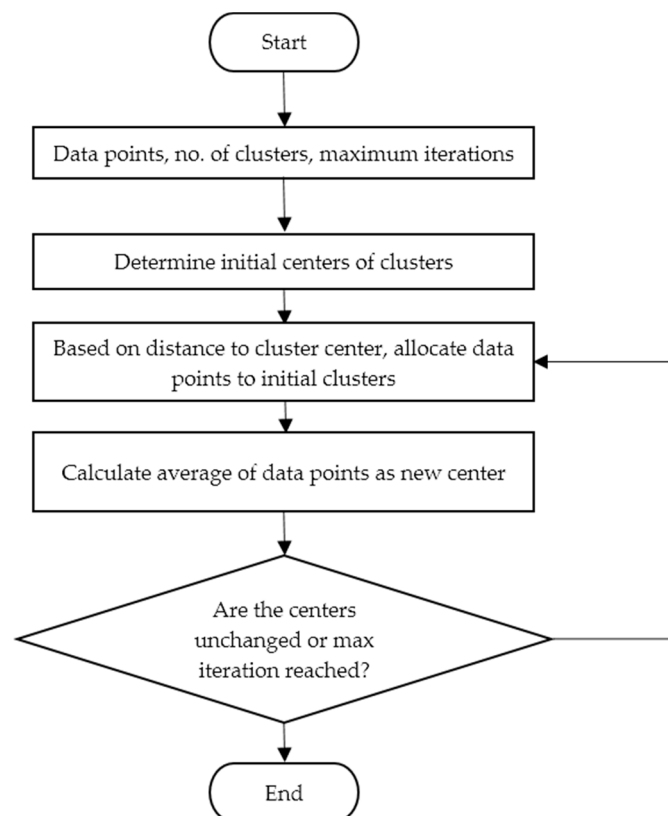
Figure 1. Flowchart of the k-means clustering algorithm.
