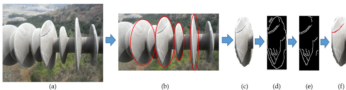
Figure 12. The process of splits detection in polymer insulator. (a) The input image, (b) ellipse detection result, (c) one of the segmented cap, (d) edge map, (e) edge map after boundary removal, and (f) splits detection result.
