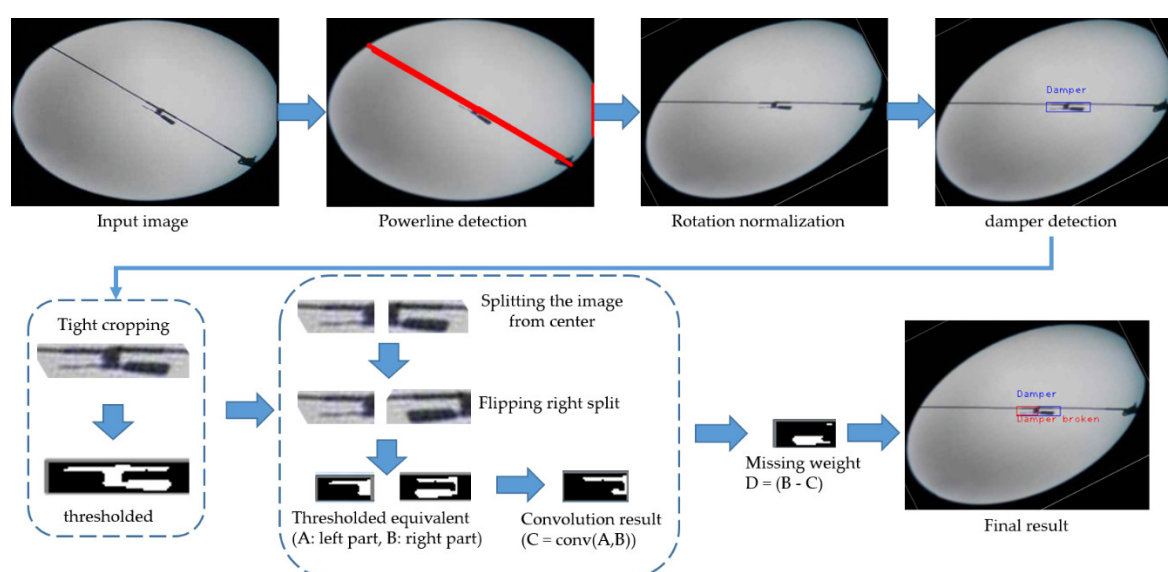
Figure 10. Schematic of the broken vibration damper detection algorithm.
