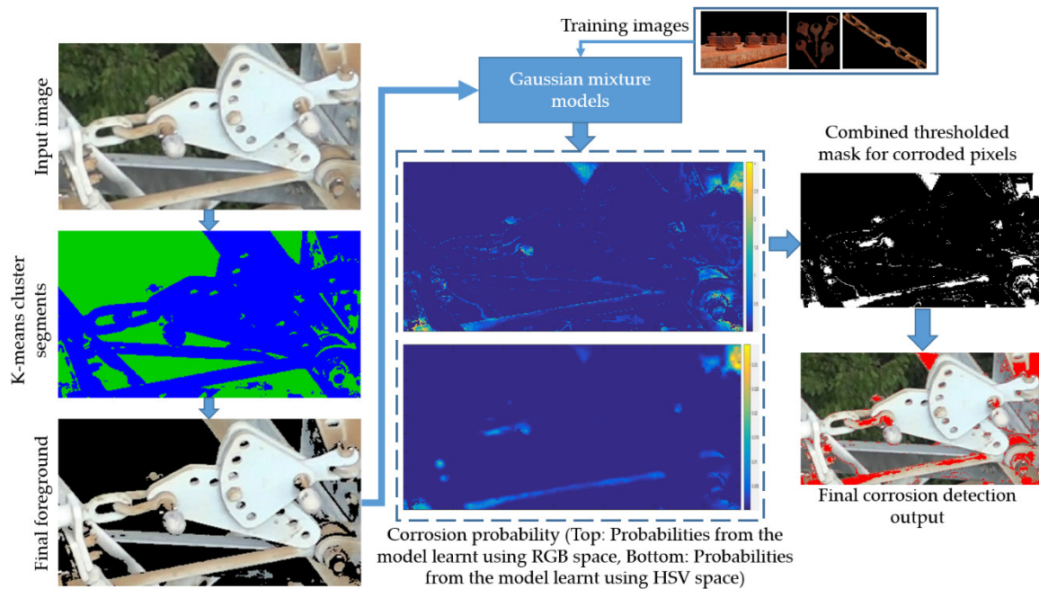
Figure 8. Schematic of the corrosion detection algorithm.
