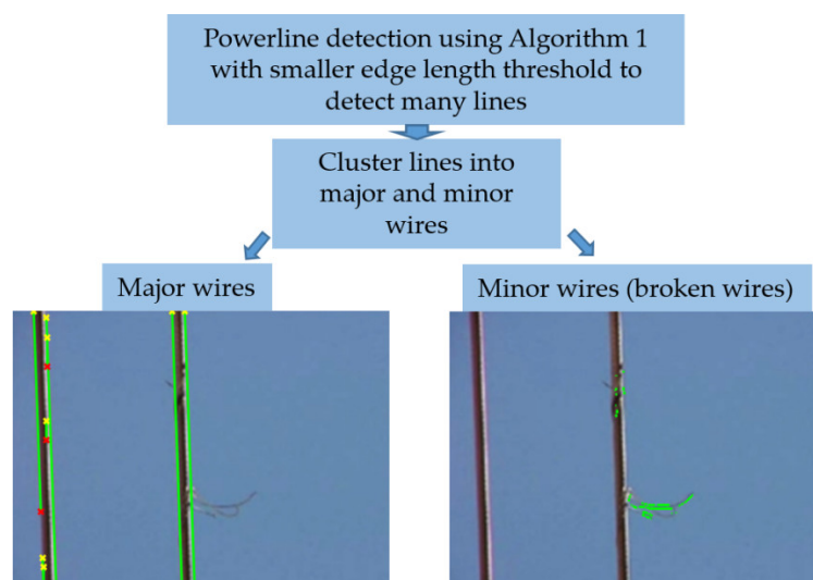
Figure 9. Schematic of the broken power line detection algorithm.
