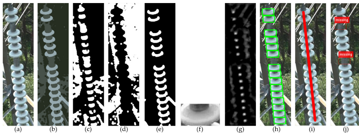
Figure 6. Steps of the broken shed detection. (a) Detected insulator image from CNN-based detector, (b) output of color clustering based segmentation, (c–e) segmentation masks of the three clusters, (f) candidate template after connected component analysis and max voting for finding most repeating pattern, (g) activation map of the template matching, (h) results of template matching, (i) fitting the centers of the template matching result to a straight line, and (j) final detected defect.
