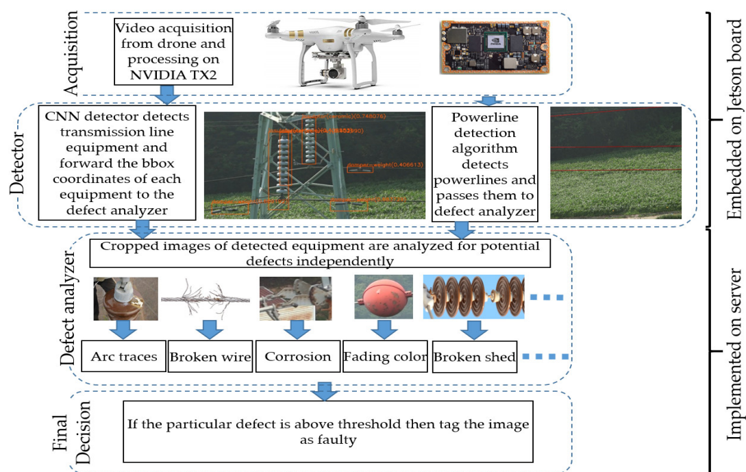
Figure 2. Overall system diagram.
