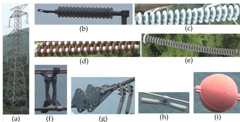
Figure 1. Example images of various types of transmission line components that can be detected by our proposed system. (a) Transmission tower; (b) lightning-arrester (LA); (c) suspension type white porcelain insulator; (d) suspension type red porcelain insulator; (e) polymer insulator; (f) spacer; (g) sag adjuster with bolted tension clamp; (h) vibration damper; and (i) balisor.
