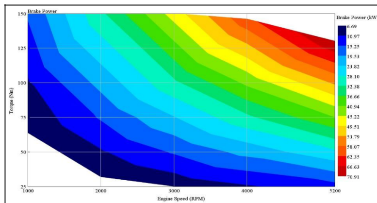
Figure 4. Brake power of engine model.
