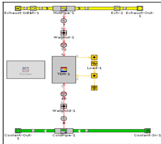
Figure 5. 1 Module of the thermoelectric generator (TEG).
