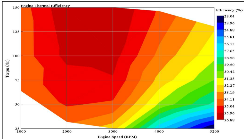
Figure 8. Engine thermal efficiency.
