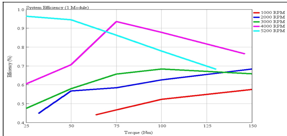
Figure 15. System efficiency of 1 module (25 mm × 25 mm).
