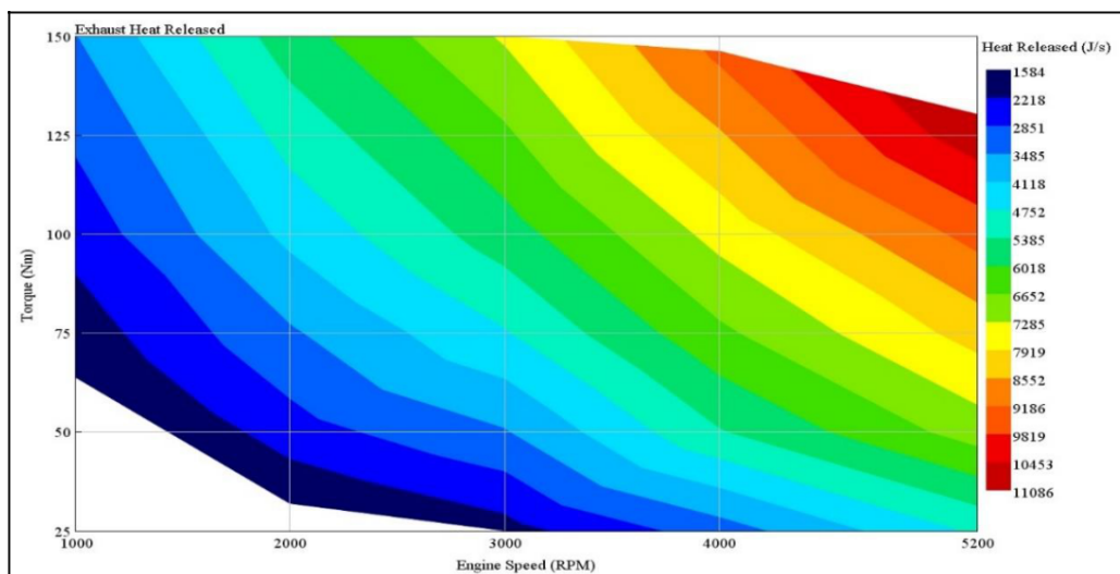
Figure 12. Exhaust heat released.
