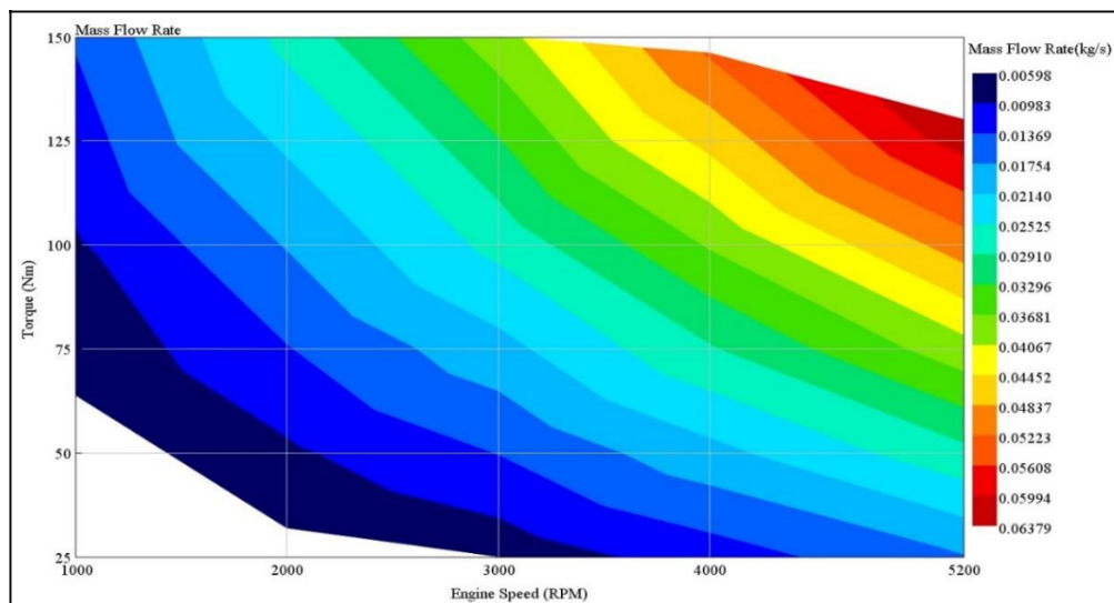
Figure 10. Exhaust mass flow rate.
