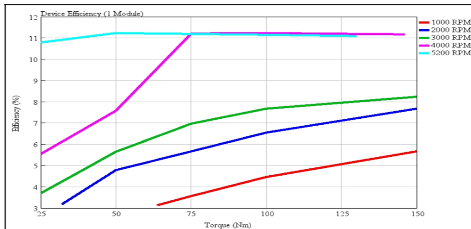
Figure 14. Device efficiency of 1 module (25 mm × 25 mm).
