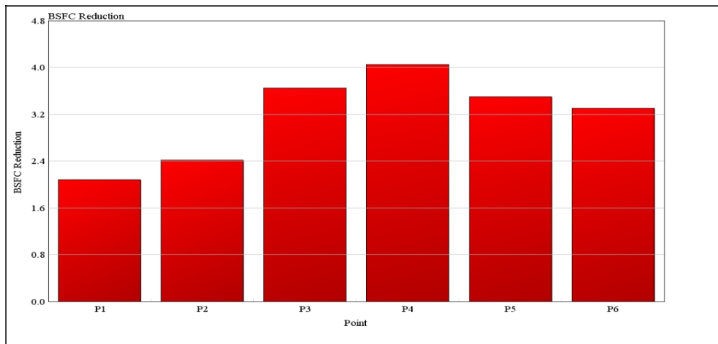
Figure 26. BSFC reduction.
