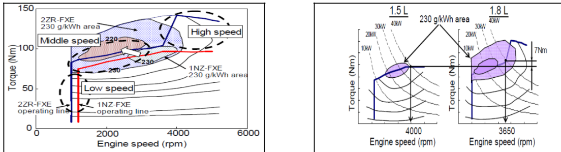
Figure 2. Theoretical BSFC map of 2 ZR-FXE Engine (left) and theoretical engine power of 2 ZR-FXE Engine (right).
