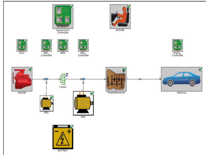
Figure 7. Series-parallel hybrid electric vehicle (HEV) model.
