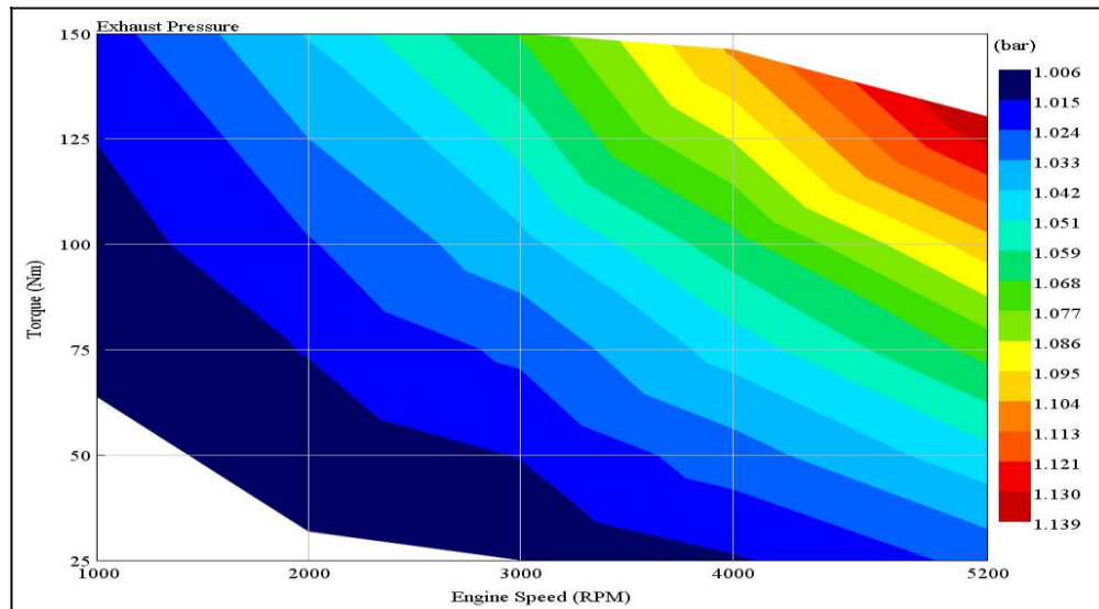
Figure 9. Exhaust pressure.
