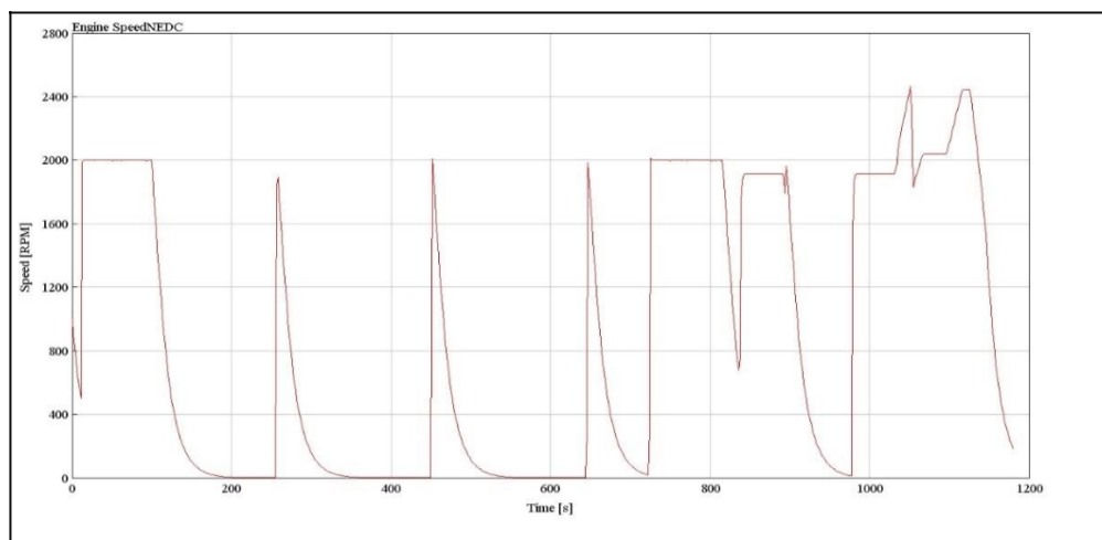
Figure 29. Engine speed (NEDC).
