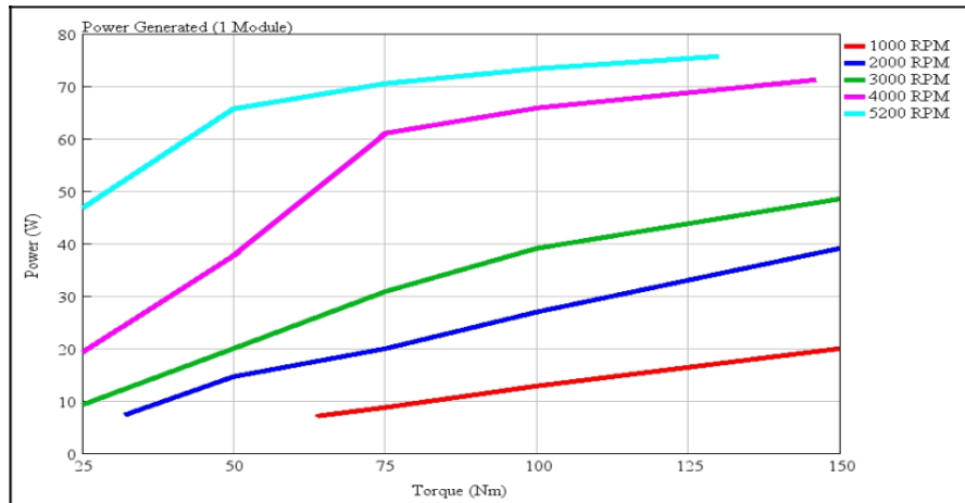
Figure 13. Power generated by 1 module (25 mm × 25 mm).
