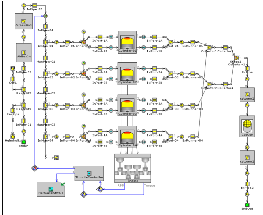
Figure 1. 4-Cylinder Engine.
