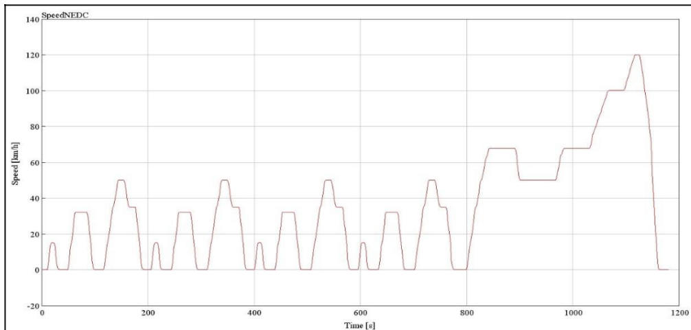
Figure 28. Driving cycle (New European Driving Cycle (NEDC)).
