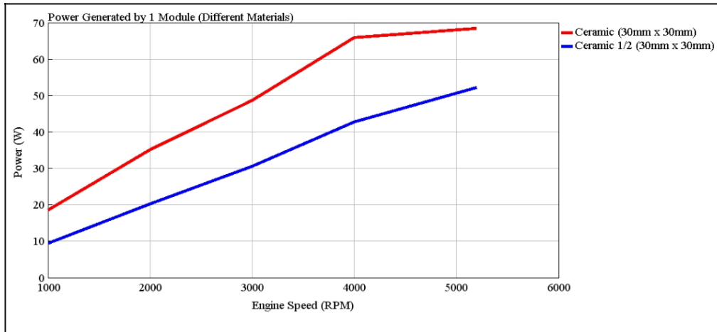
Figure 19. Power generated by different materials (1 module).
