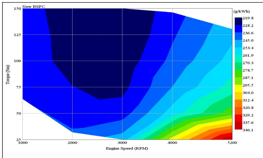
Figure 27. New BSFC.
