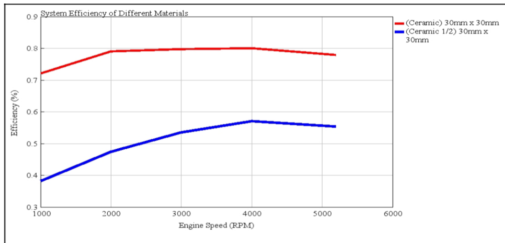
Figure 20. System efficiency of different materials (1 module).
