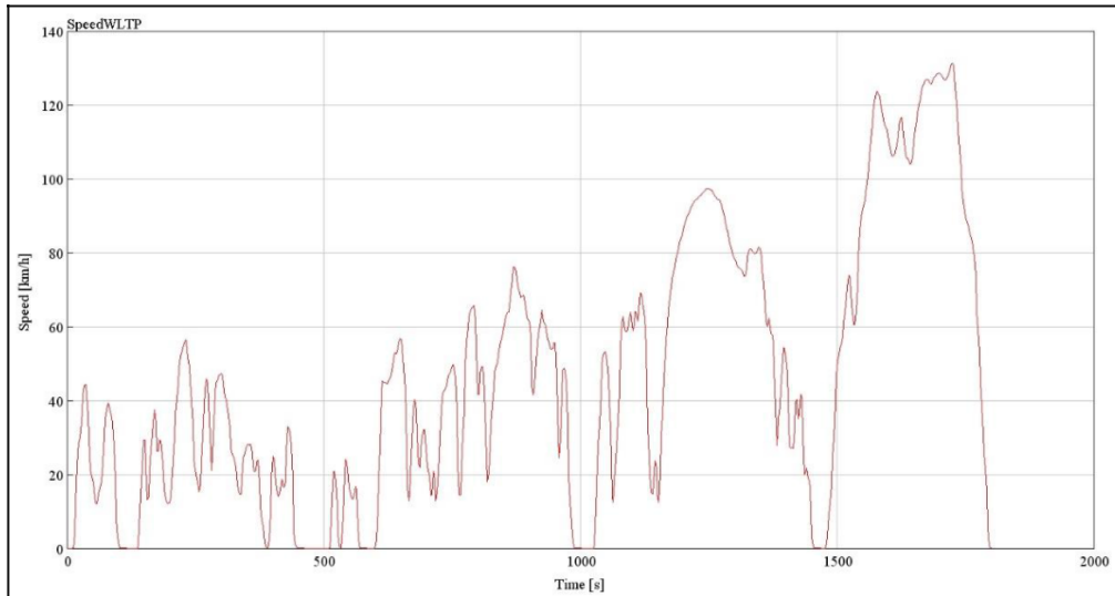
Figure 30. Drive cycle (Worldwide Harmonised Light Vehicle Test Procedure (WLTP)).
