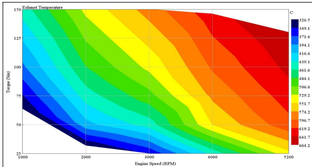
Figure 11. Exhaust temperature.
