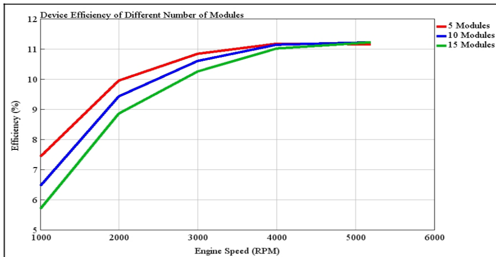
Figure 22. Device efficiency of different number of modules.
