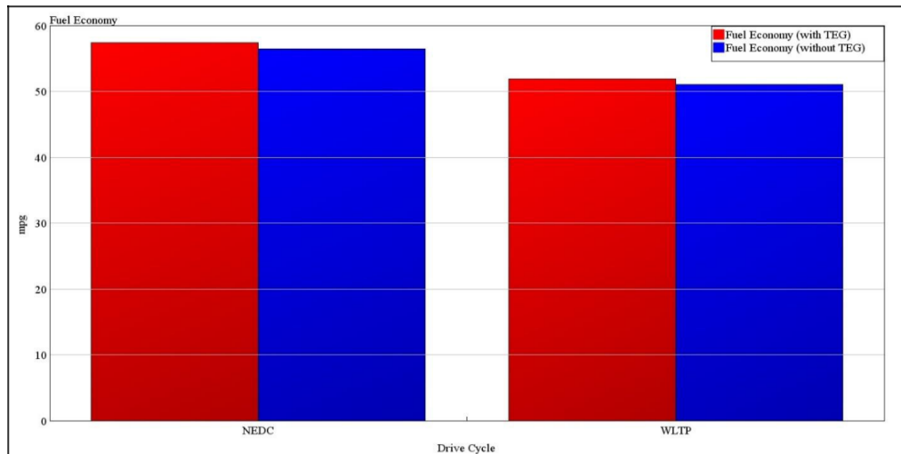
Figure 32. Fuel economy.
