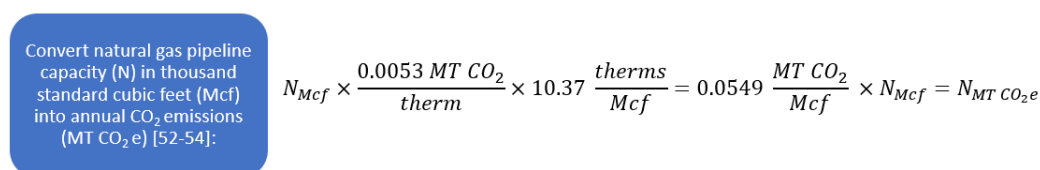
Figure 3. Equation used to calculate potential annual CO 2 emissions (MT CO 2 e) of a natural gas facility.
