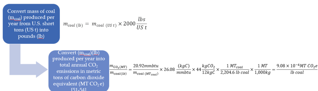
Figure 1. Stepwise process used to calculate potential annual CO 2 emissions (MT CO 2 e) of a coal facility.
