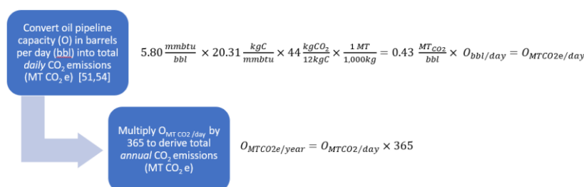
Figure 2. Stepwise process used to calculate potential annual CO 2 emissions (MT CO 2 e) of an oil facility.
