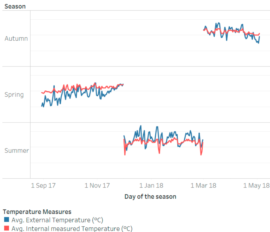
Figure 4. Weather seasons mapped with average external temperature and internal measured temperature in the greenhouse.
