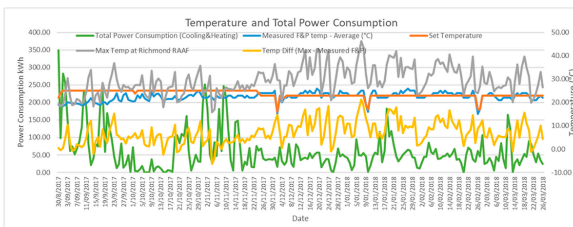
Figure 3. Temperature and power consumption over the full capsicum crop lifecycle.
