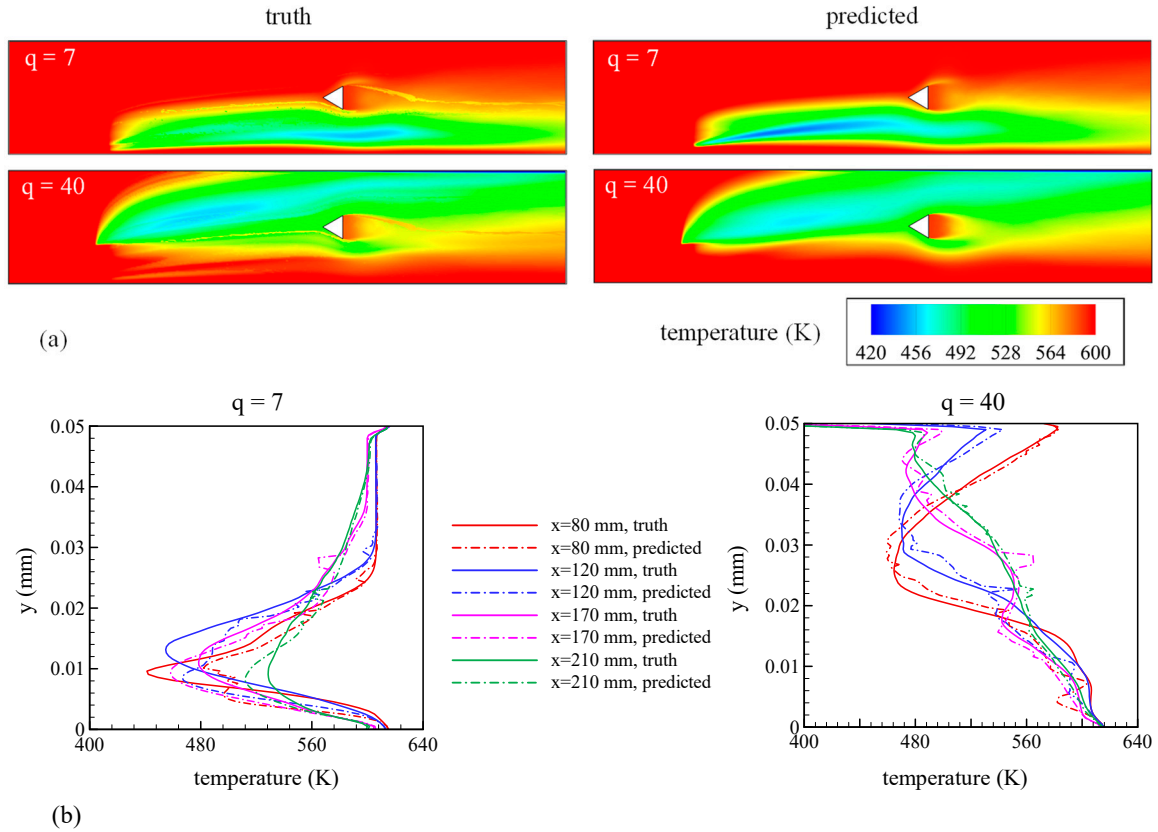
Figure 14. Comparison between predictions from the GPML algorithm (referred to as predictions) with LES results (referred to as truth) for test points of q = 7 and 40. (a) Contours of temperature in the mid-plane of the flow domain; (b) variation of temperature along the y -axis at x = 80, 120, 170 , and 210 mm.
