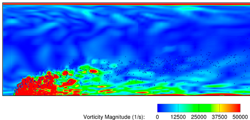
Figure 7. Instantaneous vorticity contour showing the turbulent wake formation downstream of the liquid jet.
