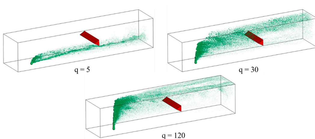
Figure 10. Instantaneous spray field for three representative cases of momentum flux ratios of 5 , 30 , 120 showing qualitative differences in the spray field.
