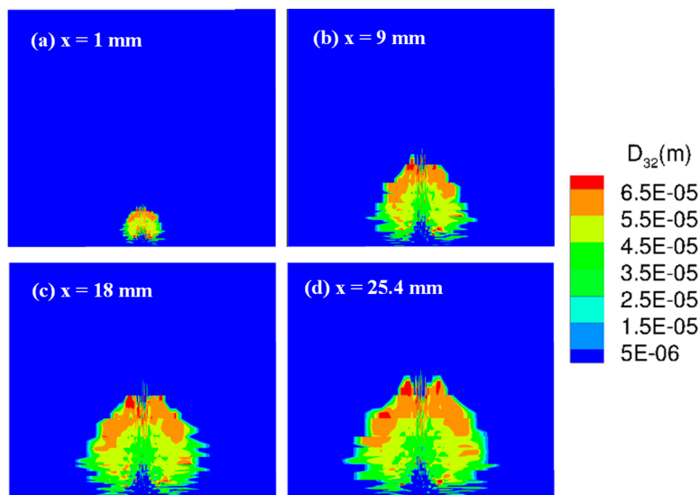
Figure 5. Sauter mean diameter (SMD) distribution on the y–z plane: progressive streamwise locations showing the development of the spray field at T_a = 300\text{ K} at (a) 1 mm, (b) 9 mm, (c) 18 mm, and (d) 25.4 mm downstream of the injection location.
