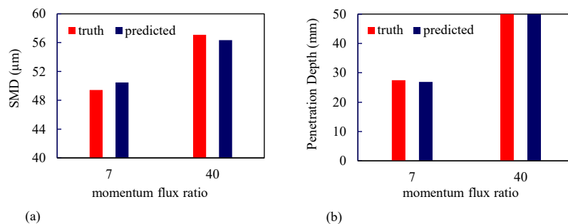
Figure 16. Comparison between predictions from the GPML algorithm (referred to as predictions) with LES results (referred to as truth) for test points of q = 7 and 40. (a) SMD; (b) liquid jet penetration depth.
