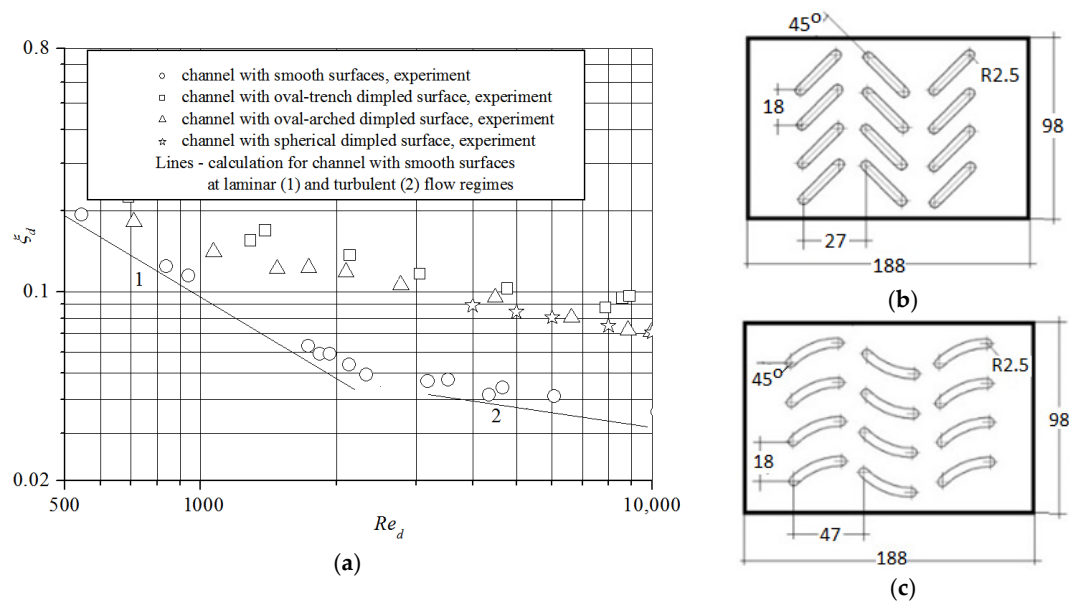
Figure 11. Friction factor coefficients versus Reynolds number values (a) for the surface with the multi-row arrangement of oval-trench (b) and oval-arched (c) dimpled surfaces. Sizes are in mm.
