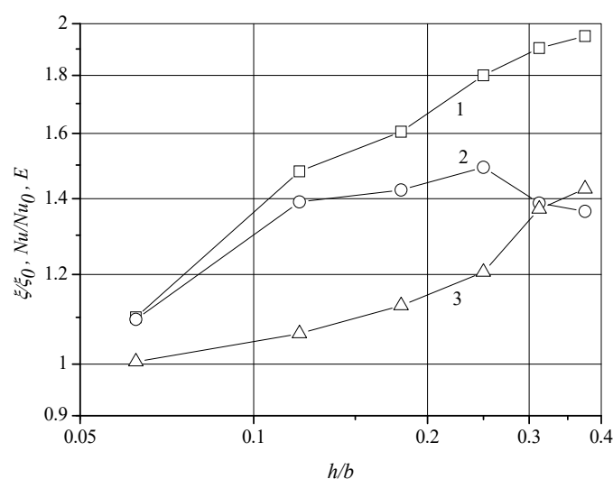
Figure 4. Relative heat transfer Nu/Nu_0 (1), friction factor \xi/\xi_0 (3) ratio, and thermal-hydraulic efficiency E = (Nu/Nu_0)/(\xi/\xi_0) (2) versus the relative depth of the dimple h/b .
