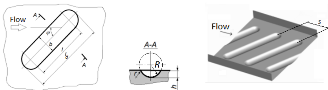
Figure 1. Characteristic scheme of the oval-trench-shaped dimple: l —a length of the dimple trench part, m; l_d —a total length, m; h —a depth, m; b —a width, m; r —edge rounding radius, m; \varphi —the angle of attack of the dimple (to the main flow), deg; S —a notching step; R —an embedding sphere radius, m; A-A—CROSS-SECTION.
