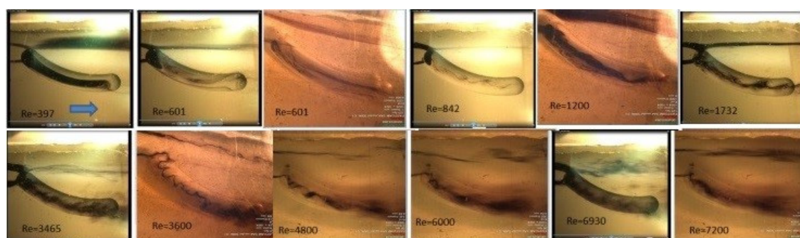
Figure 10. Visualization of flow over the oval-arched dimple for h/b = 0.5 , l_d/b = 7 for the various Reynolds number values.
