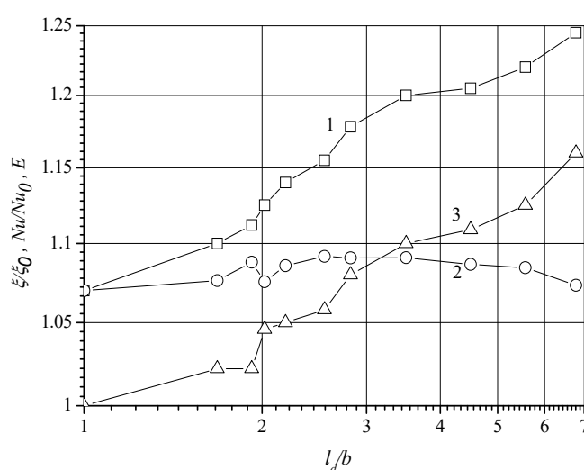
Figure 2. Relative heat transfer Nu/Nu_0 (designation 1), friction factor \xi/\xi_0 (designation 2) ratio, and thermal-hydraulic efficiency E = (Nu/Nu_0)/(\xi/\xi_0) (3) along the length of the domain with the oval-trench dimple.
