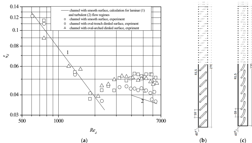
Figure 12. Friction factor coefficients versus Reynolds number values (a) for the surface with the single-row arrangement of oval-trench (b) and oval-arched (c) dimpled surfaces. Size are in mm.
