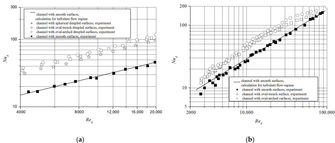
Figure 13. Heat transfer coefficient values for the surfaces with a multi-row (a) and single row (b) dimple arrangement of the oval-trench and oval-arched dimples.
