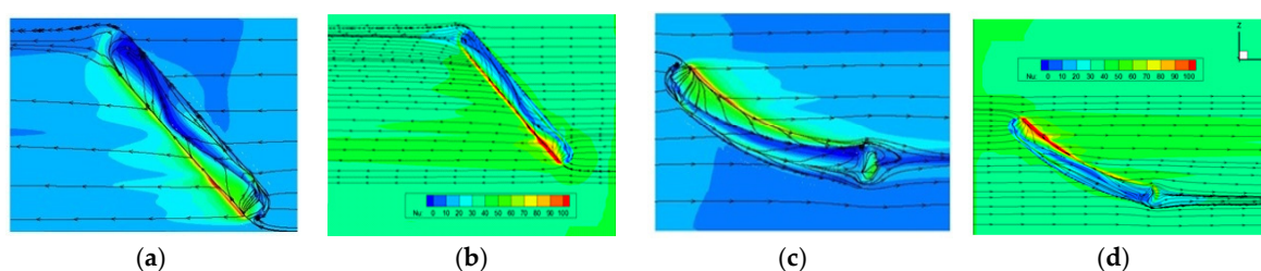
Figure 6. Streamlines for the flow over the oval-trench (a) and oval-arched (c) dimples and local heat transfer coefficients values (b) and (d), respectively.
