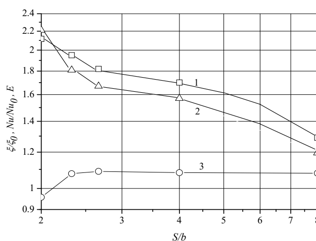
Figure 5. Relative heat transfer Nu/Nu_0 (1), friction factor \xi/\xi_0 (2) ratio, and thermal-hydraulic efficiency E = (Nu/Nu_0)/(\xi/\xi_0) (3) versus the relative notching step S/h .
