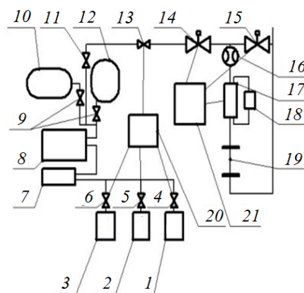
Figure 8. Scheme of the experimental stand: 1, 2, 3—compressors (capacity 2400 L/min, 1400 L/min, 880 L/min); 4, 5, 6, 13—solenoid valve two-position pilot action; 7—filtration module for cleaning compressed air; 8—dehumidifier; 9, 11—valves; 10, 12—receivers; 14—electrically operated ball valve; 15—electrically operated ball valve for bypass; 16—ultrasonic flowmeter—gas meter; 17—heater; 18—energy source for heater; 19—working area; 20—controller; 21—valve control panel 4, 5, 6, 13.
