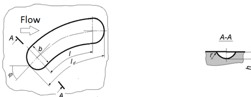
Figure 7. Characteristic scheme of the oval-arched shaped dimple: l —a length of the trench part, mm; l_d —a total length, mm; h —a depth, mm; b —a width, mm; r —edge rounding radius, mm; \varphi —the angle of attack (to the main flow), deg. of the dimple and S —a notching step; A-A—cross-section.
