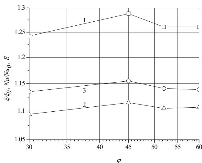
Figure 3. Relative heat transfer Nu/Nu_0 (1), friction factor \xi/\xi_0 (2) ratio, and thermal-hydraulic efficiency E = (Nu/Nu_0)/(\xi/\xi_0) (3) versus the angle of attack \varphi for the l_d/b = 6 .
