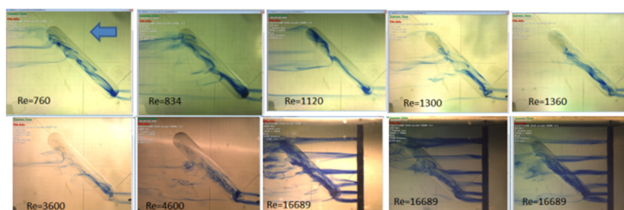
Figure 9. Visualization of flow over the oval-trench dimple for h/b = 0.5 , l_d/b = 7 for the various Reynolds number values.
