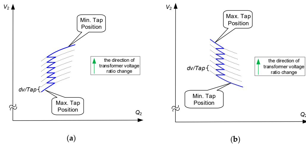
Figure 6. Influence of transformer tap position changes on the V-Q characteristics: (a) the situation corresponds to work in point “b” shown in Figure 3a; (b) the situation corresponds to work in point “a” shown in Figure 3a.
