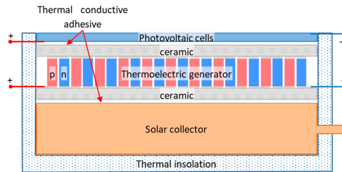
Figure 3. PV-TEG-T structure.
