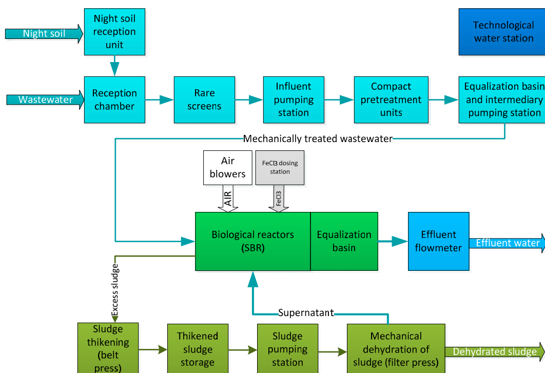
Figure 2. Process flow diagram for WWTP.
