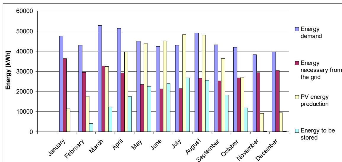
Figure 7. Monthly energy demand, energy production by PV system, energy necessary from the grid, and energy necessary to be stored in batteries.
