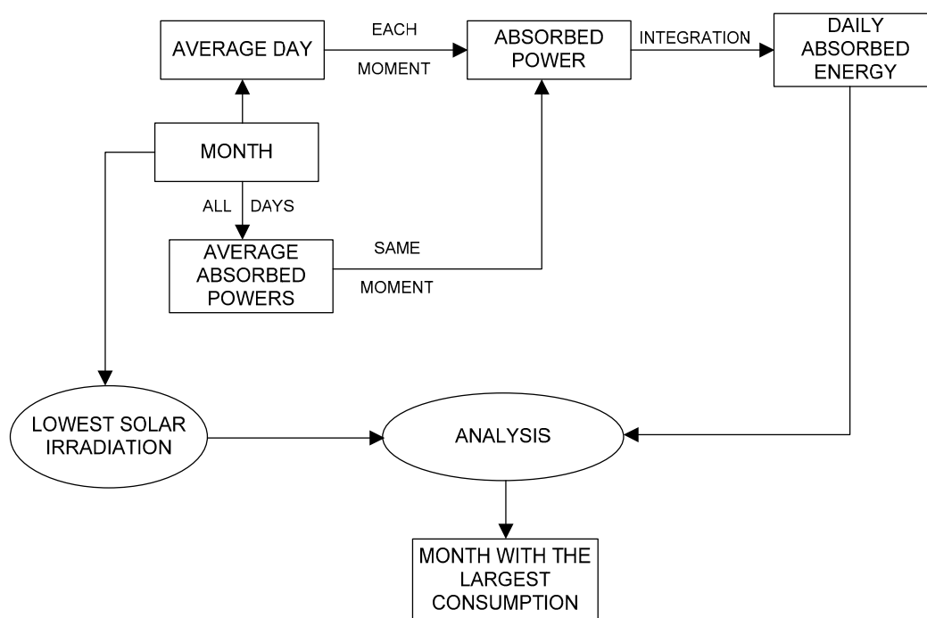
Figure 3. Flowchart of average day for consumed active power.
