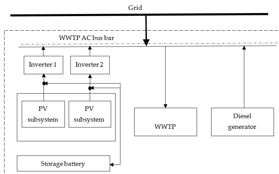
Figure 5. Schematic of a hybrid system.
