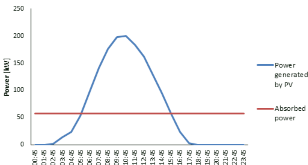
Figure 6. Hourly average power of WWTP for a typical day in July.
