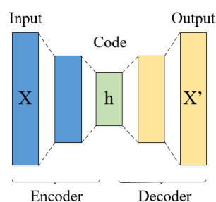
Figure 1. Example structure for an under-complete autoencoder.
