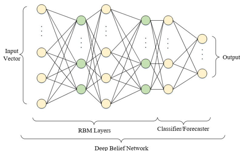
Figure 5. Example of a structure for a deep belief network.
