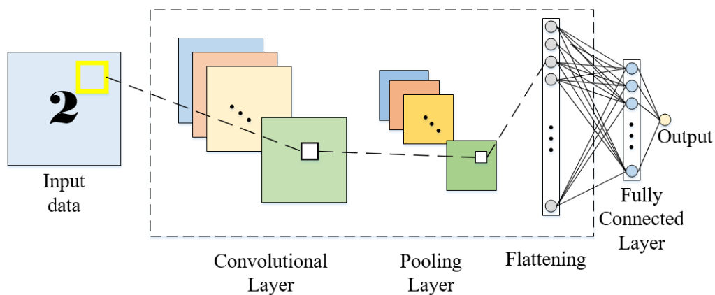
Figure 3. Example structure for a convolutional neural network.
