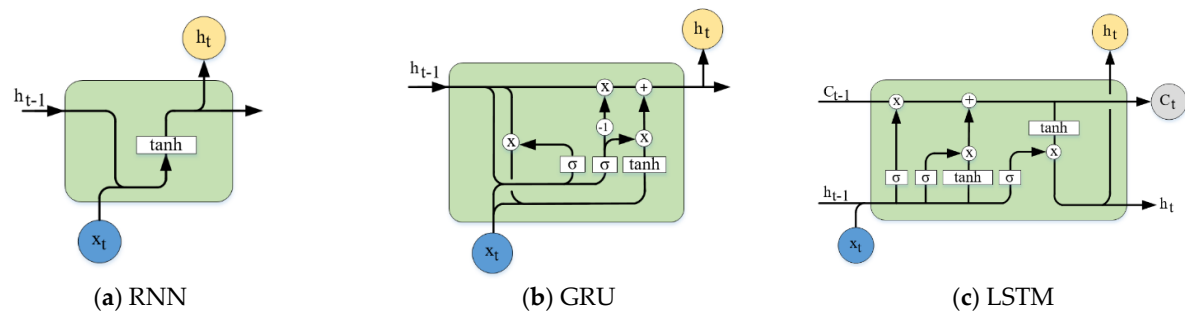
Figure 2. Recurrent neural network types.
