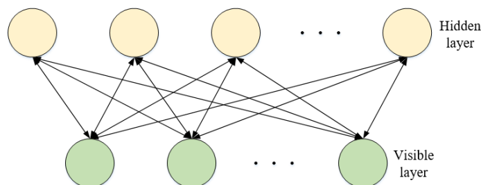
Figure 4. Example structure of a restricted Boltzmann machine.
