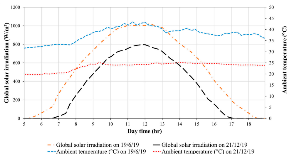
Figure 6. Actual global solar irradiation and the ambient temperature during the longest day (19 June 2019) and the shortest day (21 December 2019) in Muscat.
