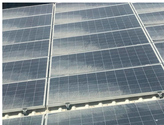
Figure 9. Photograph of partial section of the modules showing the high dust accumulation.
