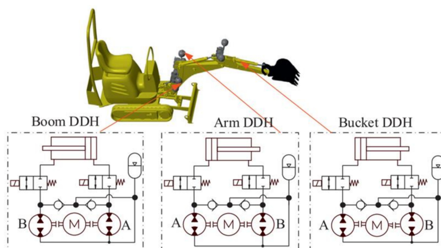
Figure 14. Direct-driven hydraulic scheme for a compact excavator. [97].
