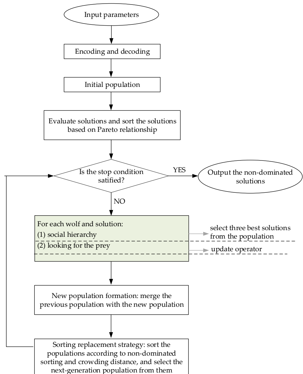
Figure 3. Multi-objective gray wolf algorithm flow chart.
