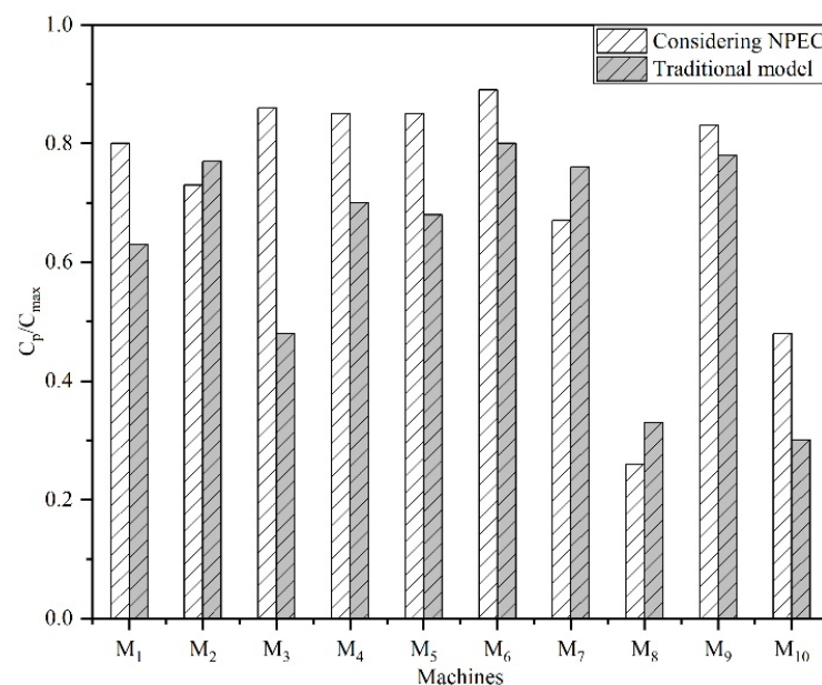
Figure 13. Comparison in C_p/C for machines.
