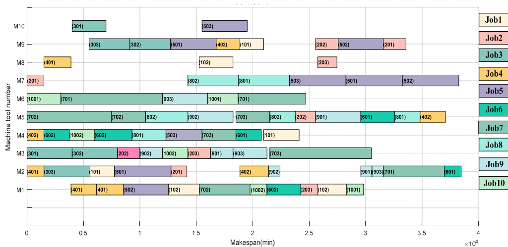
Figure 9. Gantt chart of the optimized schedule scheme.
