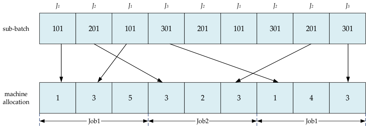
Figure 4. Chromosome coding, for example.
