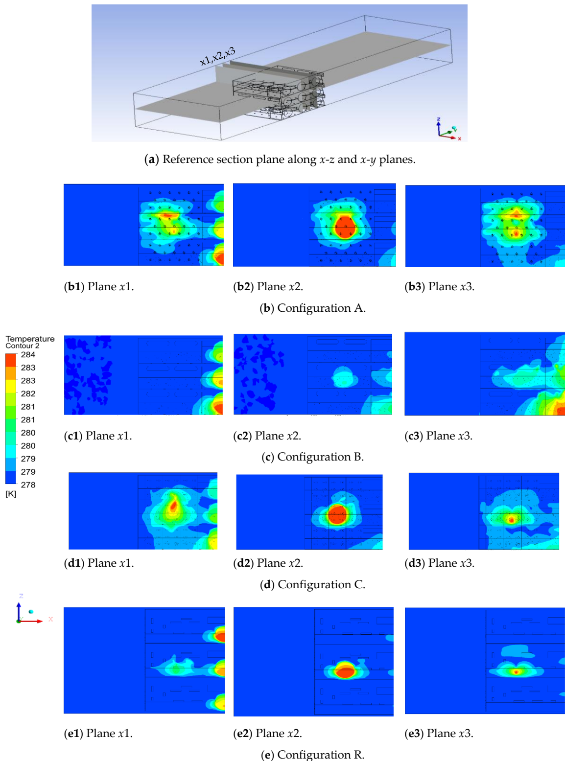
Figure 5. Temperature distribution after 8 h of simulation with section planes along x - z axis.
