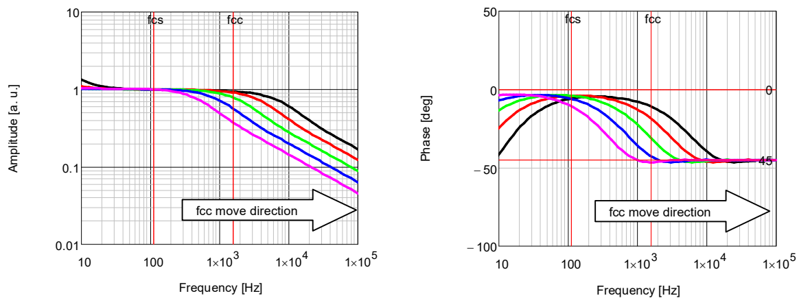
Figure 4. Theoretical PTR amplitude and phase characteristics calculated for different values of thermal parameters. Solid green line ( \alpha_c , \lambda_c ), solid red line ( 2\alpha_c , 2\lambda_c ), solid black line ( 4\alpha_c , 4\lambda_c ), solid blue line ( \alpha_c/2 , \lambda_c/2 ) and solid pink line ( \alpha_c/4 , \lambda_c/4 ).
