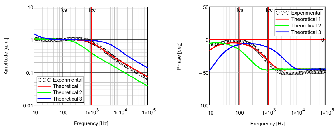
Figure 11. Theoretical and experimental PTR amplitude and phase characteristics obtained for the TMZ-I + \text{Ce}(\text{NO}_3)_3 sample.
