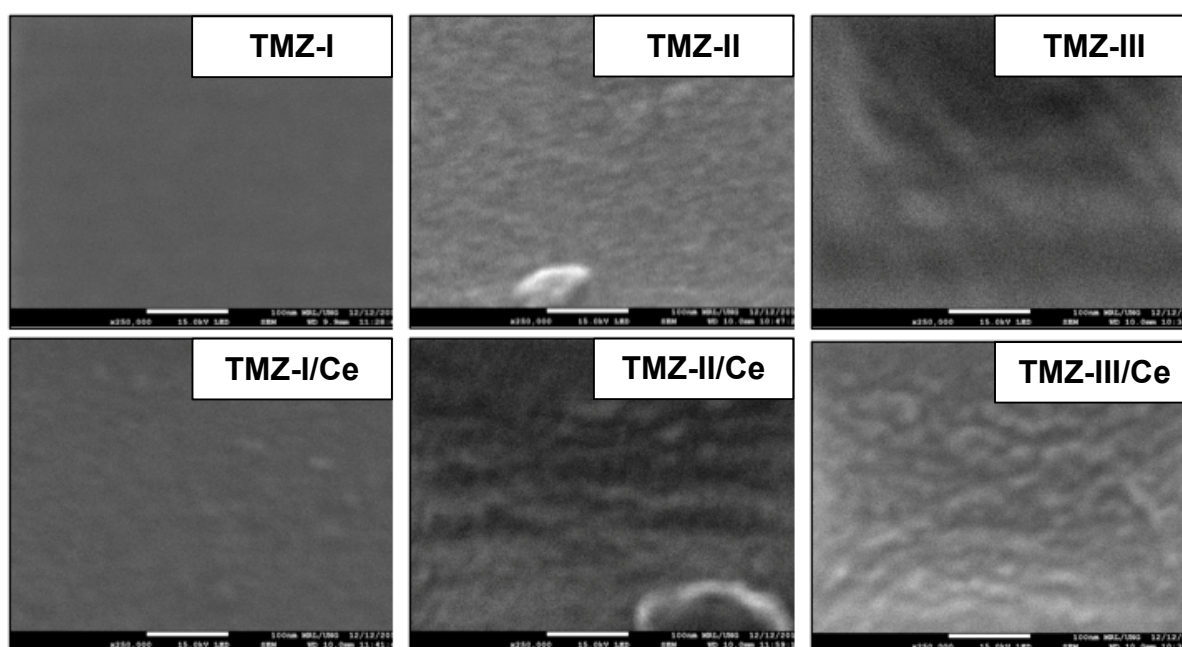
Figure 9. The SEM images (250,000×) of the TMZ coatings.
