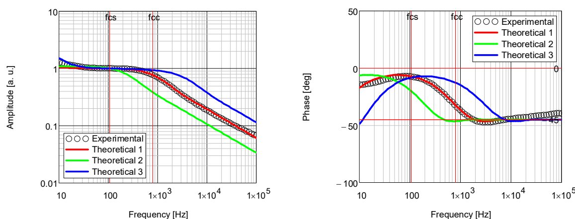
Figure 10. Theoretical and experimental PTR amplitude and phase characteristics obtained for the TMZ-I sample.
