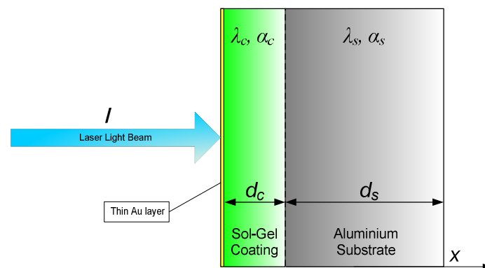
Figure 3. Simplified schematic of the investigated sample.
