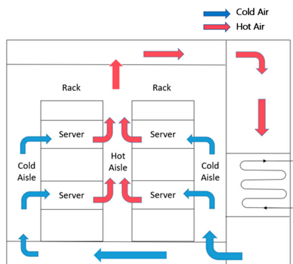
Figure 3. Direct air-side economizers.
