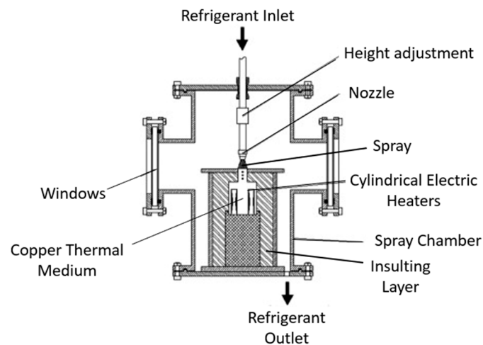
Figure 15. Schematic of closed loop spray cooling system [87].
