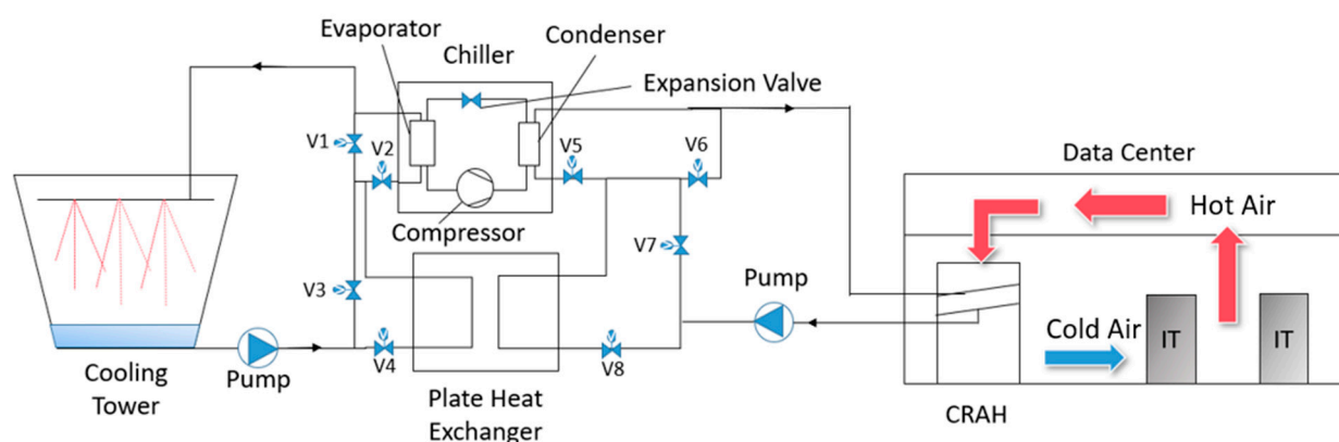
Figure 8. Plate heat exchangers in series with chillers.
