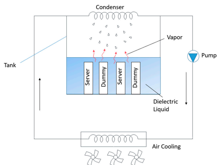
Figure 14. The schematic diagram of two-phase [68].
