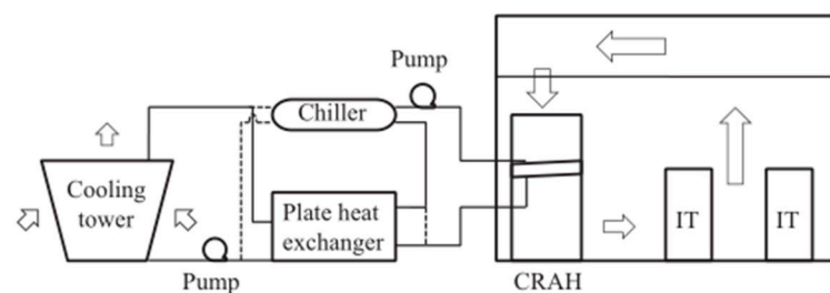
Figure 7. Cooling tower system [32].
