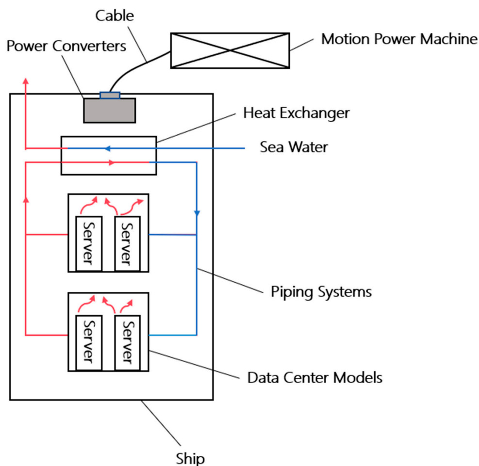
Figure 5. Seawater cooling system [39].
