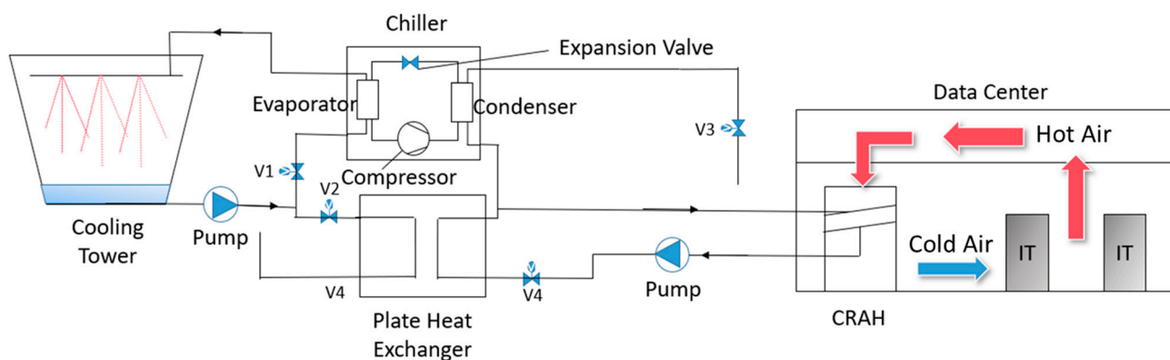
Figure 9. Plate heat exchangers in parallel with chillers.
