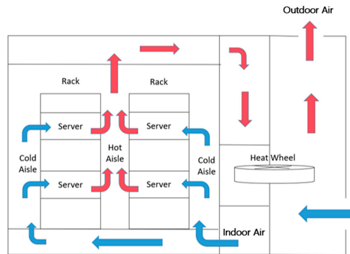
Figure 4. Wheel indirect air cooling system [32].
