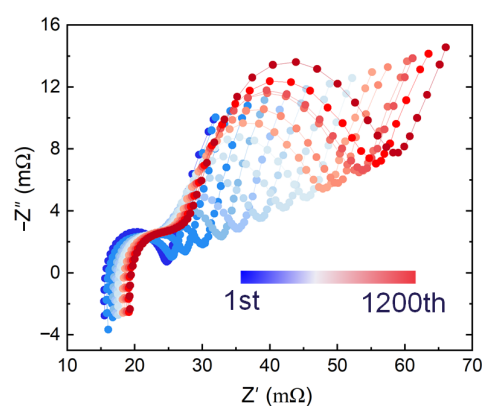
Figure 9. Evolution of the Nyquist plot (obtained through EIS measurements) due to aging from BOL to 1200 EFCs of an NMC-based Li-ion battery. Aging: WLTC discharging to 75% DOD and full re-charging with 0.5 C-rate at 45 °C. EIS measurement: 6.5 kHz–10 mHz frequency range, 50% SOC, and 25 °C.
