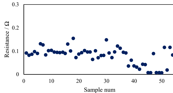
Figure 7. Resistance values of 54 s-life batteries [32].
