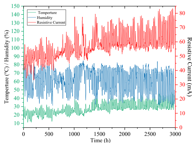
Figure 1. Original data in respect of MOA resistive current, environmental temperature, and humidity.
