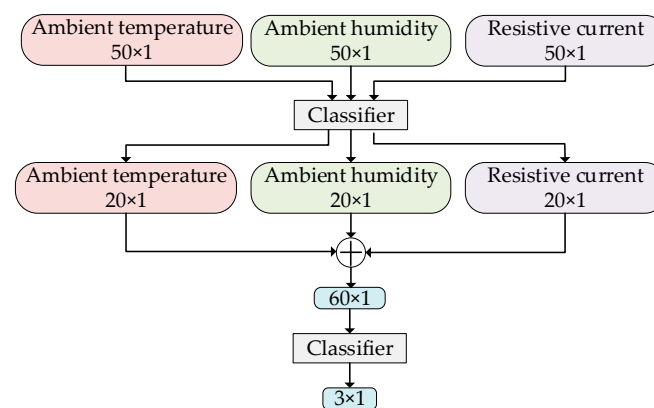
Figure 4. Feature fusion network framework.
