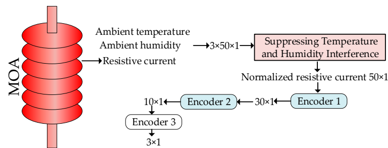
Figure 2. Framework diagram of the MOA fault identification method combining temperature and humidity interference suppression with SAE.
