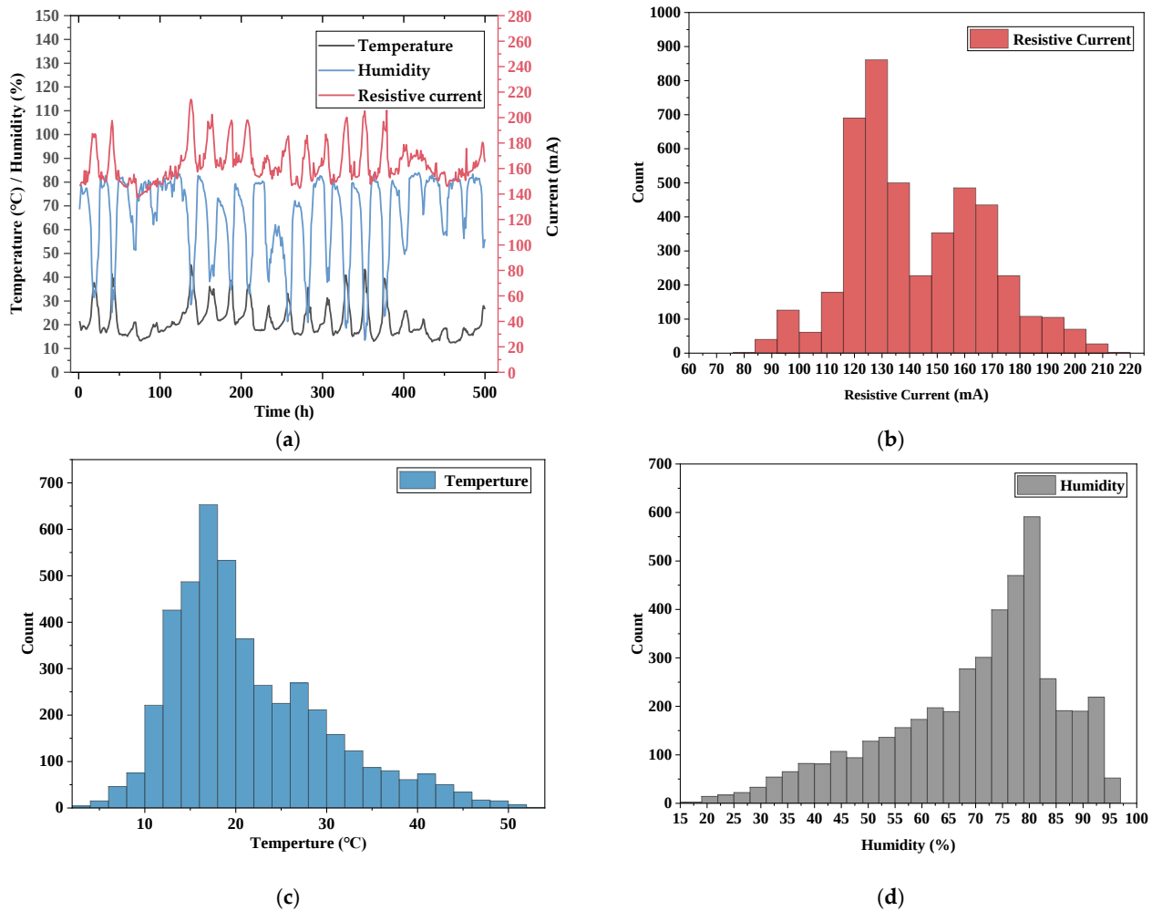
Figure 6. Original data and histograms of the frequency distribution under MOA fault condition. (a) Original data in respect of resistive current and environmental temperature and humidity; (b) histogram of the frequency distribution of the MOA resistive current; (c) histogram of the frequency distribution of environmental temperature; (d) histogram of the frequency distribution of environmental humidity under normal conditions.
