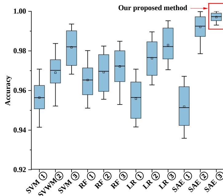
Figure 11. Accuracy distribution under 50 trials for different classification algorithms.
