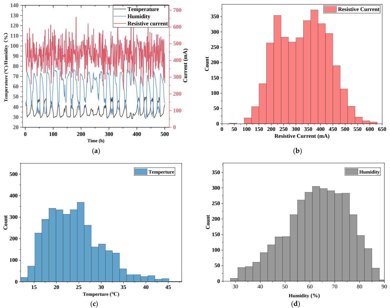
Figure 7. Original data and histograms in respect of the frequency distribution under MOA monitoring device failure conditions. (a) Original data regarding resistive current and environmental temperature and humidity; (b) histogram of the frequency distribution of the MOA resistive current; (c) histogram of the frequency distribution of environmental temperature; (d) histogram of the frequency distribution of environmental humidity under normal conditions.
