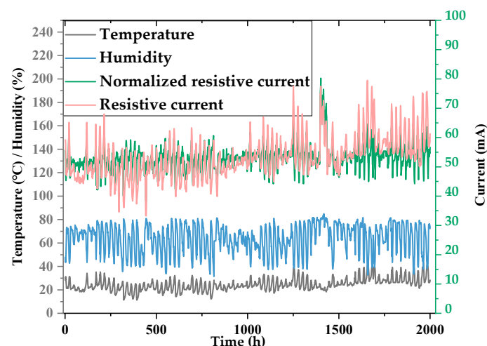
Figure 8. Fluctuation diagram of MOA resistance current and environmental temperature and humidity monitoring data before and after suppression of the temperature and humidity interference.
