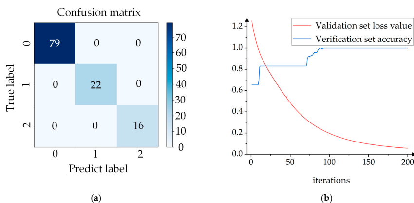
Figure 9. (a) Confusion matrix of the MOA classification algorithm combining suppression of environmental temperature and humidity interference with SAE; (b) accuracy and loss values of the validation set.
