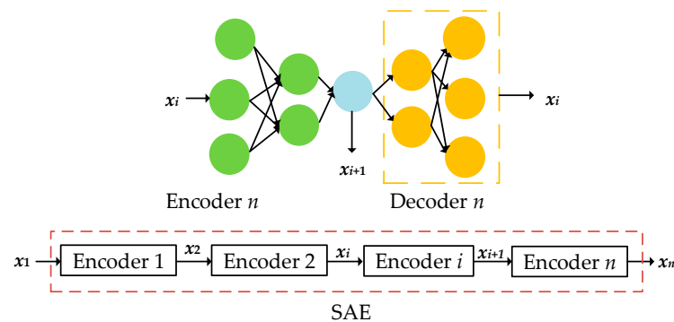
Figure 3. Stacked self-encoding structure.
