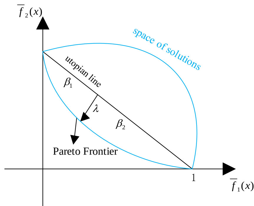
Figure 3. Schematic diagram of NBI algorithm after normalization.
