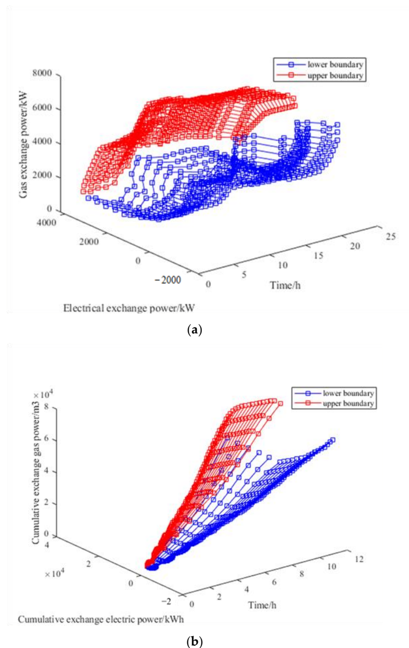
Figure 7. Three-dimensional adjustable capacity in scenario I. (a) coupling relation of exchanged electric and gas power; (b) coupling relation of accumulated exchanged electric and gas power.
