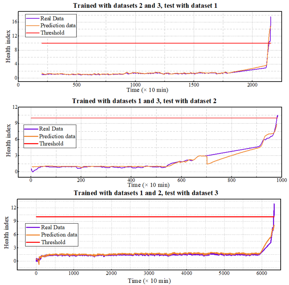
Figure 10. RUL prediction results of similarity models.
