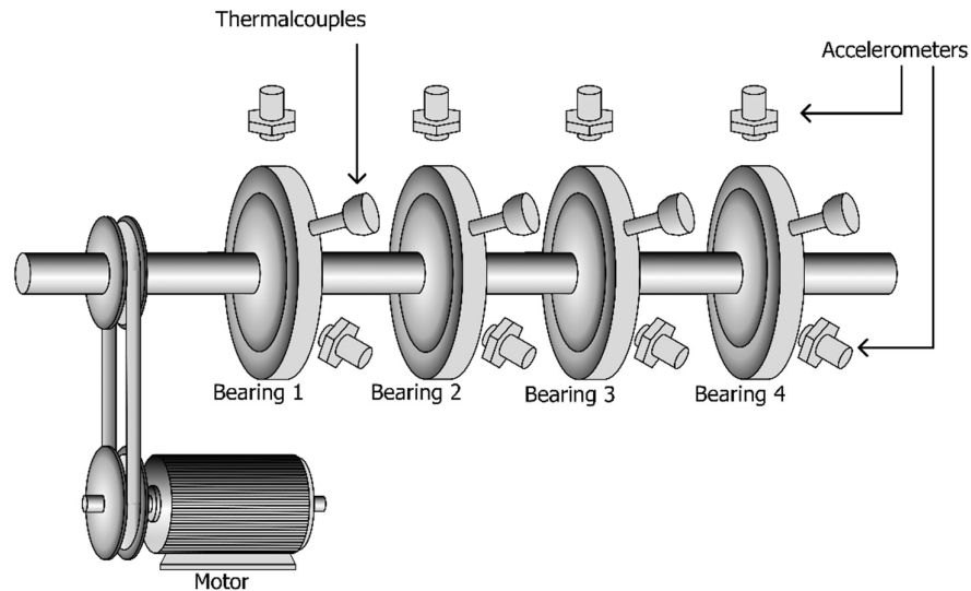
Figure 1. Bearing test rig.
