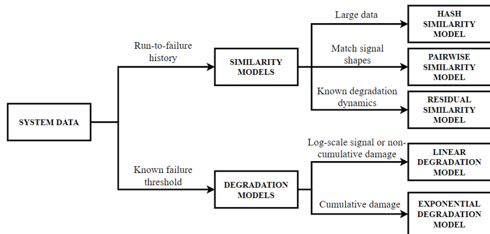
Figure 8. Approach to predicting RUL of main bearing.
