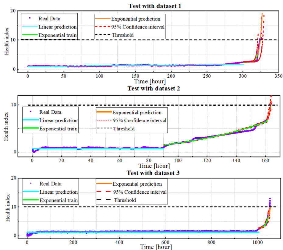
Figure 11. RUL prediction results of degradation models.
