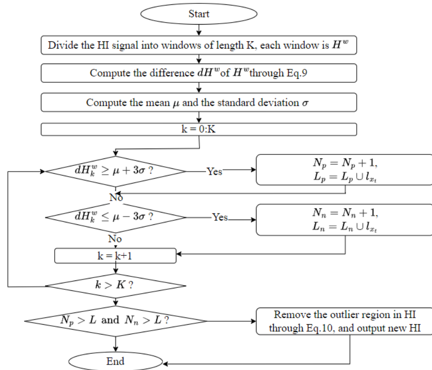
Figure 6. Flowchart for the algorithm to eliminate outliers in the HI.
