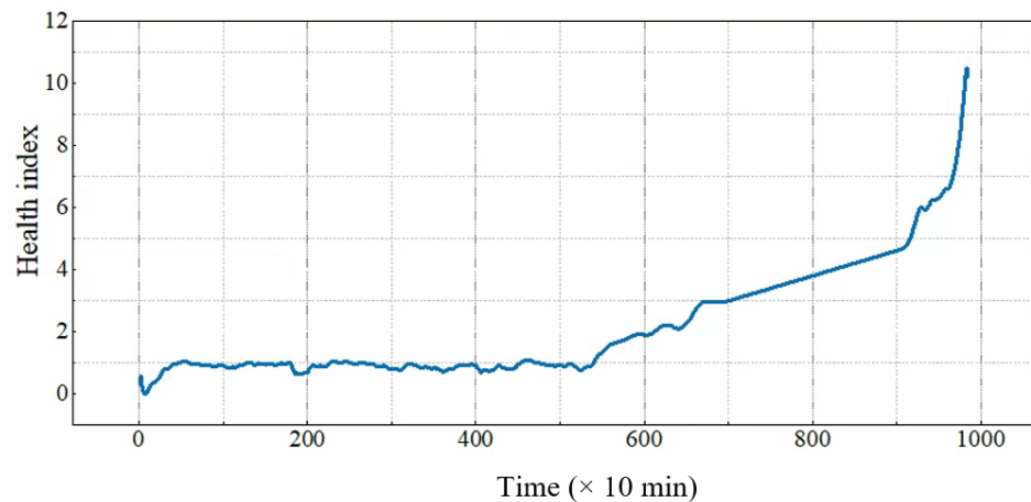
Figure 7. The HI value has been eliminated from the outlier.
