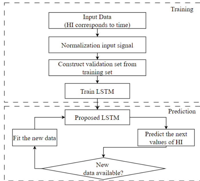
Figure 9. The process of diagnosing the RUL of the device is based on the similarity model.
