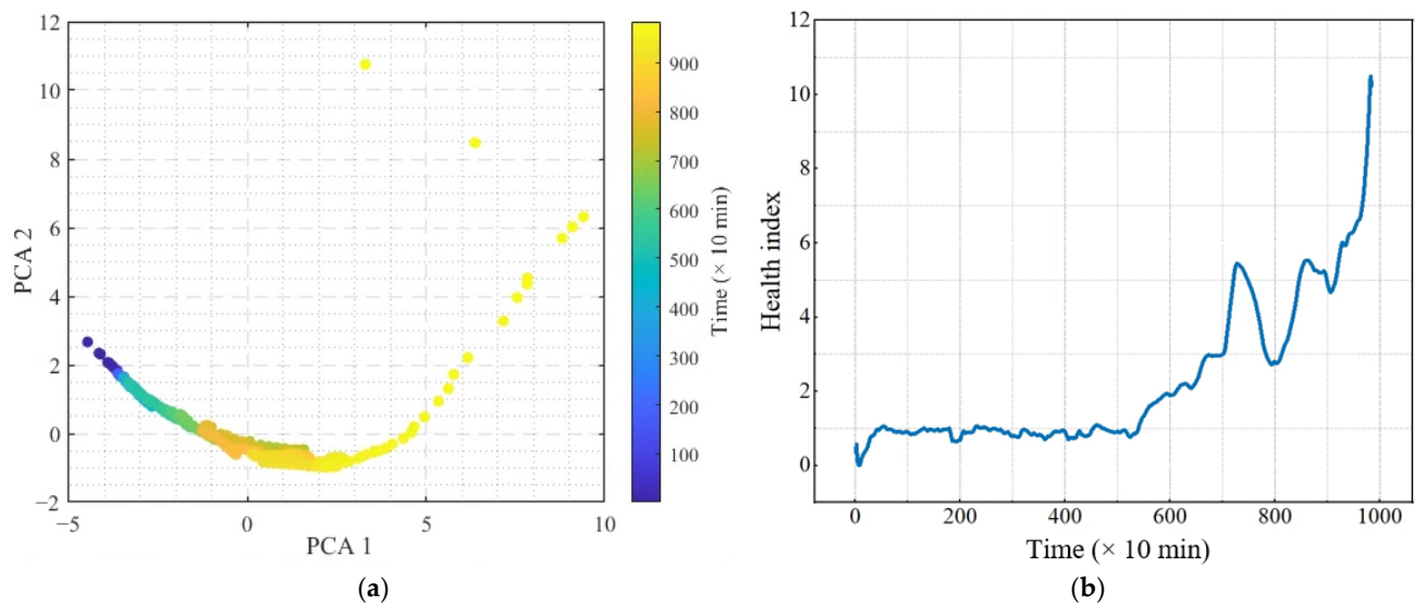
Figure 4. (a) The principal component; (b) HI was built from features selected.
