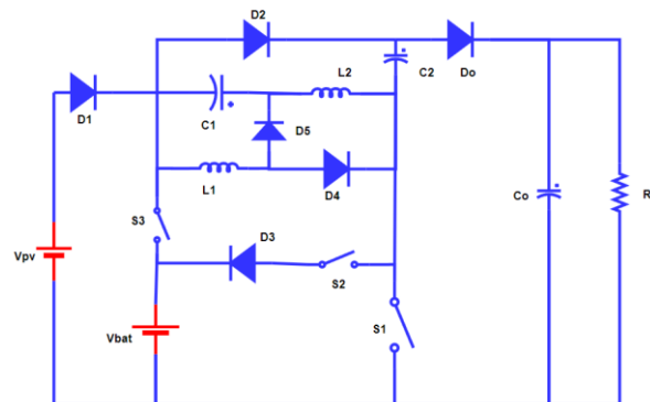
Figure 24. Circuit of the proposed dual-input bidirectional DC-DC converter.
