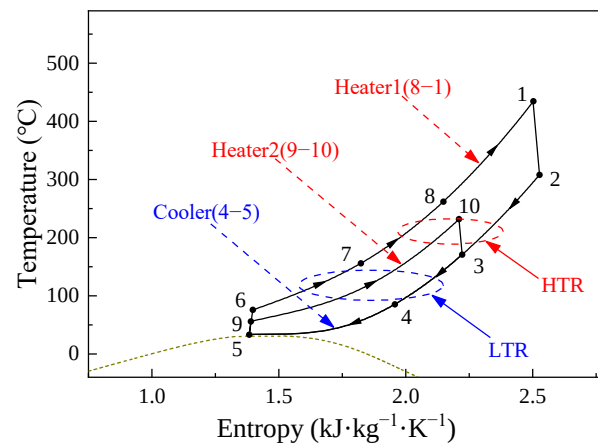
Figure 2. Temperature entropy diagram of the system.
