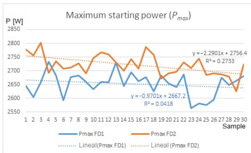
Figure 5. Maximum instantaneous starting power for two measurement series.
