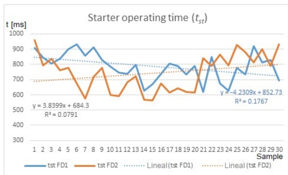
Figure 7. Starter operating time for two measurement series.
