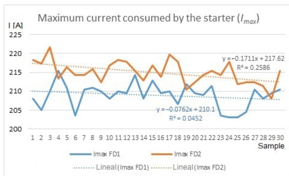
Figure 3. Values of the maximum current consumed by the starter for two measurement series.
