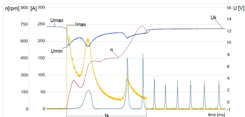
Figure 2. Chart describing the recorded parameters of the start-up process.
