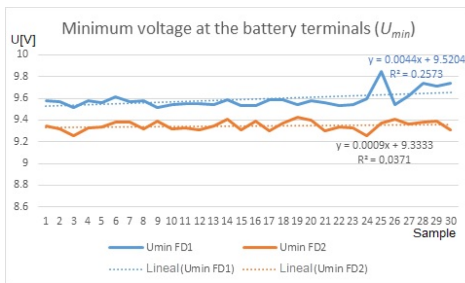
Figure 4. Minimum voltage at the battery terminals at start-up for two measurement series.
