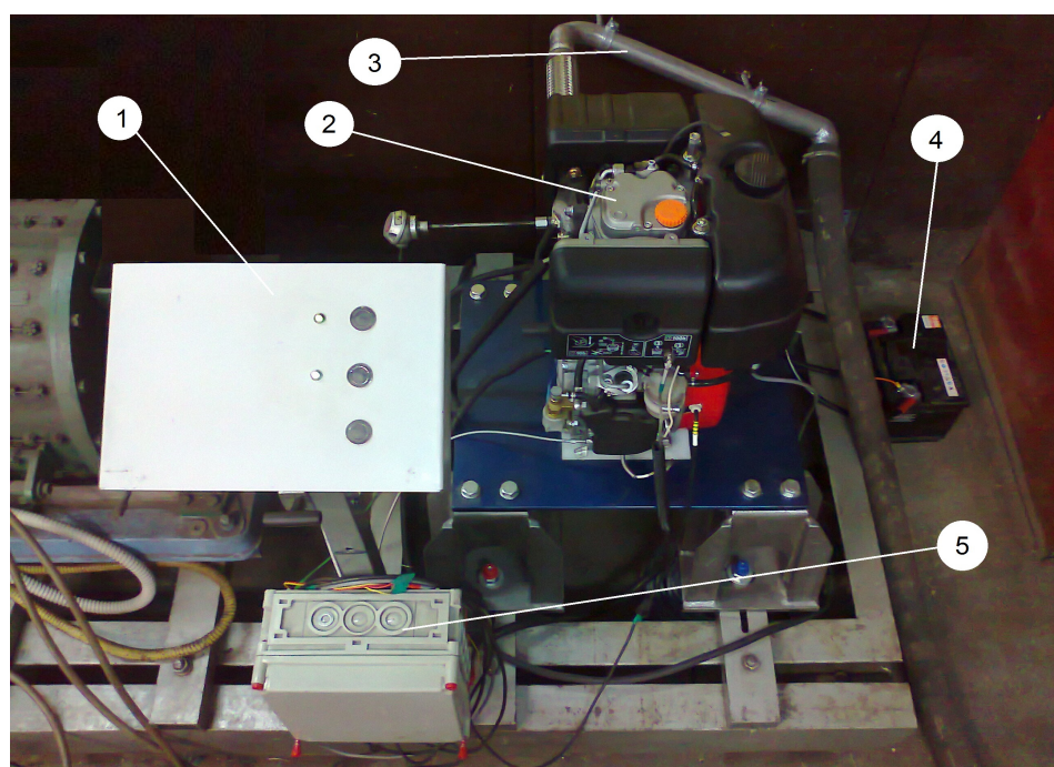
Figure 1. View of the research stand: 1—control panel, 2—research engine, 3—exhaust gas discharge system, 4—starting battery, 5—connection of measurement signals [78].
