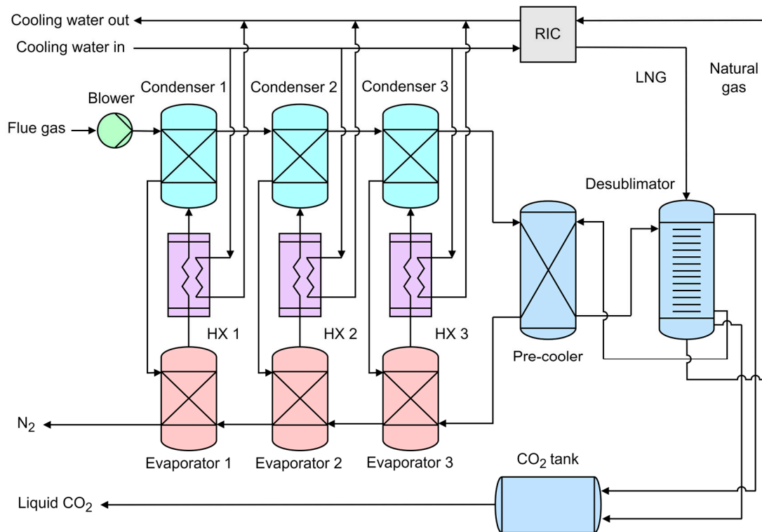
Figure 9. Process flow diagram of the AnSU technology [54].
