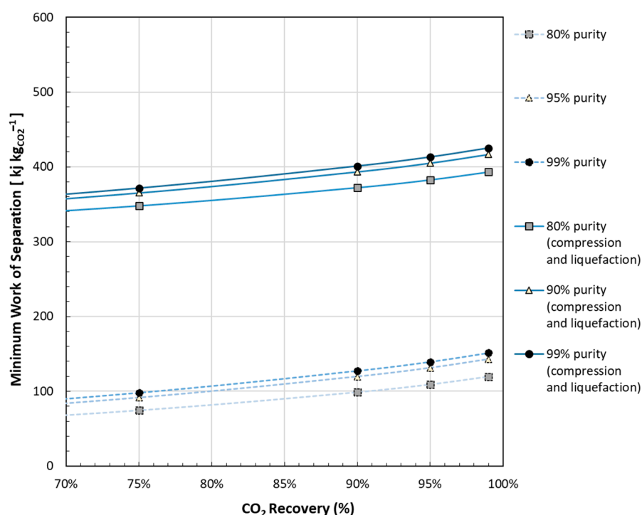
Figure 2. Minimum work of separation to obtain purified CO 2 streams from a 15% CO 2 feed stream as a function of CO 2 recovery in the solid phase. The dotted lines represent the minimum work of separation only. Continuous lines represent the total minimum work of separation, including the work of CO 2 compression and liquefaction.
