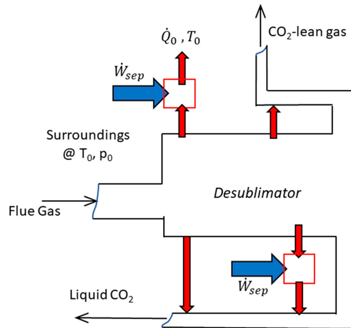
Figure 3. Schematic of a cryogenic desublimator used for theoretical calculations [22].
