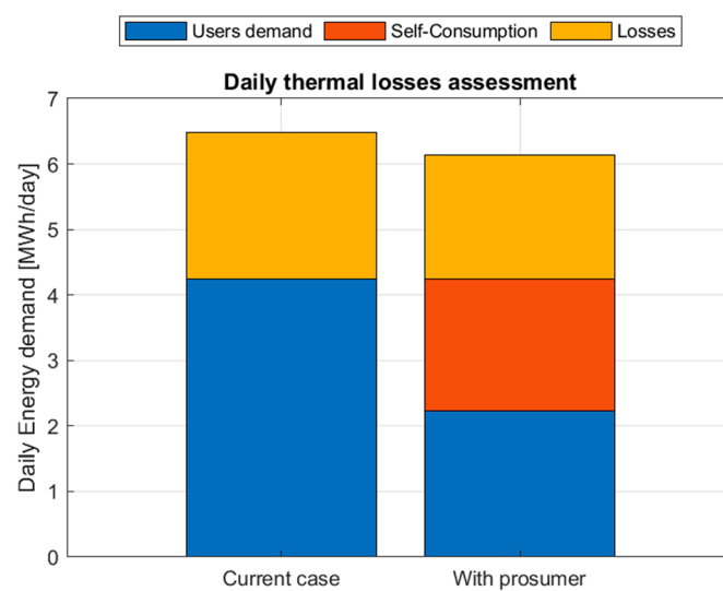
Figure 13. Evaluation of the thermal losses during a day with respect to the total users' demand in the current case ( left ) and with the installation of a thermal prosumer ( right ) with Configuration 1A.
