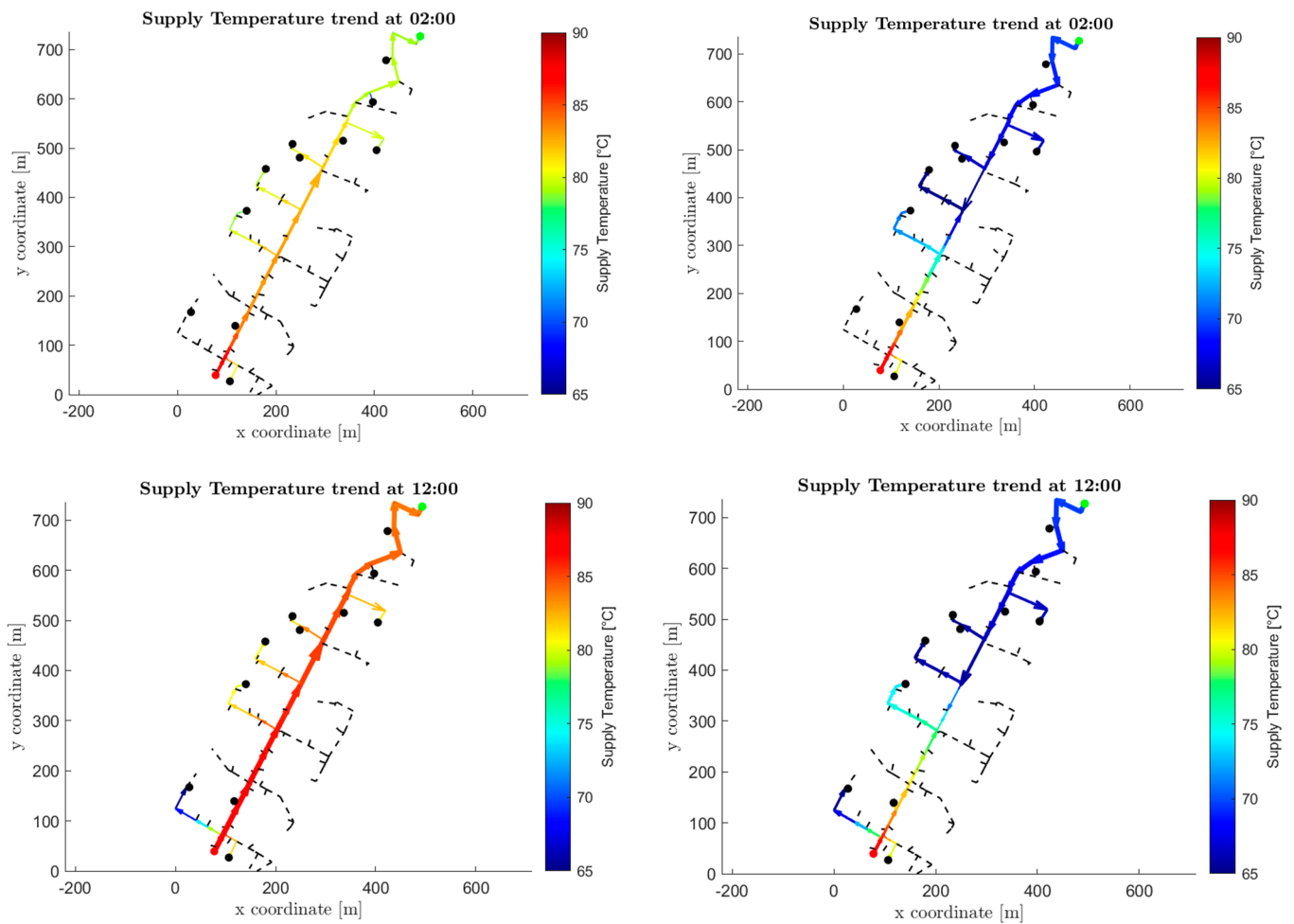
Figure 12. Temperature distribution (color bar reported in the right) in the distribution network in the current case ( left ) and with installation of a thermal prosumer ( right ) with Configuration 1A. The connection node to the main network is shown in red; the users with domestic hot water demand are highlighted in black; and the prosumer location is indicated in green.
