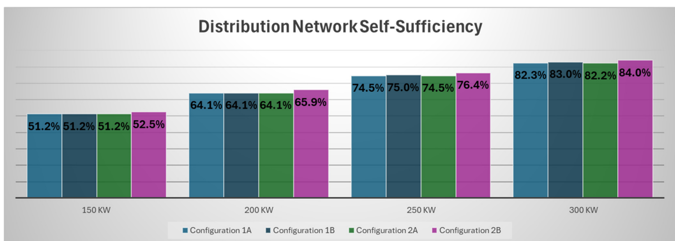
Figure 9. Network self-sufficiency: comparison between scenarios and different HP sizes.
