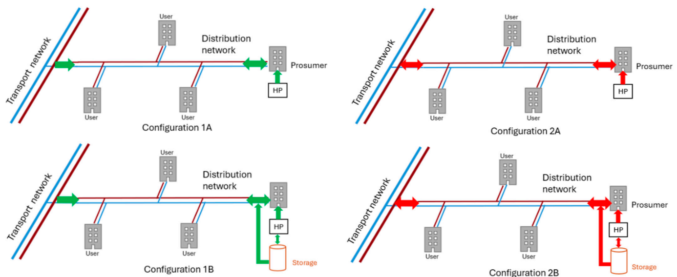
Figure 1. Schematic diagrams of the four configurations: local distribution sharing (left) and injection into the transport network (right). The two configurations at the top are without storage; the two below include storage. The red line indicates the supply line, blue ones indicates the return. The arrows show the thermal power exchanges for the two configurations (green for Configuration 1, red for Configuration 2).
