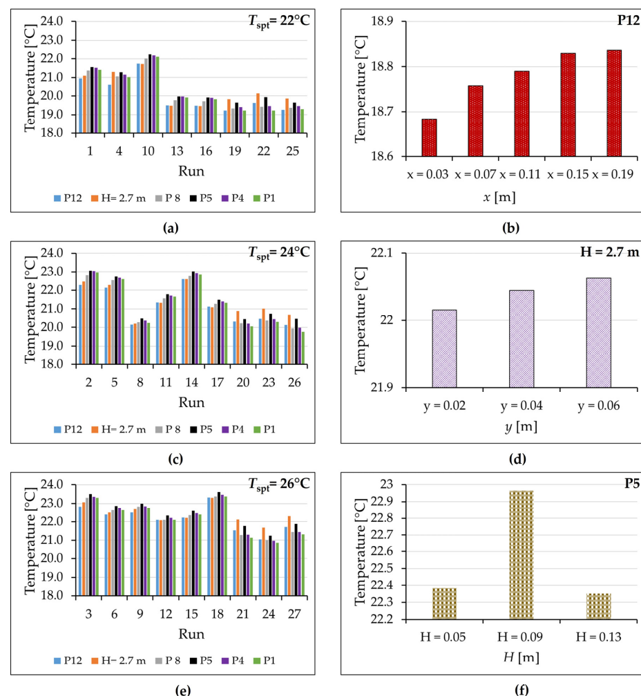
Figure 5. Wall confluent jet temperature in Zone I at P12, Zone II at H = 2.7 m, and Zone II at P1, P4, P5, and P8 in summer and autumn. (a) WCJ temperature with runs at T_{\text{spt}} = 22^\circ\text{C} , (b) WCJ
