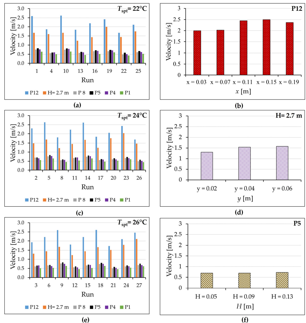
Figure 4. Wall confluent jets (WCJ) velocity along the ceiling (P12), external wall ( H = 2.7 m), and floor positions (P1, P4, P5, and P8) in summer and autumn: (a) WCJ velocity with runs at T_{spt} = 22^\circ\text{C} (b) WCJ velocity distribution in the boundary layer in Zone I at P12, (c) WCJ velocity with runs at T_{spt} = 24^\circ\text{C} , (d) WCJ velocity distribution in the boundary layer Zone II at H = 2.7 m, and (e) WCJ velocity with runs at T_{spt} = 26^\circ\text{C} , and (f) WCJ velocity distribution in the boundary layer in Zone III at P5. Note: x , y and H are the perpendicular distances from the ceiling, inner surface of the external wall and the floor into the room, respectively.
