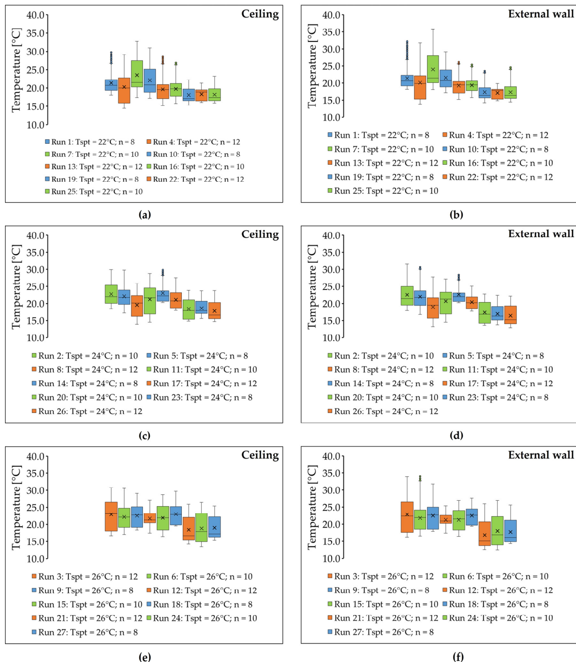
Figure 6. Ceiling surface temperature and inner surface temperature of external wall: (a) ceiling surface temperature for runs at T_{spt} = 22^\circ\text{C} , (b) inner surface temperature of external wall for runs at T_{spt} = 22^\circ\text{C} , (c) ceiling surface temperature for runs at T_{spt} = 24^\circ\text{C} , (d) inner surface temperature of external wall for runs at T_{spt} = 24^\circ\text{C} , (e) ceiling surface temperature for runs at T_{spt} = 26^\circ\text{C} , and (f) inner surface temperature of external wall for runs at T_{spt} = 26^\circ\text{C} . Note that blue represents runs with n = 8 , green represents runs with n = 10 , and orange represents runs with n = 12 .
