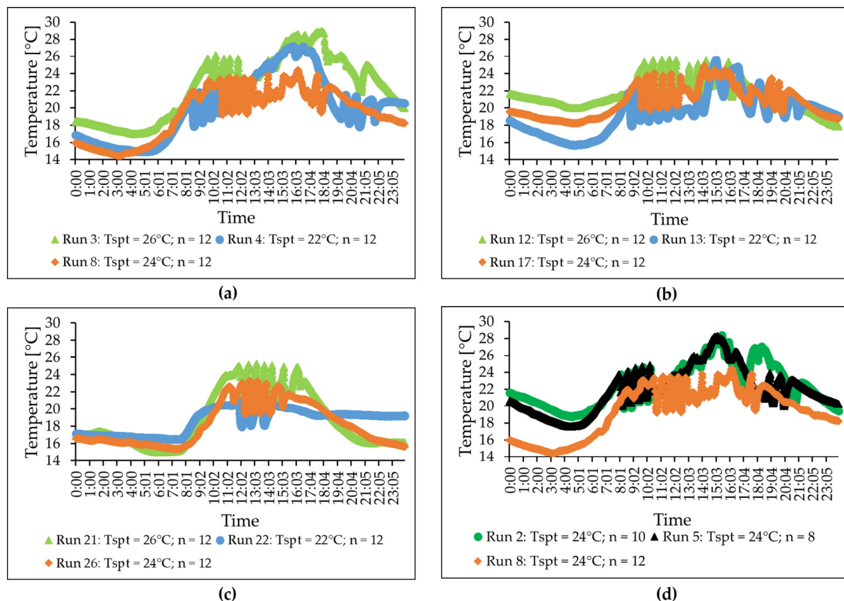
Figure 9. Variation in room air temperature: (a), influence of room air temperature setpoint ( T_{\text{spt}} ) in summer at n = 12 with unshaded external wall, (b), influence of room air temperature setpoint ( T_{\text{spt}} ) in summer at n = 12 with shaded external wall, (c), influence of room air temperature setpoint ( T_{\text{spt}} ) in autumn at n = 12 with unshaded external wall, (d) effect of number of nozzle rows in summer at T_{\text{spt}} = 24^\circ\text{C} .
