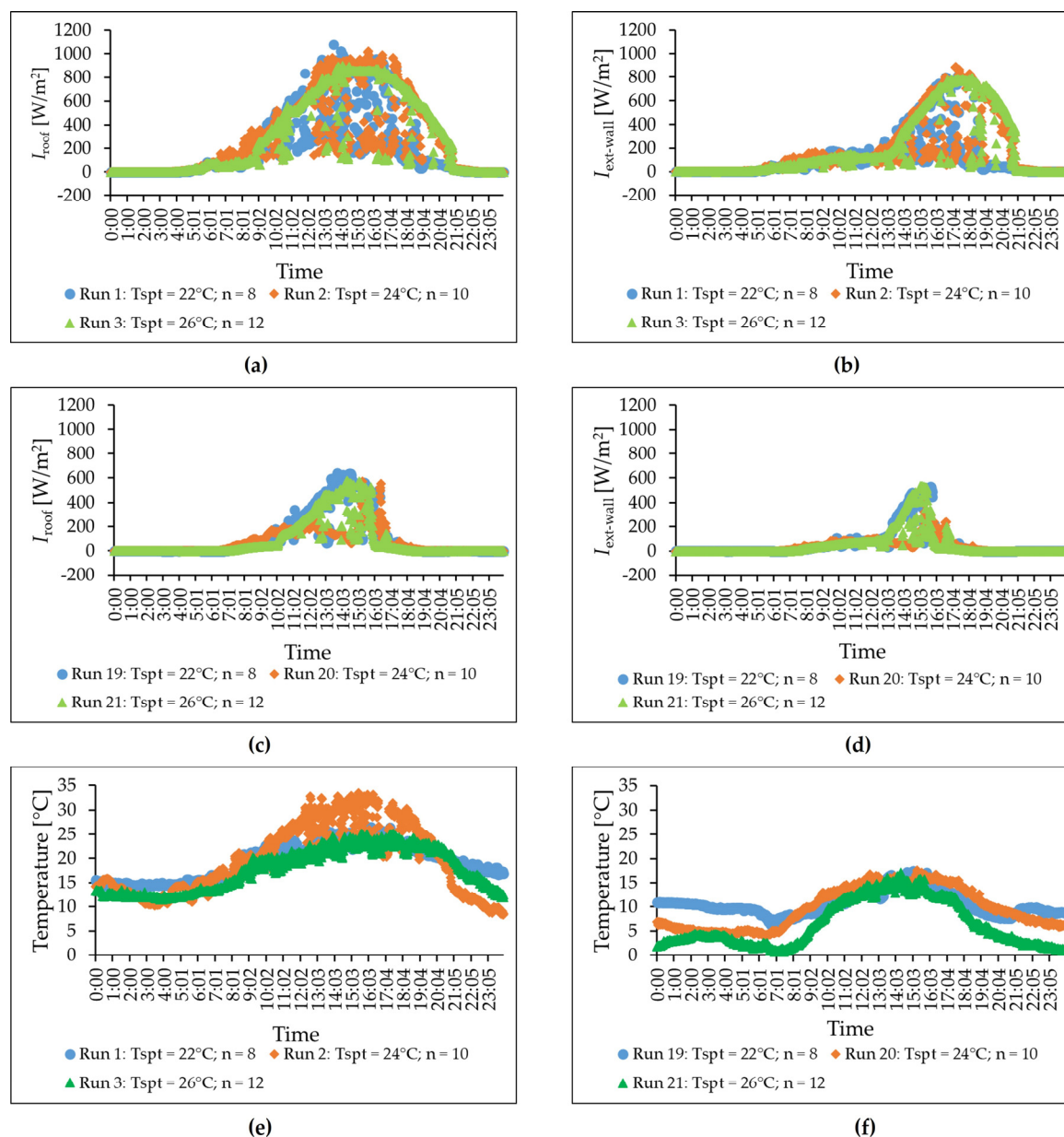
Figure 3. Time-series of external climate conditions during selected experimental runs: (a) incident solar radiation on the roof in summer, (b) incident solar radiation on the external wall in summer, (c) incident solar radiation on the roof in autumn, (d) incident solar radiation on the external wall in autumn, (e) outdoor air temperature in summer, and (f) outdoor air temperature in autumn.
