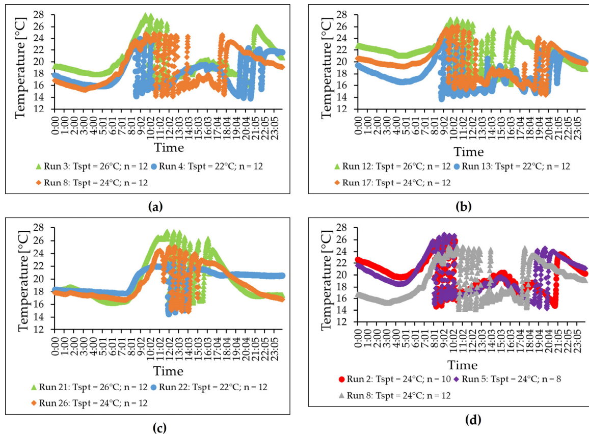
Figure 8. Variation in inlet air temperature under different experimental conditions: (a), influence of room air temperature setpoint ( T_{spt} ) in summer at n = 12 with unshaded external wall, (b), influence of room air temperature setpoint ( T_{spt} ) in summer at n = 12 with shaded external wall, (c), influence of room air temperature setpoint ( T_{spt} ) in autumn at n = 12 with unshaded external wall, (d) effect of number of nozzle rows in summer at T_{spt} = 24^{\circ}\text{C} .
