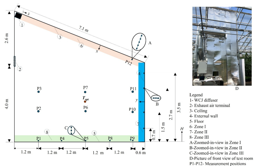
Figure 2. Side view of the test room illustrating WCJ velocity and temperature measurement zones, room air temperature measurement positions, and a front-view photo of the test room. Zoomed-in views (A, B, C) depict the orientation of constant current anemometers, while (D) shows the shaded side wall of the test room enclosed in the main greenhouse. Using constant current anemometers, the WCJ velocity and temperature measurement positions are marked as follows: H = 0.7 m, H = 1.5 m, H = 2.7 m, H = 3.5 m, P1, P4, P5, P8, P9, and P12. Room air temperature measurement positions, indicated as P2, P3, P6, P7, P10, and P11, with T_{spt} for the room air temperature setpoint.
