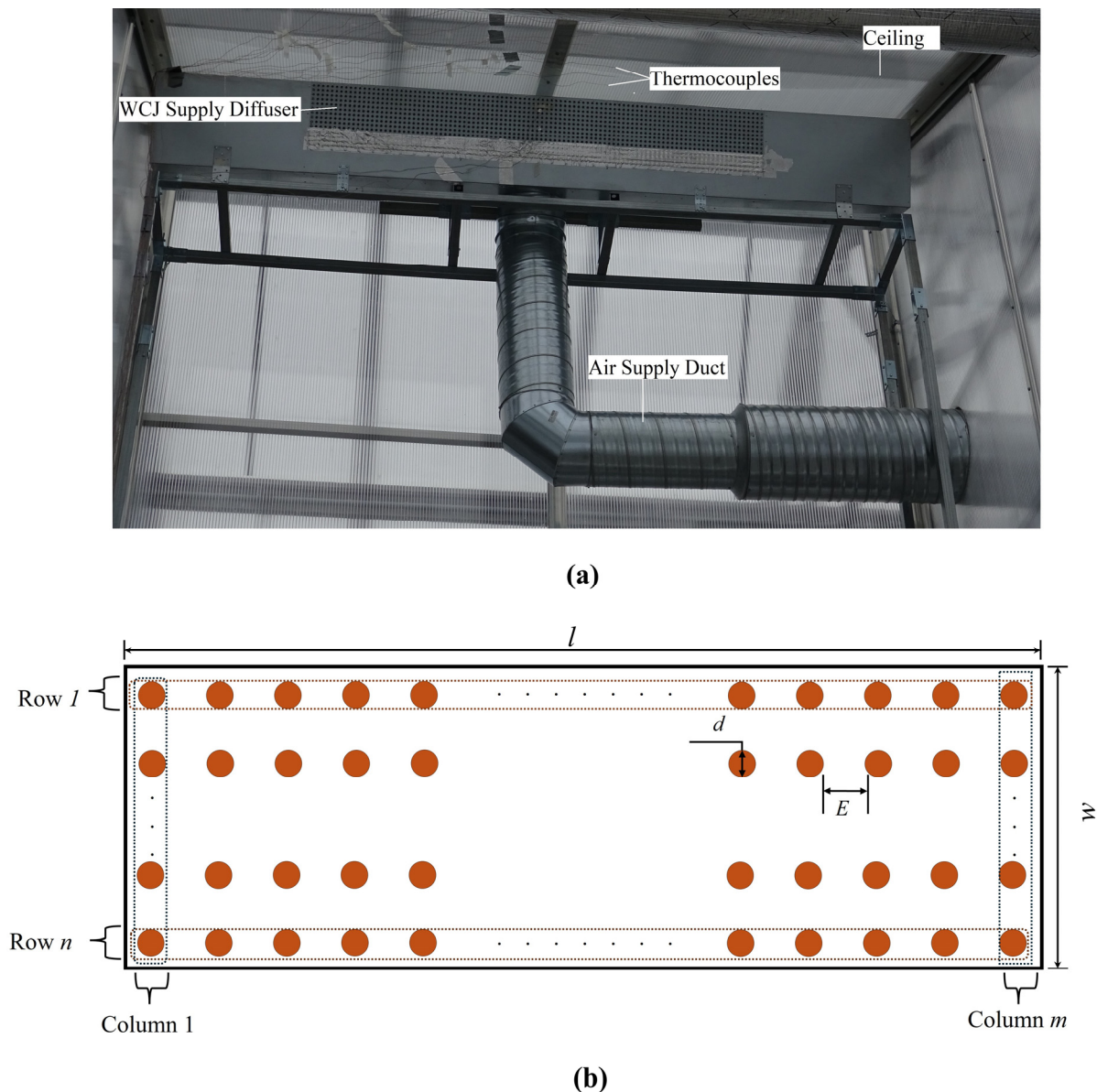
Figure 1. (a) Picture of the installed WCJ diffuser and supply air duct; (b) WCJ diffuser nozzle plate with representative nozzles. Note: d is the interior diameter of the nozzle, E is the spacing between adjacent nozzles, w is the width of the nozzle plate, l is the length of the nozzle plate, n is the number of nozzle rows, and m is the number of nozzle columns.
