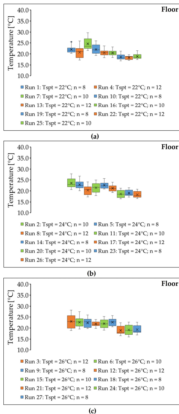
Figure 7. Floor surface temperature: (a) for runs with T_{spt} = 22^\circ\text{C} , (b) for runs with T_{spt} = 24^\circ\text{C} , and (c) for runs with T_{spt} = 26^\circ\text{C} . Note that blue represents runs with n = 8 , green represents runs with n = 10 , and orange represents runs with n = 12 .
