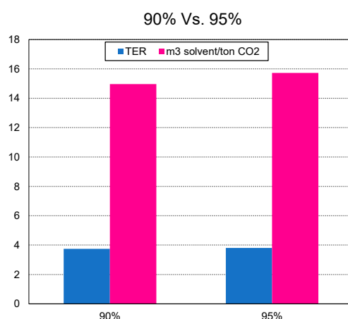
Figure 6. TER and m 3 solvent/ton CO 2 for the two optimum considered cases.
