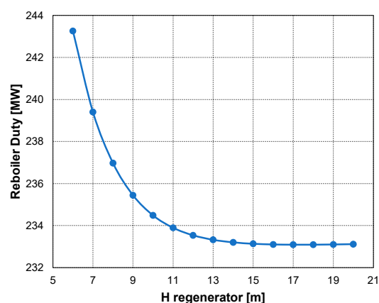
Figure 4. Dependence of the reboiler duty on the regenerator height with H_{\text{abs}} = 20 m and \alpha = 0.2 mol \text{CO}_2 /mol MEA.
