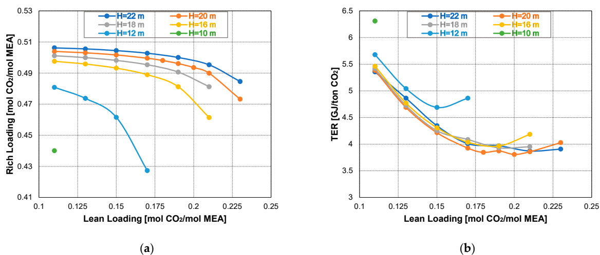
Figure 3. Influences of the absorber packing height and lean loading on (a) rich loading and (b) TER.
