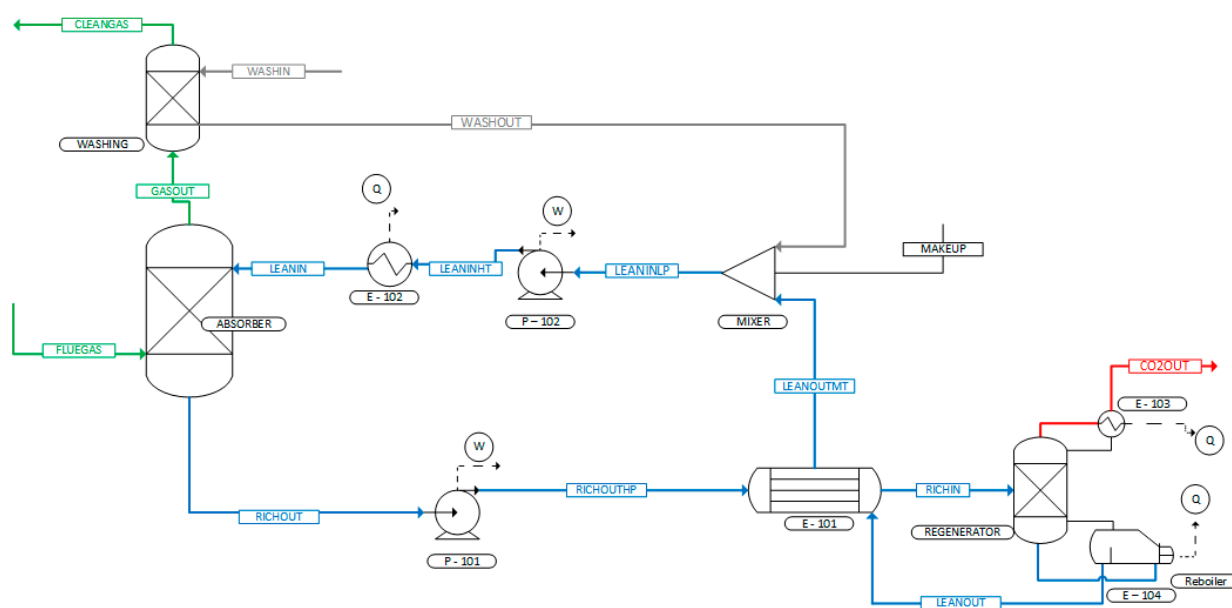
Figure 2. Process flow diagram of the designed 95% CO 2 removal section in the considered steel plant.
