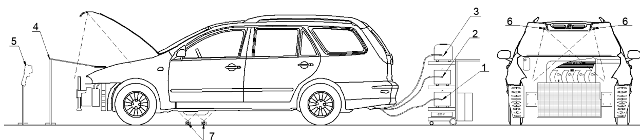
Figure 1. Scheme of the experimental setup of the study: 1—gas analyzer, Texa Gasbox (TEXA S.p.A., Monastier di Treviso, Italy); 2—gas analyzer, Brain Bee AG-200 (Brain Bee S.p.A., Parma, Italy); 3—diffusion charging (DC) particle number concentration (PNC) (TEXA S.p.A., Monastier di Treviso, Italy); 4—microphone, USB Noise Meter (Spl-Lab, The Woodlands, TX, USA); 5—thermal imaging camera, RayThink RM200F (Raythink Technology Co., Ltd., Shenzhen, China); 6 and 7—thermal imaging camera, Melexis MLX90640 (Melexis NV, Tessenderlo, Belgium).
