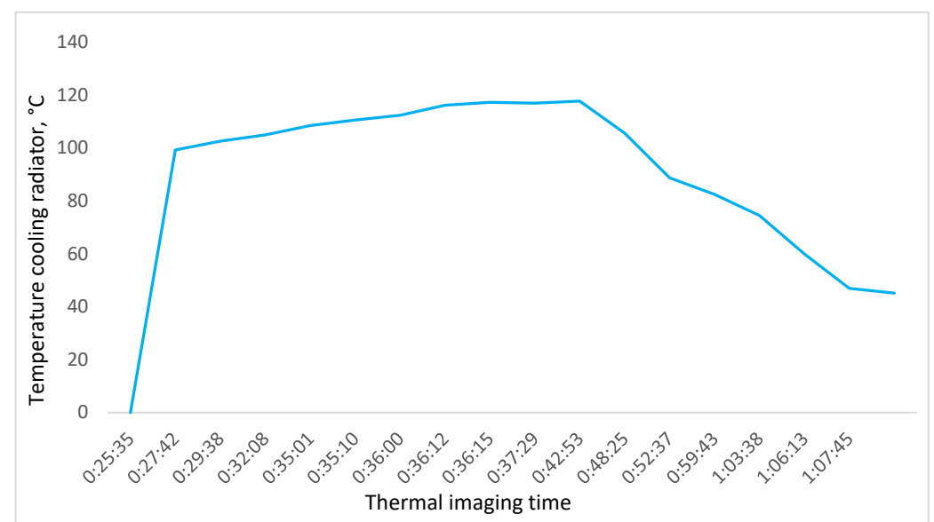
Figure 13. Cooling radiator surface temperature (IR) vs. time.
