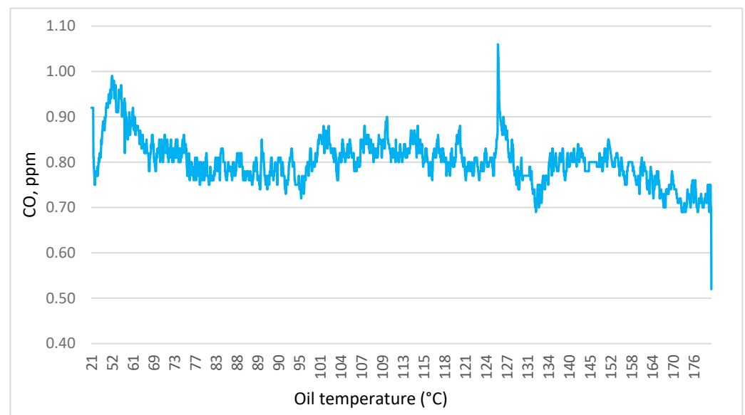
Figure 16. Carbon monoxide (CO) concentration as a function of engine oil temperature during idling without forced cooling.
