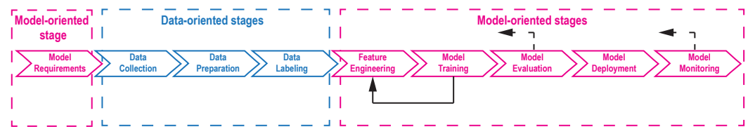
Figure 6. The nine stages of the ML workflow. Source: Authors' work.
