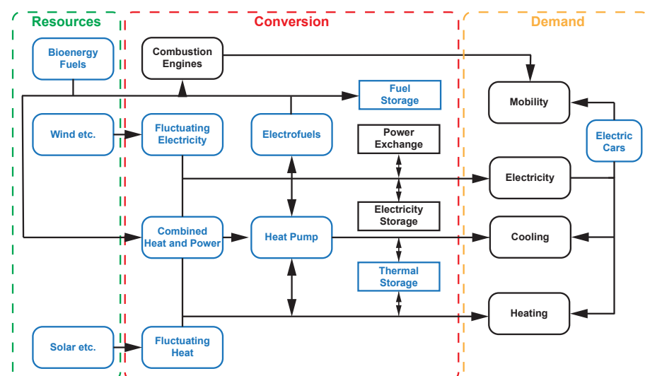
Figure 9. Interaction between sectors and technologies in a future smart energy system.
