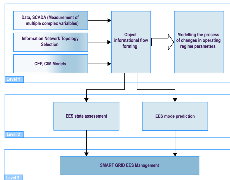
Figure 11. Organization for managing the information flow in monitoring and controlling the smart grid implemented by AI. Source: Authors' work.
