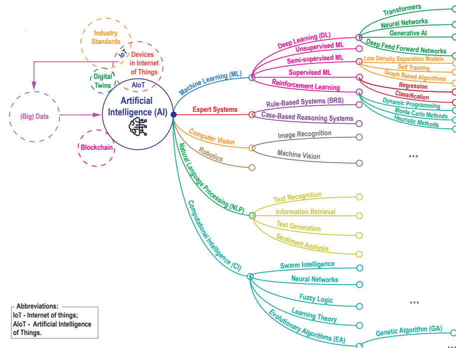
Figure 4. Taxonomy of hierarchical levels of AI, ML, and DL and their interaction with digital energy components. Note: The figure provides an overview of some basic types of AI. Within these categories, there are numerous other AI technologies and subfields, as well as opportunities for combinations between them. AI research is a dynamic field, with new advances continually emerging. Source: Authors' work.
