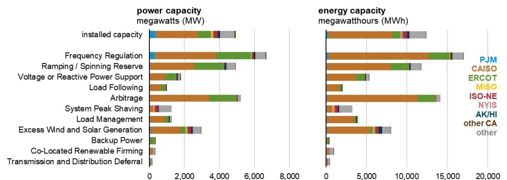
Figure 17. The distribution of large-scale battery storage application for power grid needs.
