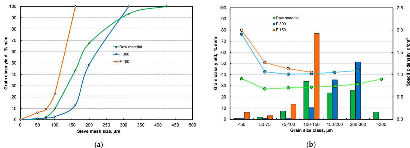
Figure 4. Microsphere raw material and two products obtained as result of basic refining processes: (a) grain size distribution, (b) yields of grain size classes and their density.
