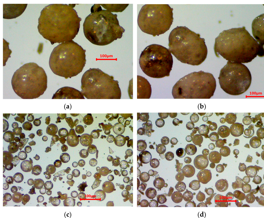
Figure 6. Transmitted light optical microscope images of the tested microspheres: (a,b)—grain size class 150–200 \mu\text{m} ; (c,d)—grain size class <75 \mu\text{m} .
