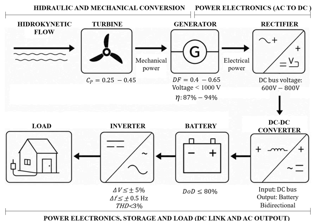
Figure 2. Electrical power system components of a residential hydrokinetic turbine and their contribution to system resilience.
