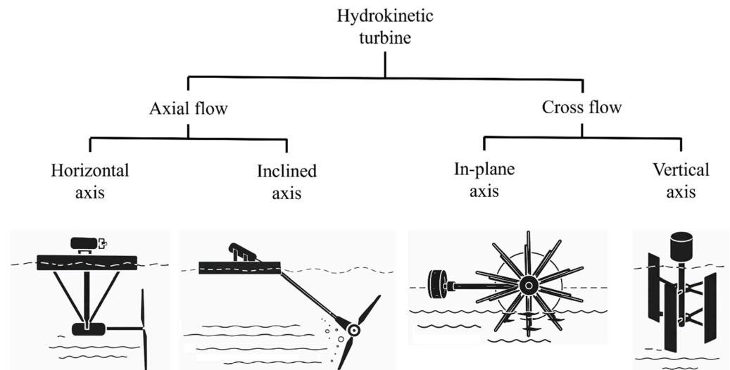
Figure 5. Representative configurations of hydrokinetic turbines for river applications. Dashed lines indicate the approximate water free surface.
