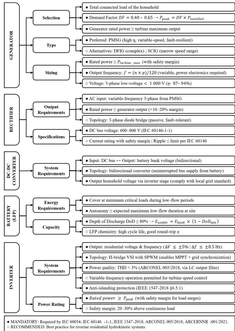
Figure 3. Criteria for selecting electrical components in residential hydrokinetic systems with emphasis on reliability and resilience.
