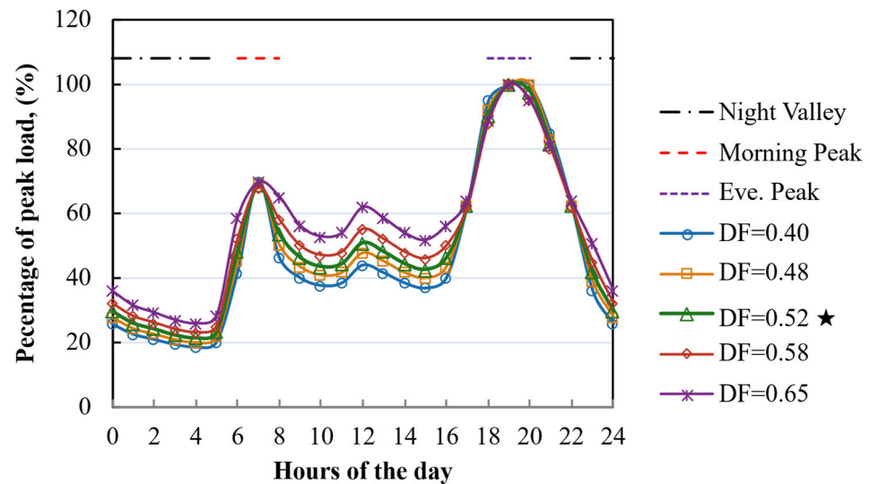
Figure 6. Representative daily load curves for residential loads. The star identifies the demand factor ( DF = 0.52 ) adopted for the Napo River case study.
