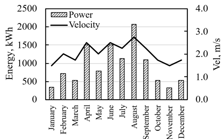
Figure 9. Monthly energy production and flow velocity variation for the selected site.
