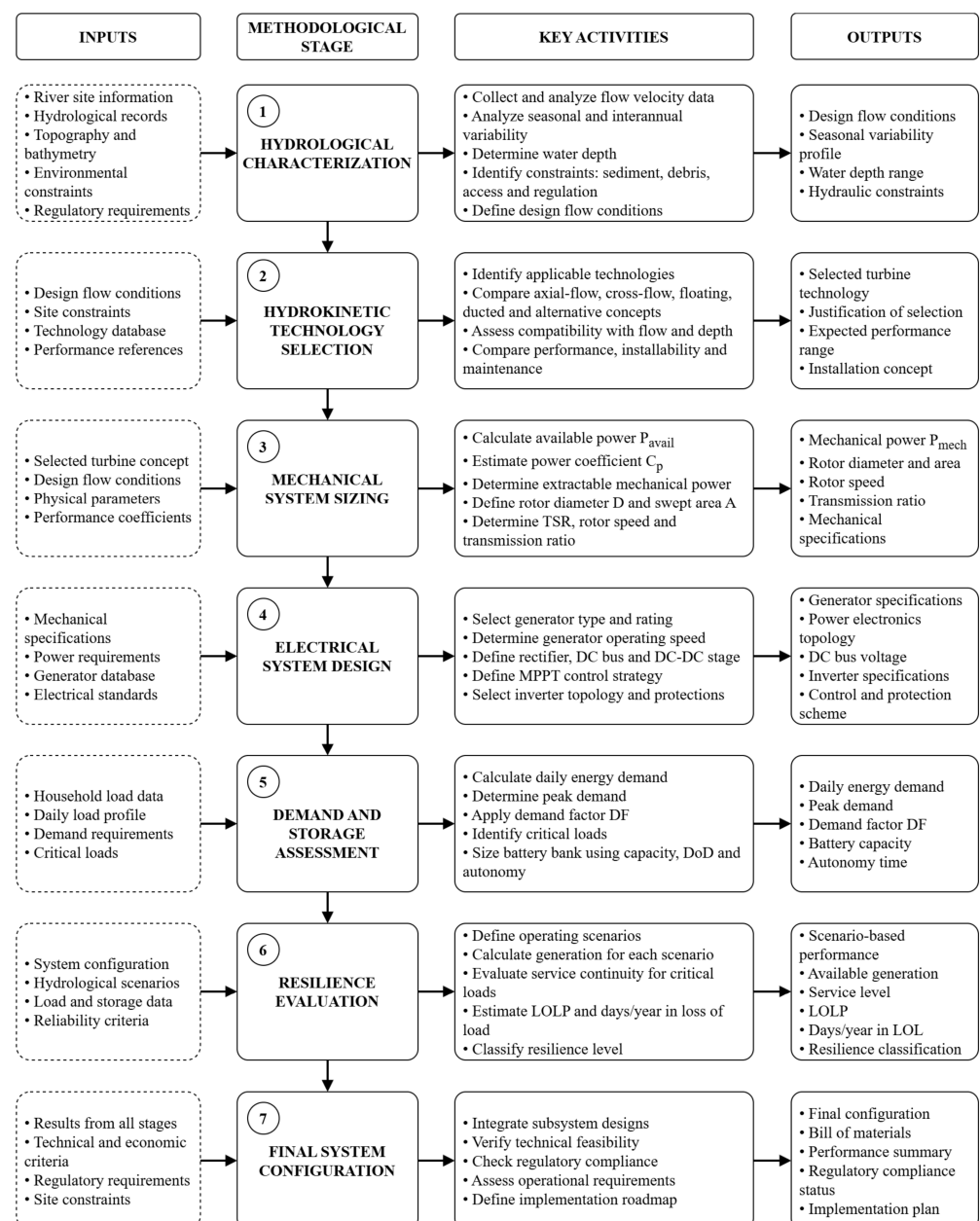
Figure 1. Proposed resilience-oriented design framework for residential hydrokinetic power systems.
