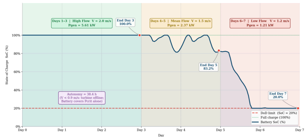
Figure 10. Battery SoC Over 7 Day Flow Scenarios.
