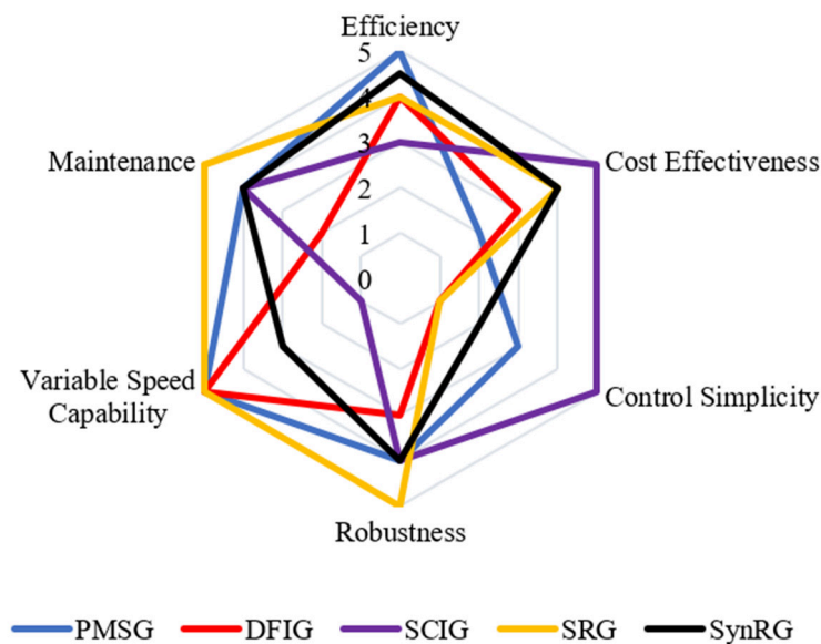
Figure 7. Generator performance comparison.
