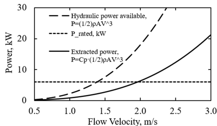
Figure 4. Power-Velocity Curve.
