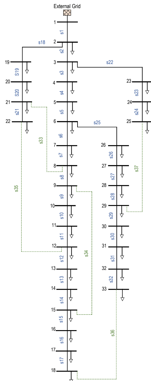
Figure 1. Single-line diagram of the IEEE 33-bus test system.
