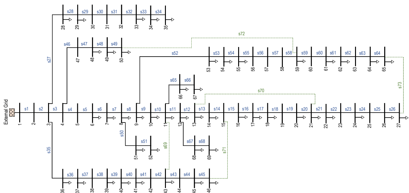
Figure 2. Single-line diagram of the IEEE 69-bus test system.
