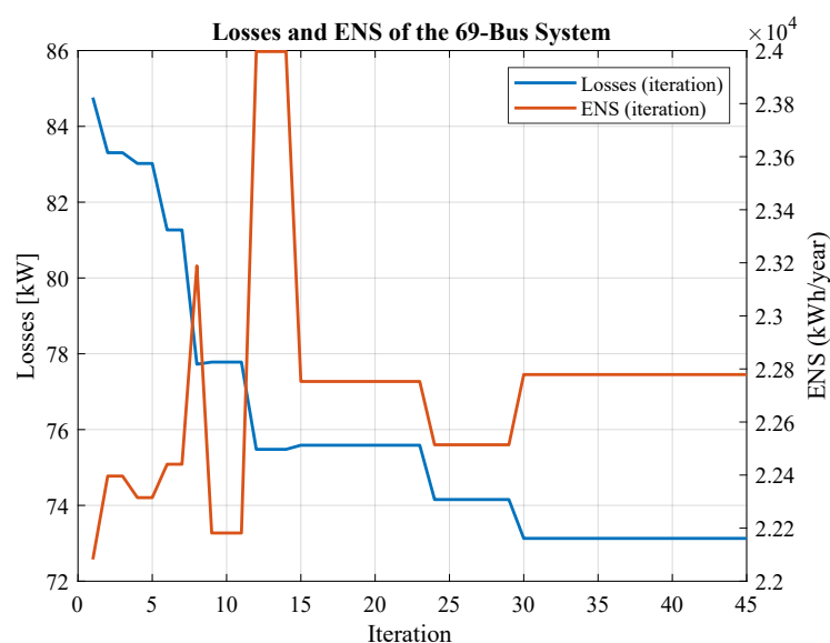
Figure 4. Comparison of losses and ENS for the IEEE 69-bus system.
