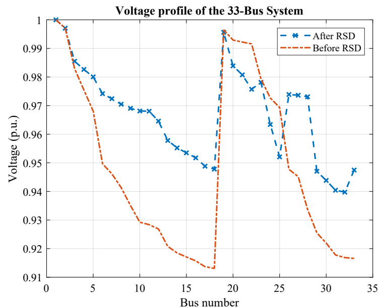
Figure 5. Voltage profile for the IEEE 33-bus system.
