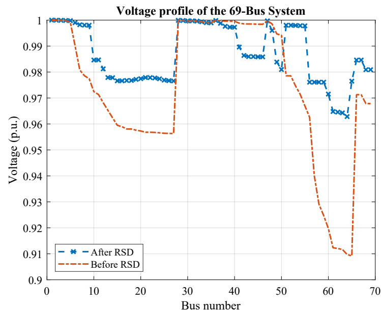
Figure 6. Voltage profile for the IEEE 69-bus system.
