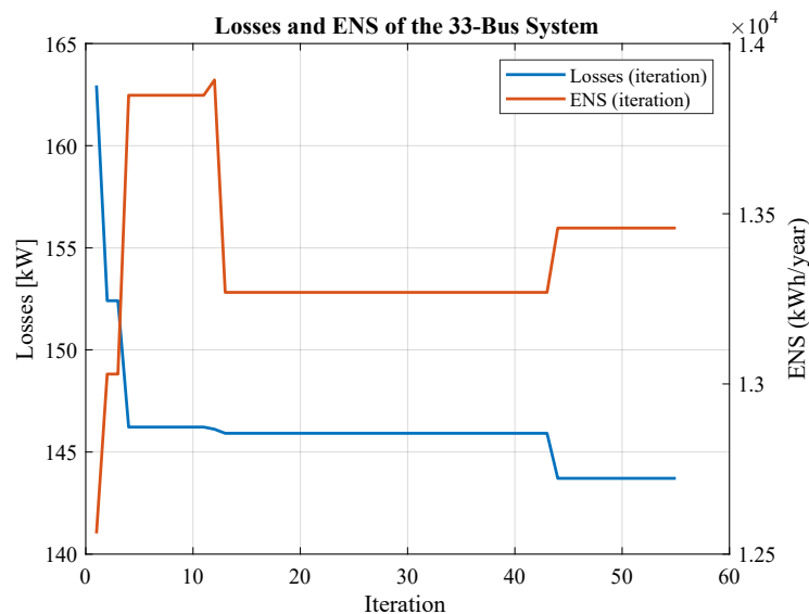
Figure 3. Comparison of losses and ENS for the IEEE 33-bus system.
