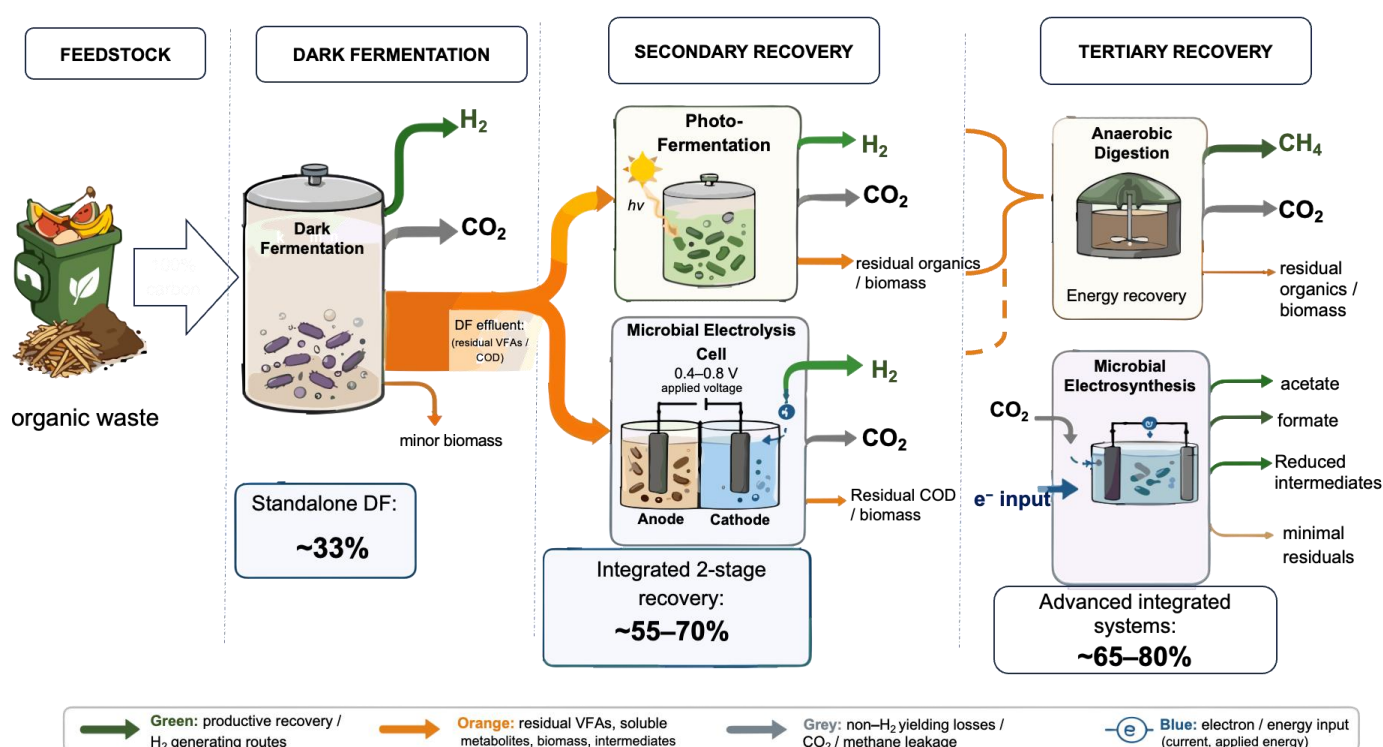
Figure 2. Carbon and electron recovery in integrated biohydrogen configurations. Cumulative carbon to H_2 recovery ranges are midpoint values derived from Tables 1 and 2 and are shown for conceptual comparison.
