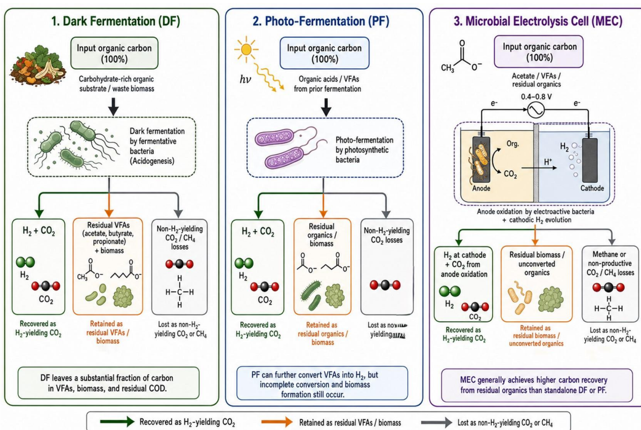
Figure 1. Carbon partitioning in standalone biohydrogen technologies. Schematic representation of the fate of input organic carbon during dark fermentation (DF), photo-fermentation (PF), and microbial electrolysis cell (MEC) operation. Numerical ranges shown reflect typical values reported for real-waste operation in the cited literature (Table 1) and are not single-source measurements.
