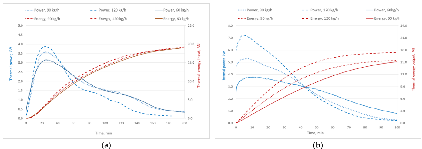
Figure 12. Thermal power and thermal energy input/output during (a) charging and (b) discharging, depending on air flow rates 60–120 kg/h. Target PCM packed-bed temperature of 290 °C.
