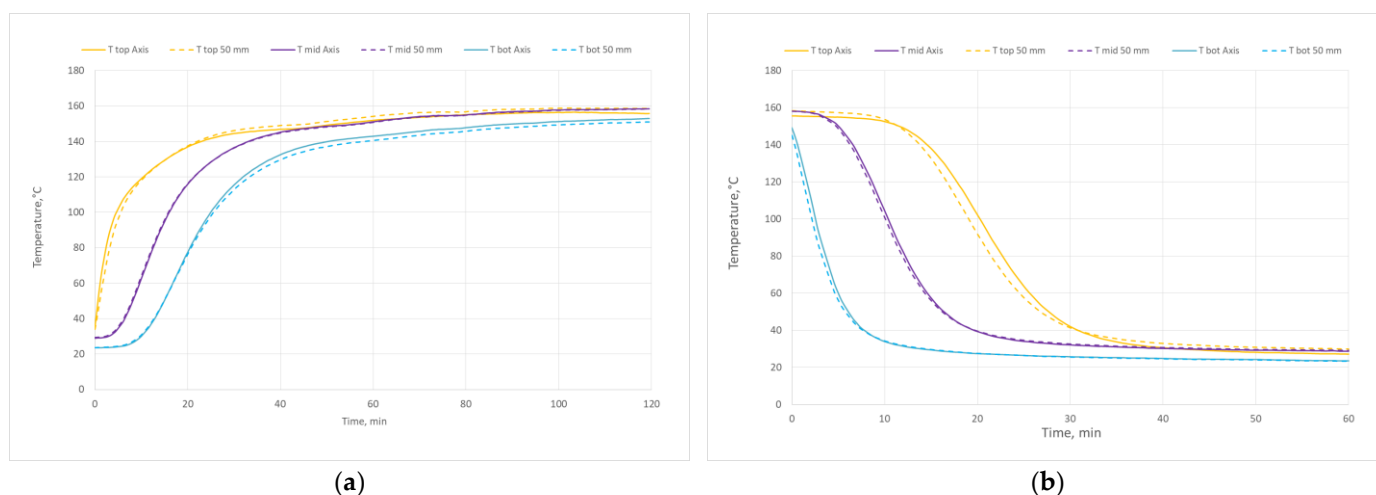
Figure 5. Temperature profile in the TES unit along the column axis and 50 mm from the axis for (a) charging and (b) discharging. Air flow rate of 120 kg/h.
