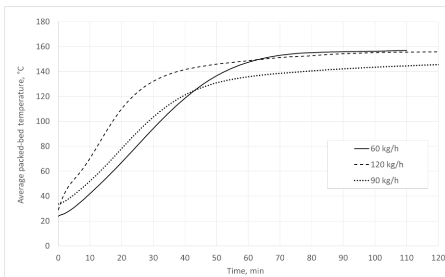
Figure A10. Average basalt packed-bed temperatures for tests B1–B3.
