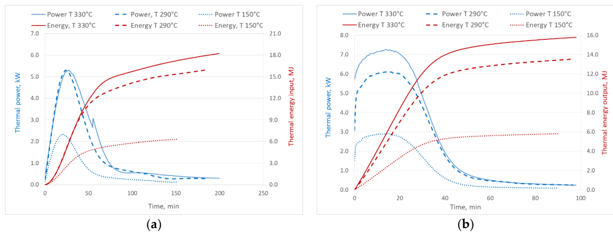
Figure A8. Thermal power and thermal energy of the TES unit depending on basalt packed-bed temperature; (a) charging and (b) discharging. Air flow rate of 90 kg/h (tests B2, B5, B8).
