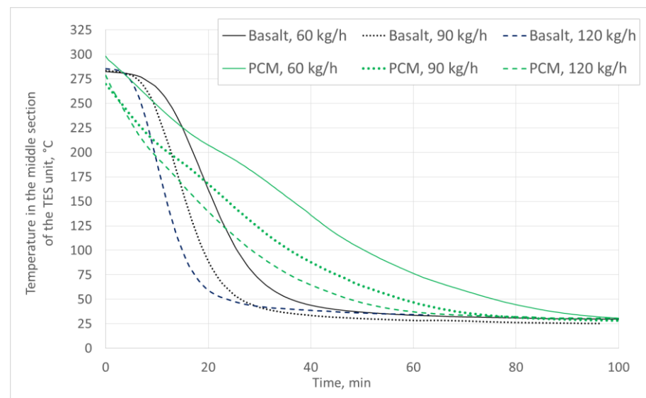
Figure 13. Comparison of temperature profiles in the middle section of the TES unit during discharging for basalt aggregate and encapsulated solar salt packed beds.
