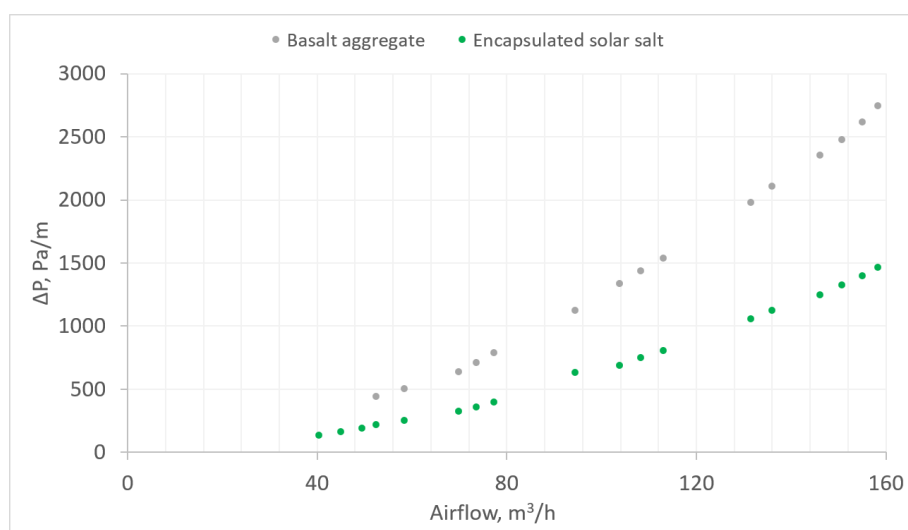
Figure A11. Measured pressure drop in the TES unit.
