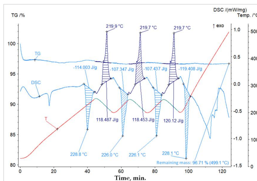
Figure 1. TG–DSC analysis of prepared phase change material (solar salt).
