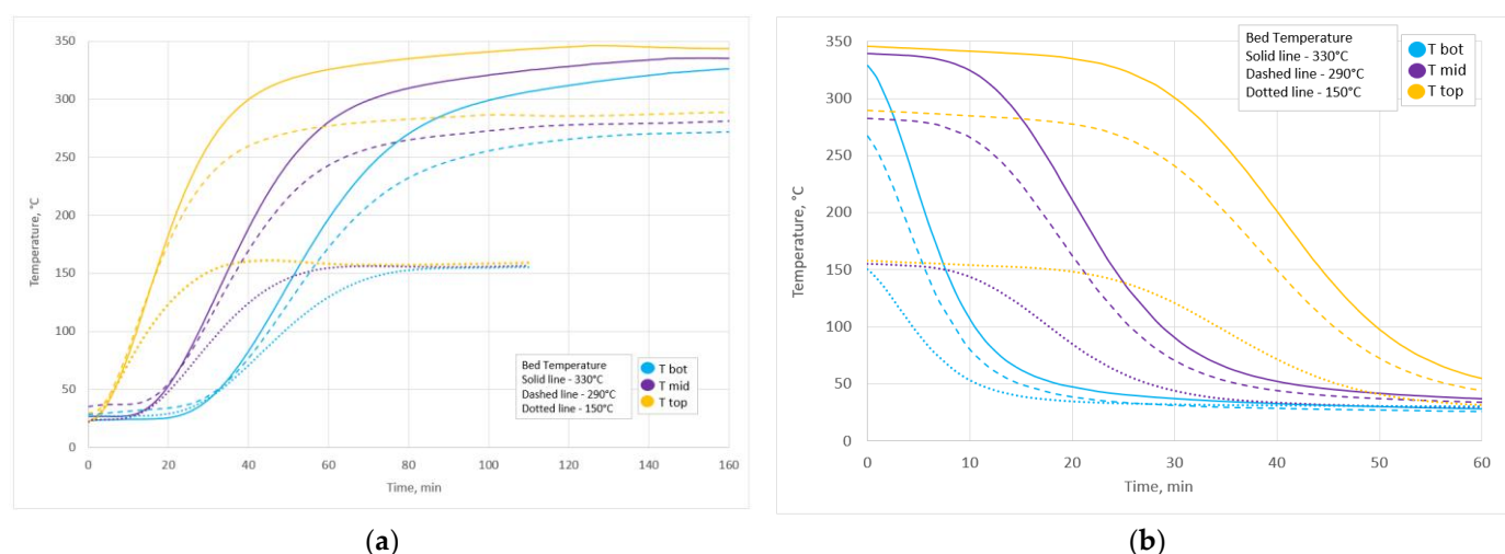
Figure 8. Temperature profiles of TES unit depending on bed temperature; (a) charging and (b) discharging. Air flow rate of 60 kg/h.
