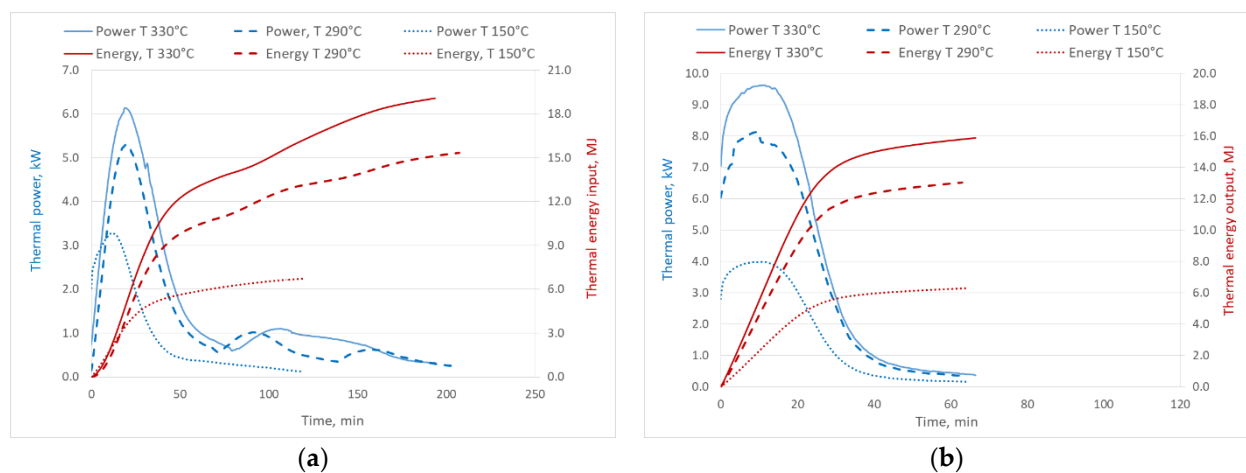
Figure A9. Thermal power and thermal energy of the TES unit depending on basalt packed-bed temperature; (a) charging and (b) discharging. Air flow rate of 120 kg/h (tests B3, B6, B9).
