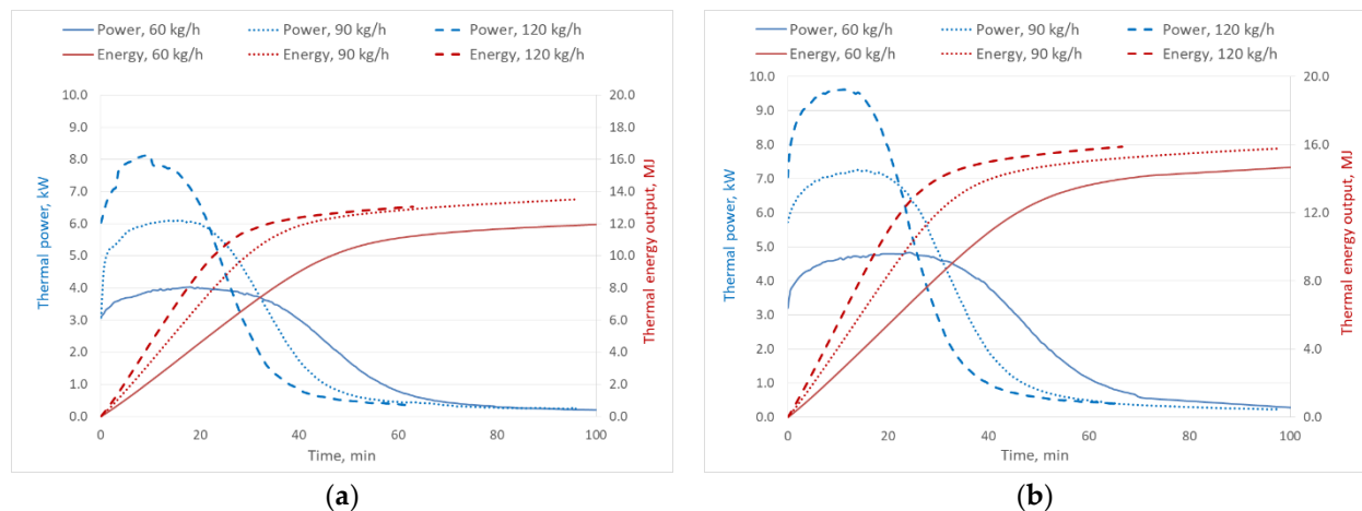
Figure A5. Thermal power and recovered energy at various air flow rates during discharging basalt packed bed at target temperatures of (a) 290 °C and (b) 330 °C (tests B4–B9).
