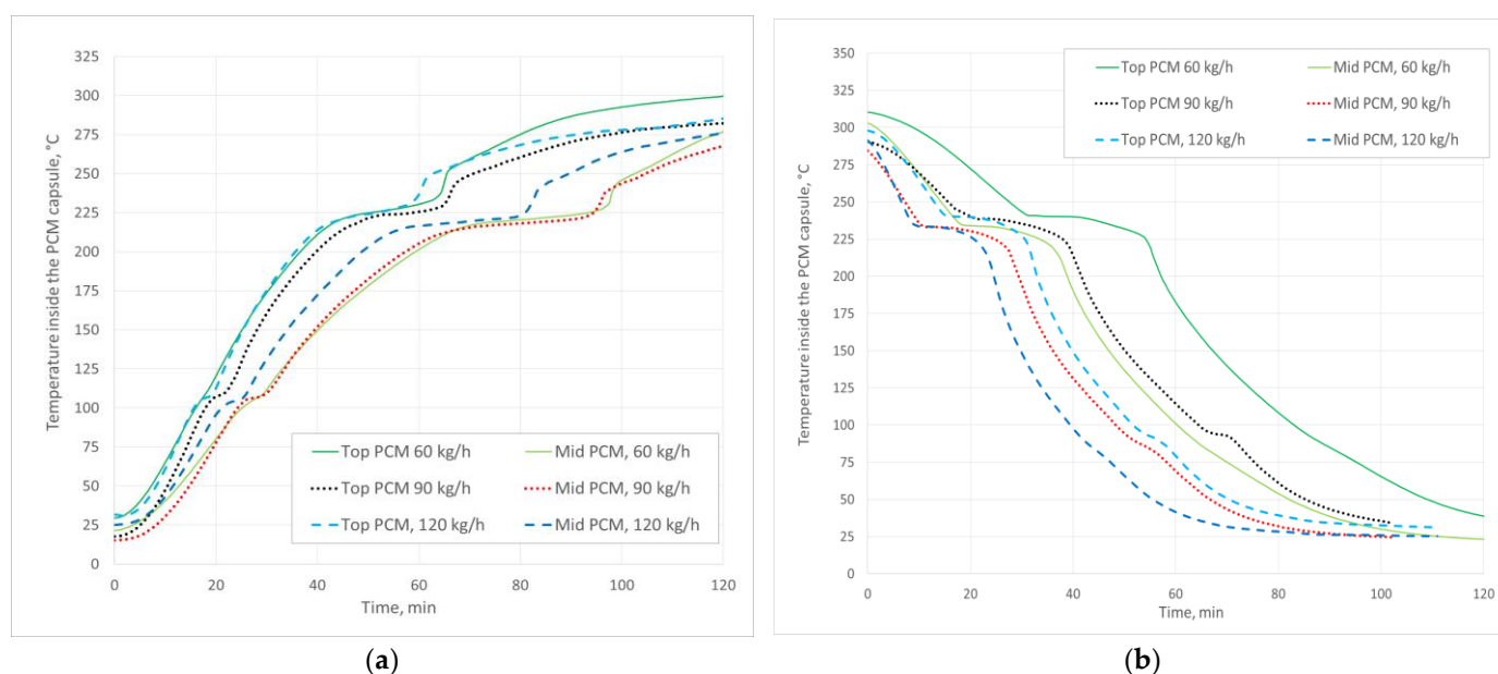
Figure 11. Temperature inside the PCM capsule during (a) charging and (b) discharging, depending on air flow rates 60–120 kg/h. Target PCM packed-bed temperature of 290 °C.
