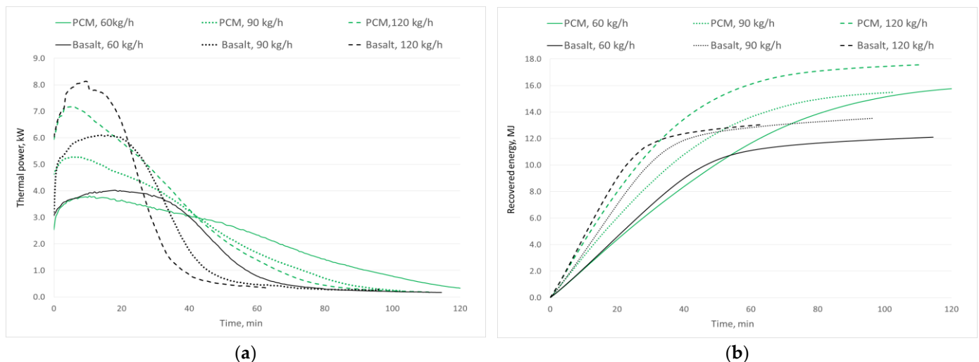
Figure 14. Comparison of (a) thermal power output and (b) recovered thermal energy during discharging for basalt aggregate and encapsulated solar salt-packed beds at different air flow rates. Target packed-bed temperature: 290 °C.
