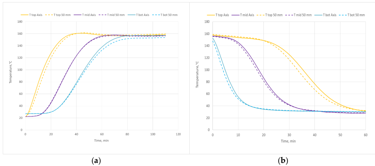
Figure A1. Temperature profiles in the TES unit along the column axis and 50 mm from the axis during (a) charging and (b) discharging. Air flow rate of 60 kg/h and target basalt packed-bed temperature of 150 °C (test B1).
