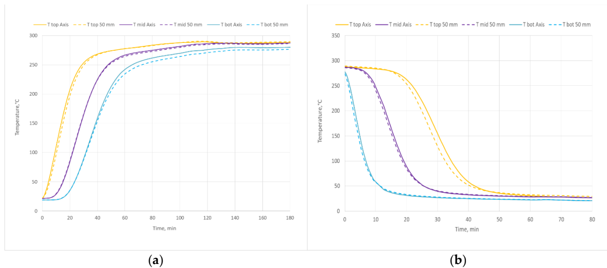
Figure A2. Temperature profiles in the TES unit along the column axis and 50 mm from the axis during (a) charging and (b) discharging. Air flow rate of 90 kg/h and target basalt packed-bed temperature of 290 °C (test B5).
