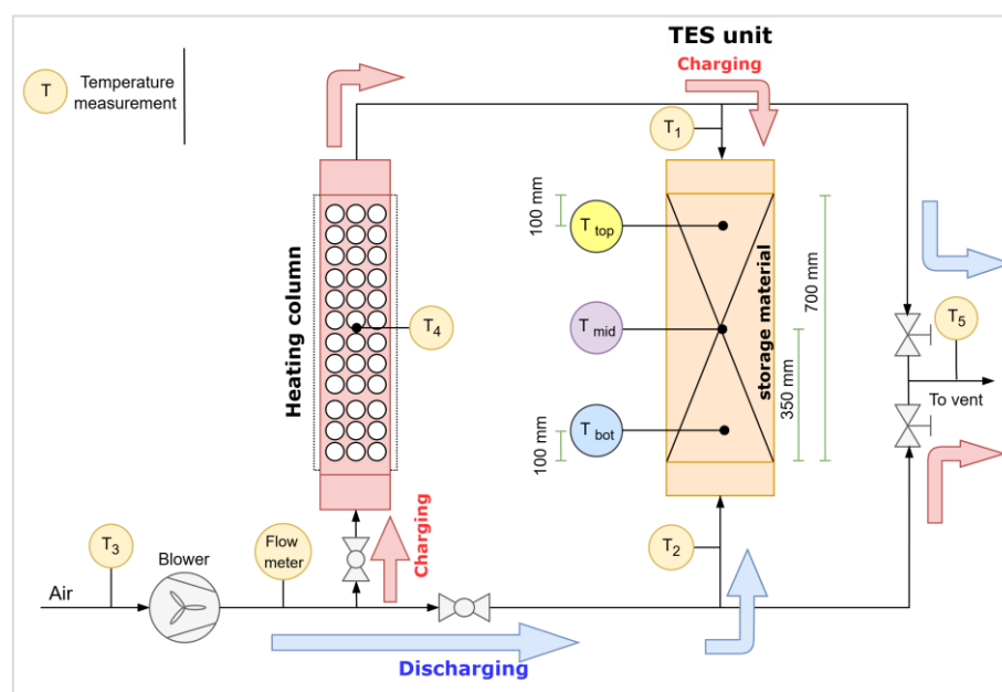
Figure 4. A schematic diagram of the test rig used in this study.
