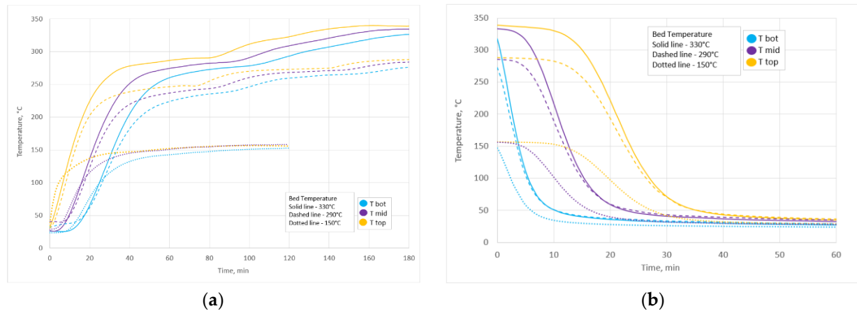
Figure A7. Temperature profiles of the TES unit depending on basalt packed-bed temperature; (a) charging and (b) discharging. Air flow rate of 120 kg/h (tests B3, B6, B9).
