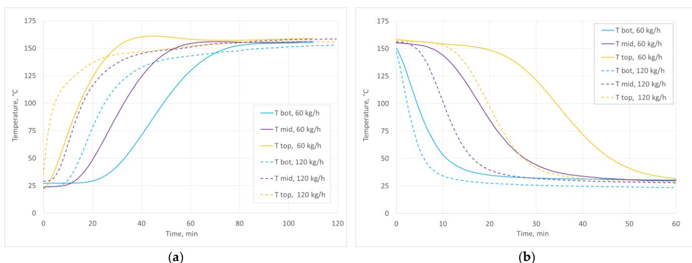
Figure 6. Comparison of axial temperature profiles for air flow rates of 60 kg/h and 120 kg/h during (a) charging and (b) discharging of the basalt packed bed. Target packed bed temperature of 150 °C.
