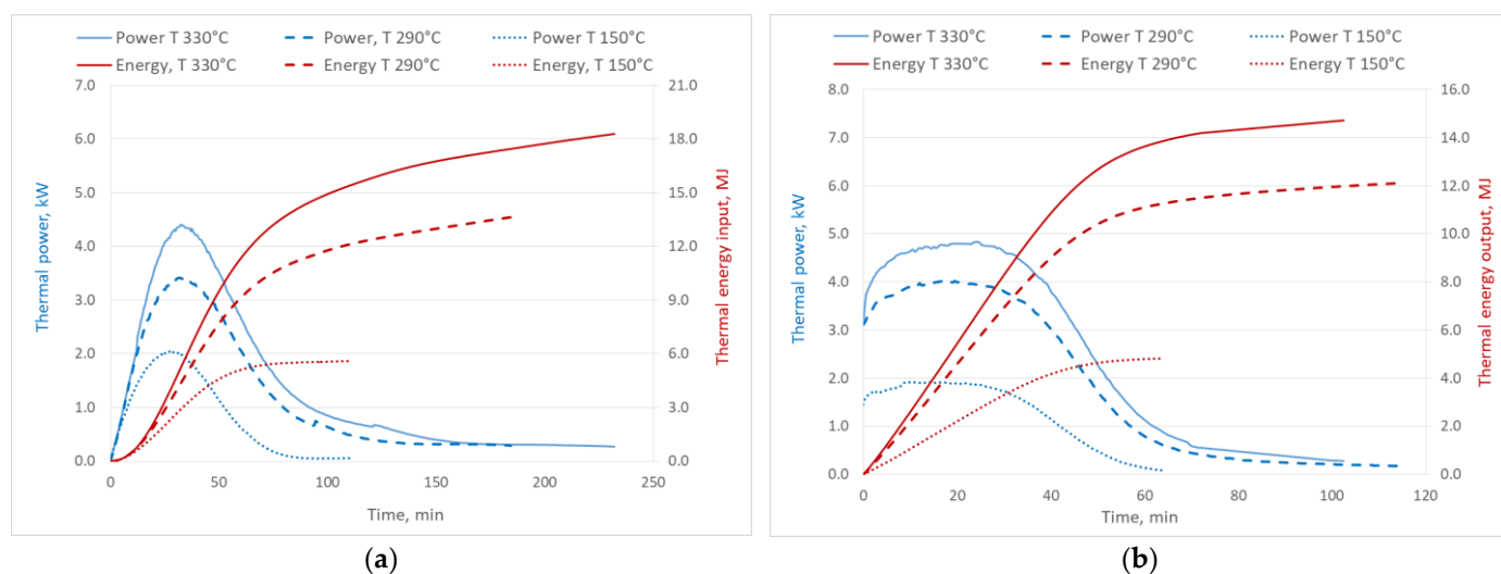
Figure 9. Thermal power and energy profiles of the TES unit depending on packed-bed temperature; (a) charging and (b) discharging. Air flow rate of 60 kg/h (tests B1, B4, B7).
