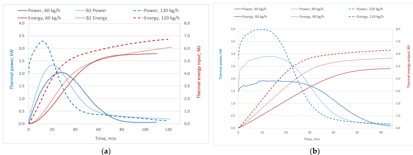
Figure 7. Thermal power and thermal energy input/output during (a) charging and (b) discharging, depending on air flow rates (60–120 kg/h). Target packed bed temperature of 150 °C.
