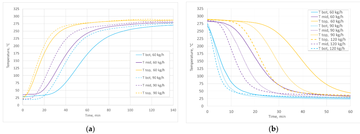
Figure A4. Temperature distribution during (a) charging and (b) discharging of the TES unit at various air flow rates. Target basalt packed-bed temperature of 290 °C (tests B4–B6).
