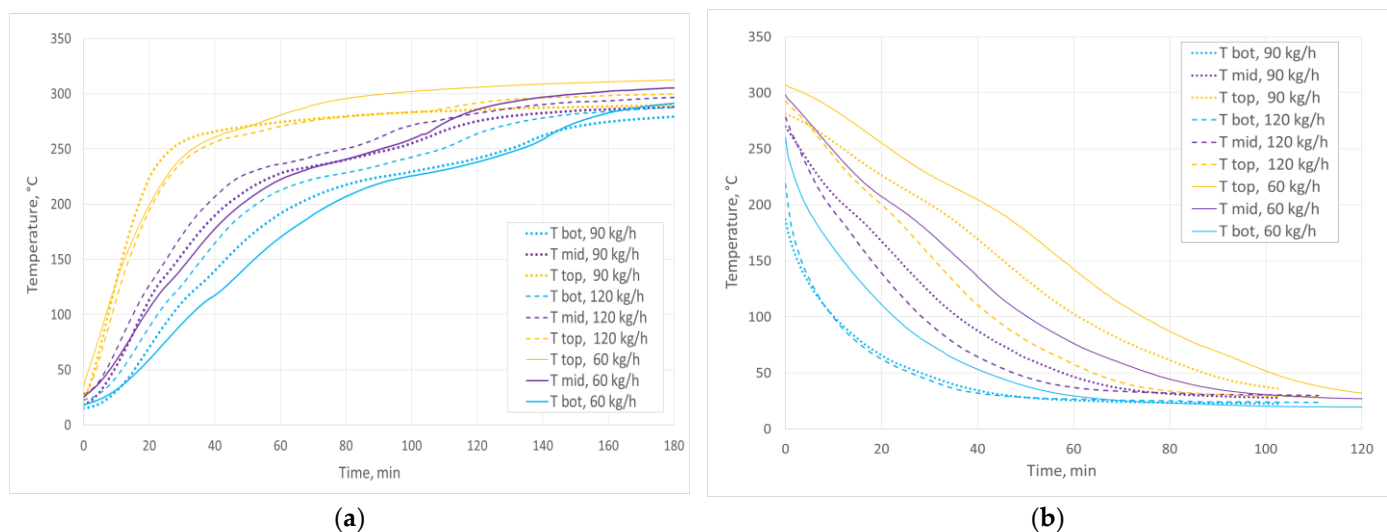
Figure 10. Comparison of axial temperature profiles for air flow rates of 90 kg/h and 120 kg/h during (a) charging and (b) discharging of PCM packed bed. Target packed-bed temperature of 290 °C.
