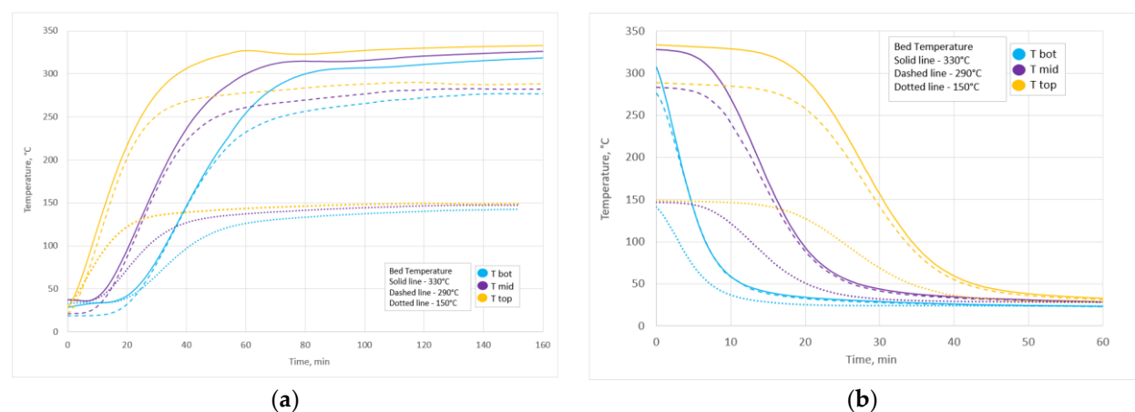
Figure A6. Temperature profiles of the TES unit depending on basalt packed-bed temperature; (a) charging and (b) discharging. Air flow rate of 90 kg/h (tests B2, B5, B8).
