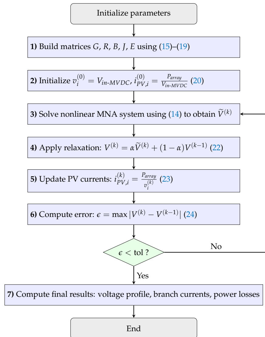
Figure 5. Flowchart of iterative nonlinear MNA solution applied to LPV MVDC collection network.
