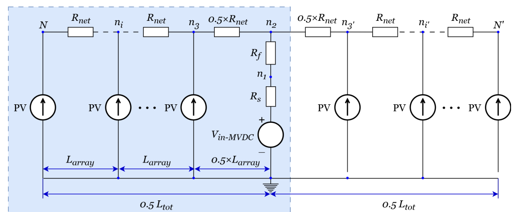
Figure 4. MNA formulation of MVDC collection network for LPV system.
