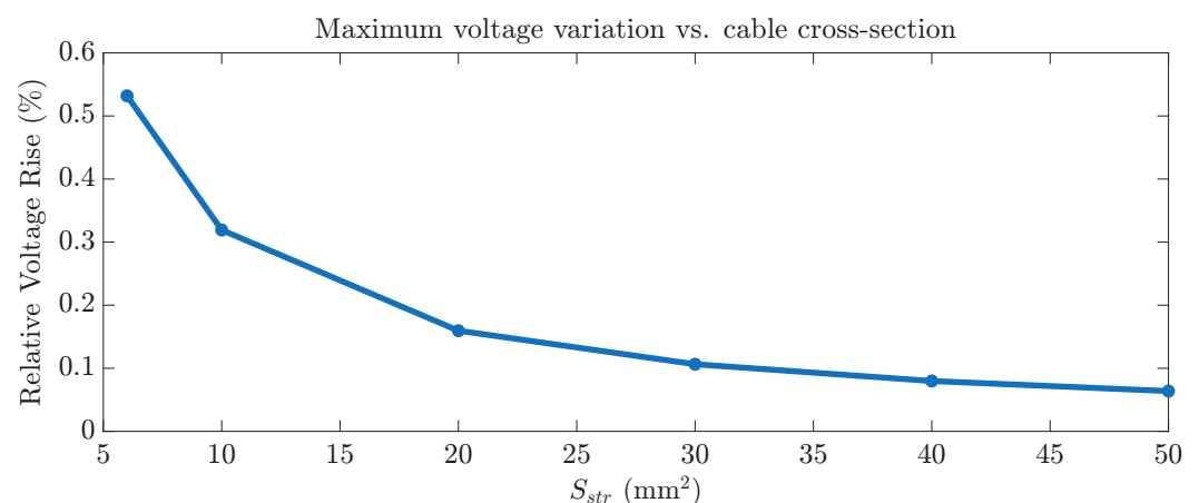
Figure 7. Maximum voltage variations at the most distant point under different cross sections.
