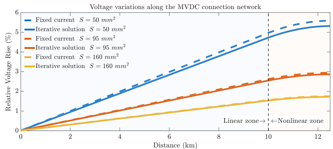
Figure 9. Relative voltage increase along the MVDC connection cable.
