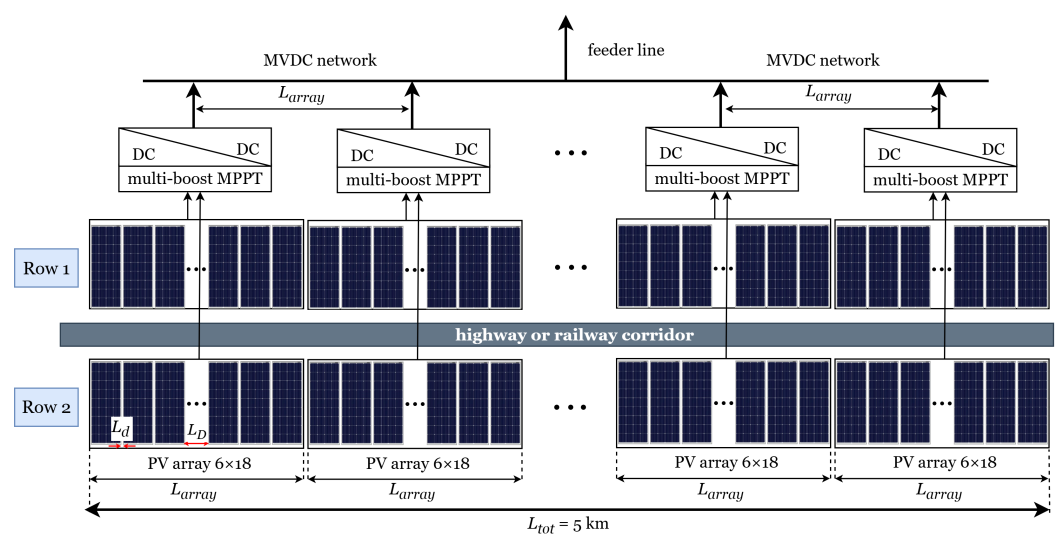
Figure 1. Physical layout design of two-row linear vertical PV power plant.
