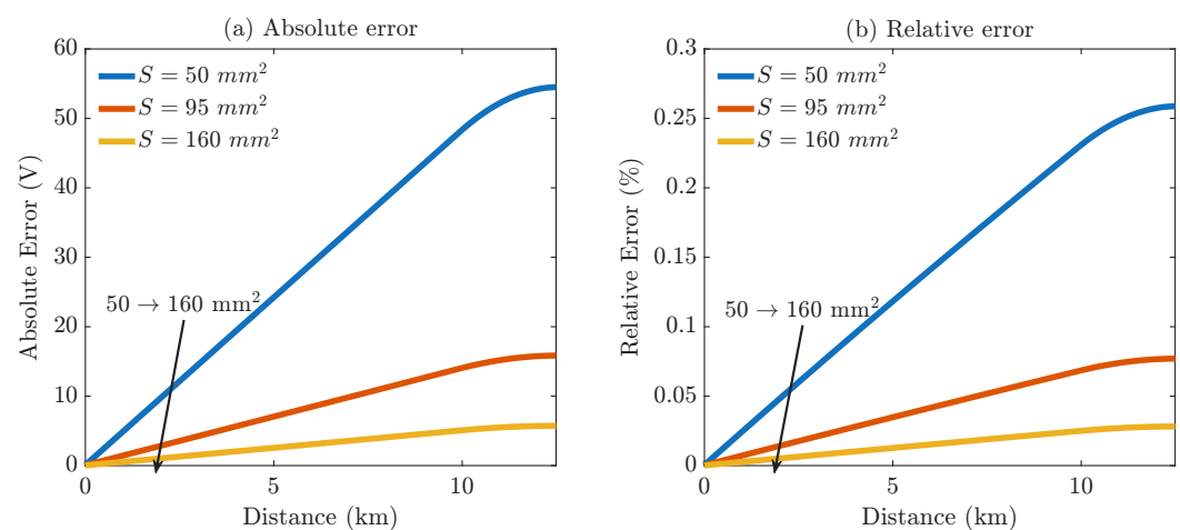
Figure 8. Comparison between fixed-current MNA and proposed iterative MNA.
