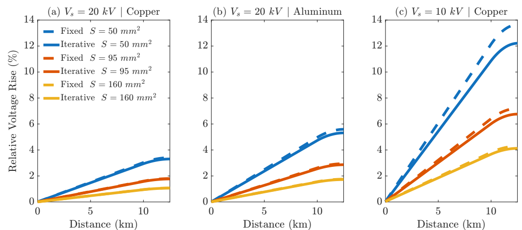
Figure 10. Comparative results: (a) Reference case, (b) different conductor materials comparison, (c) different voltage levels comparison.
