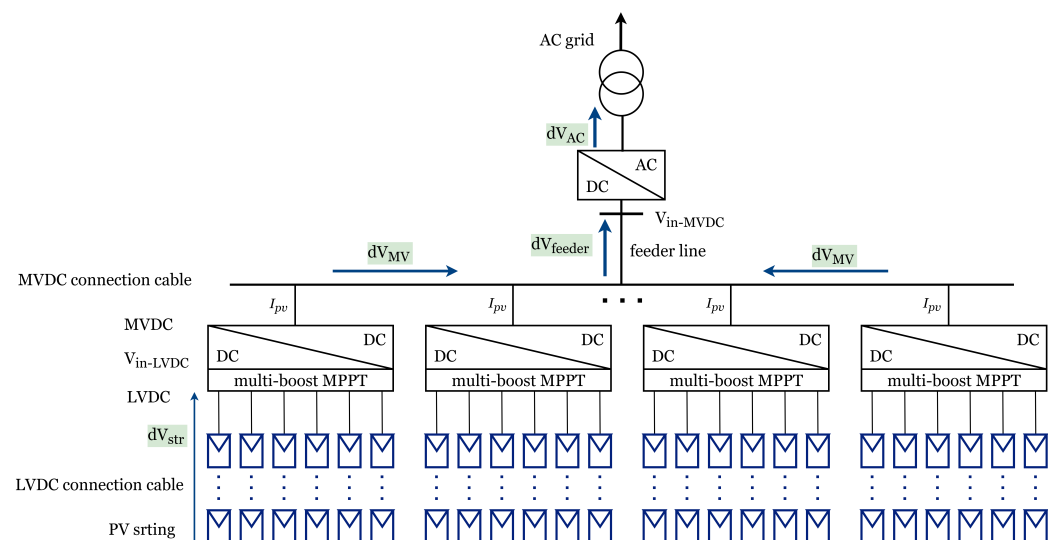
Figure 2. Global architecture design of LPV power plant using MVDC collection network.
