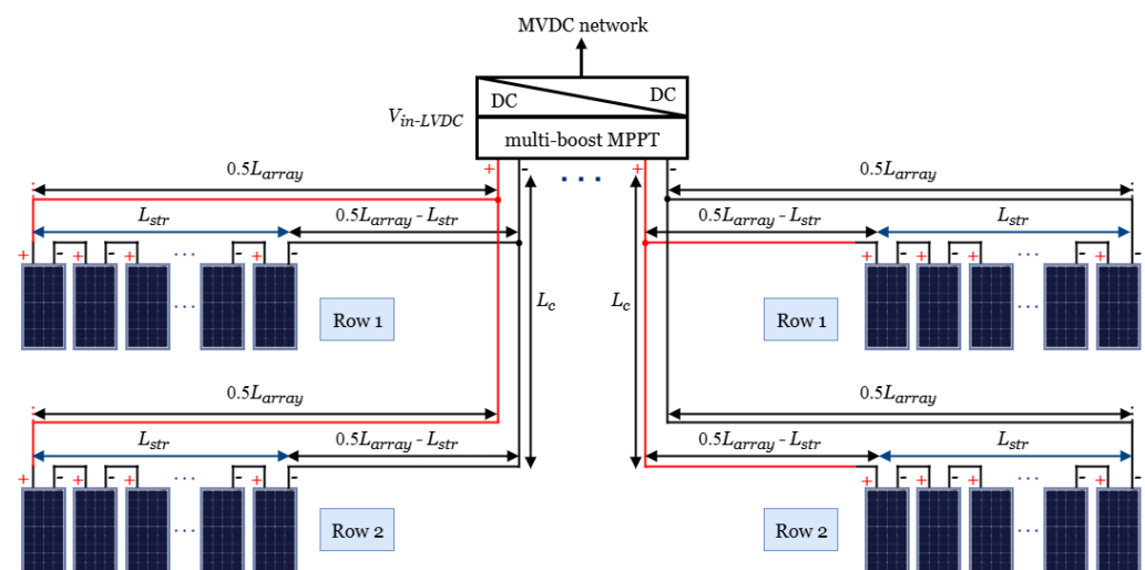
Figure 3. LVDC network configuration of PV string.
