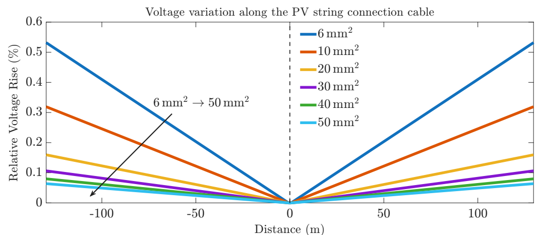
Figure 6. Relative voltage increase along the PV string connection cable.
