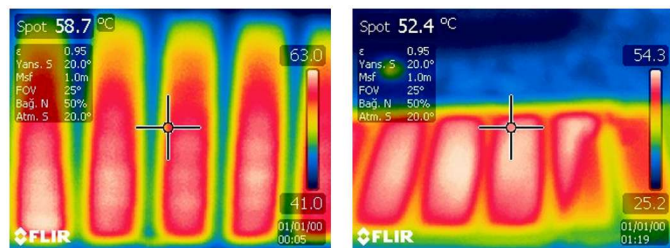
Figure 6. Thermal camera measurement of the smart glass-integrated PV module.
