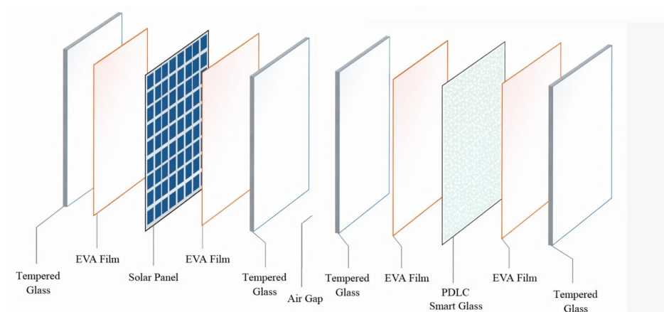
Figure 1. Cross-sectional structure of the system.
