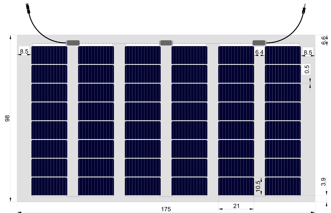
Figure 2. The cell layout geometry.
