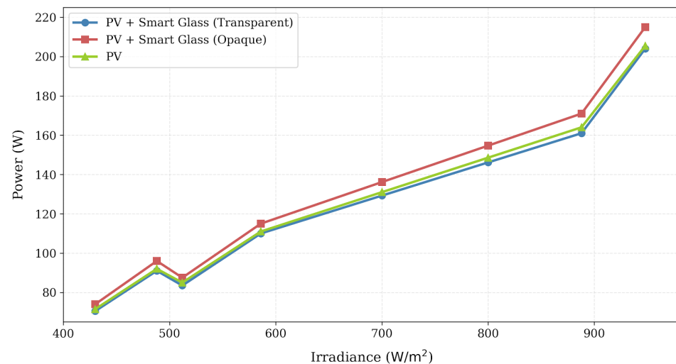
Figure 5. DC power output of three different PV configurations.
