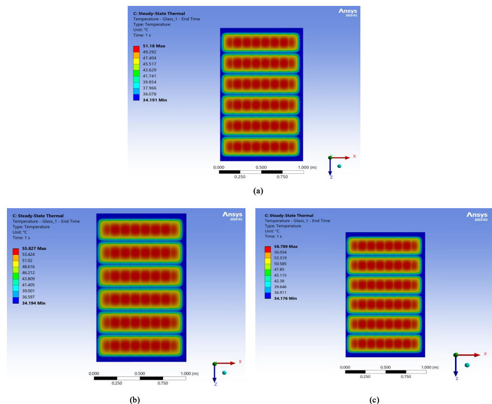
Figure 7. (a) ANSYS analysis of PV module, (b) ANSYS analysis of transparent mode of BIPV, (c) ANSYS analysis of opaque mode of BIPV.
