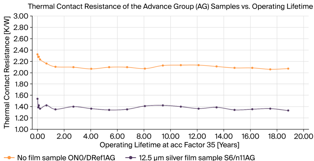
Figure 6. Two Advance Group samples' thermal contact resistances as a function of operating lifetime. "ON0/DRef1AG" sample without film and "S6/n11AG" sample with 12.5 µm silver film.
