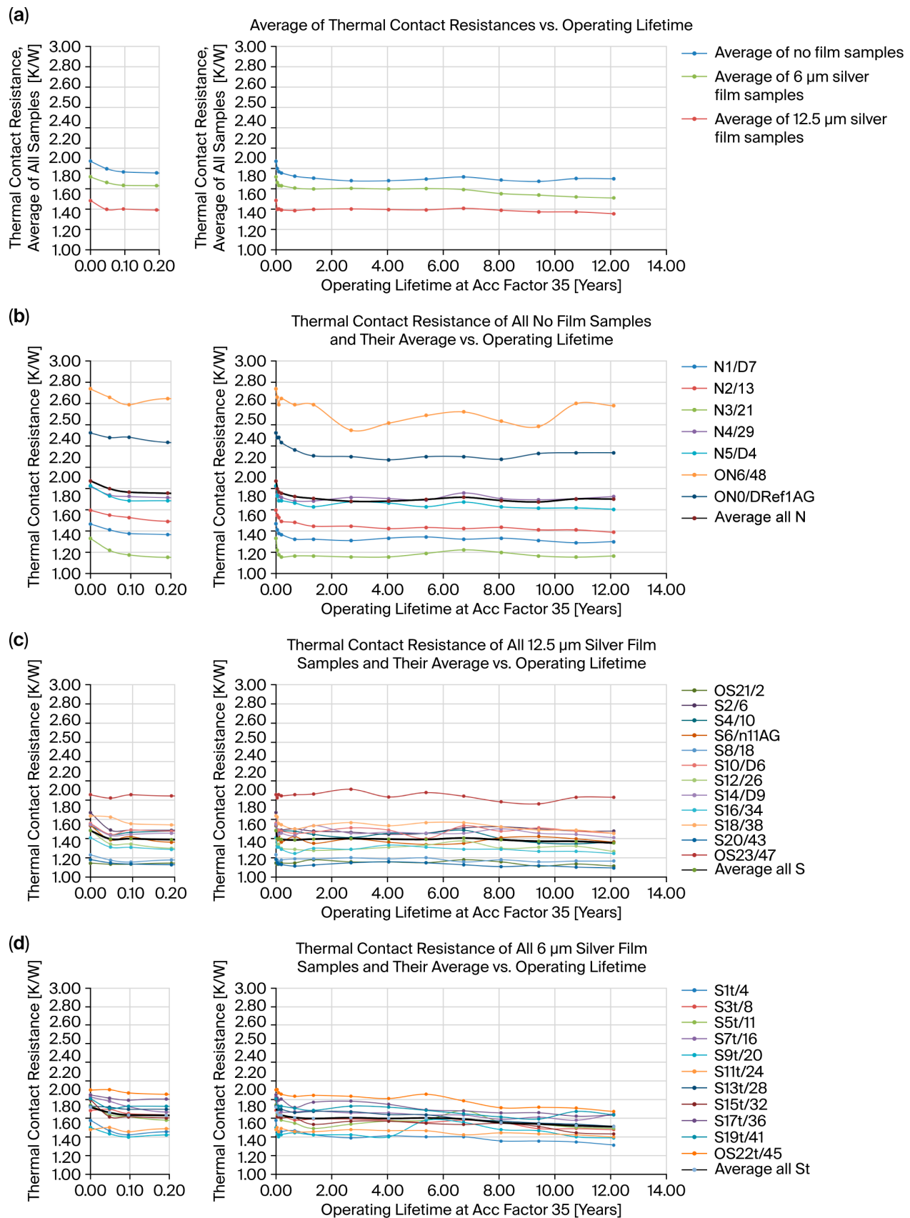
Figure 5. Thermal contact resistance behavior of 30 samples during 12.1 years of operating lifetime. (a) Film group averages of thermal contact resistance, (b) Thermal contact resistance for samples
