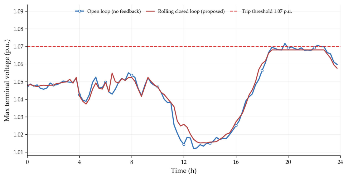
Figure 12. Maximum terminal voltage over time under wind-PV forecast error (heavy condition), for open-loop versus rolling closed-loop execution, with the 1.07 p.u. trip threshold.
