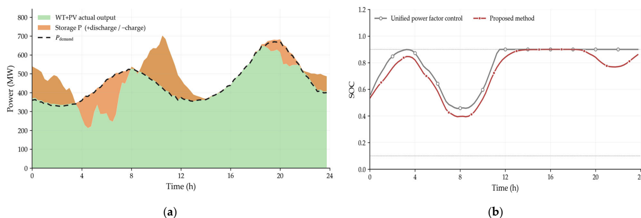
Figure 11. Operation of the base under the heavy condition: (a) active-power balance, showing WT+PV actual output, storage charging/discharging, and the active-power delivery schedule P_{demand} ; (b) base-average state of charge of the storage under the two methods. In (b), the gray and red curves denote unified power factor control and the proposed method, respectively. In panel (a), the black dashed curve denotes the active-power delivery schedule, P_{demand} .
