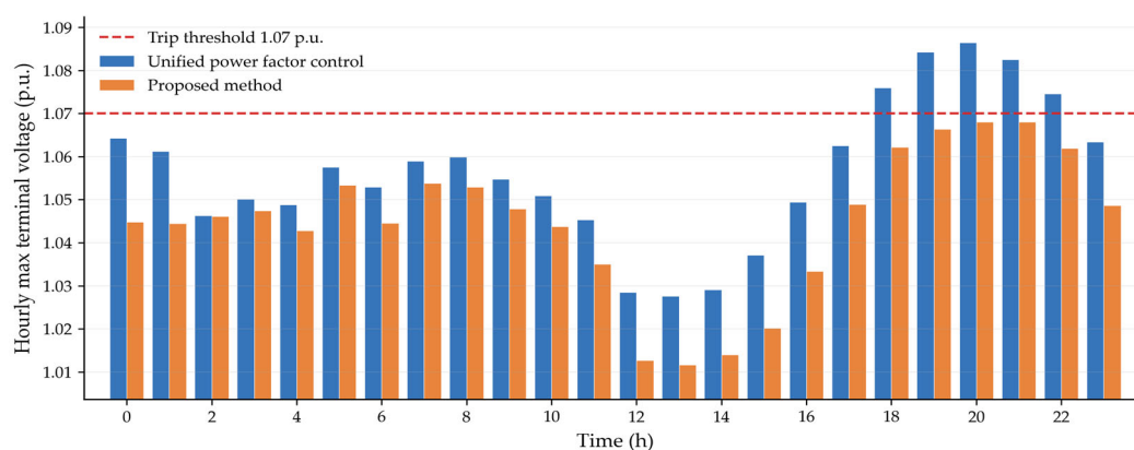
Figure 5. Hourly maximum terminal voltage under the typical condition.
