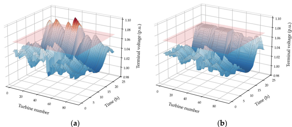
Figure 8. Terminal voltage of all 90 wind turbines over time under the heavy condition: (a) unified power factor control; (b) the proposed method. The semi-transparent red plane marks the 1.07 p.u. trip threshold. On the surface plots, blue-to-red shading denotes increasing terminal-voltage magnitude.
