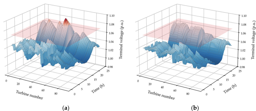
Figure 4. Terminal voltage of all 90 wind turbines over time under the typical condition: (a) unified power factor control; (b) the proposed method. The semi-transparent red plane marks the 1.07 p.u. trip threshold. On the surface plots, blue-to-red shading denotes increasing terminal-voltage magnitude.
