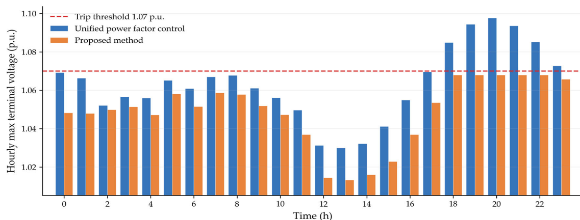
Figure 9. Hourly maximum terminal voltage under the heavy condition.
