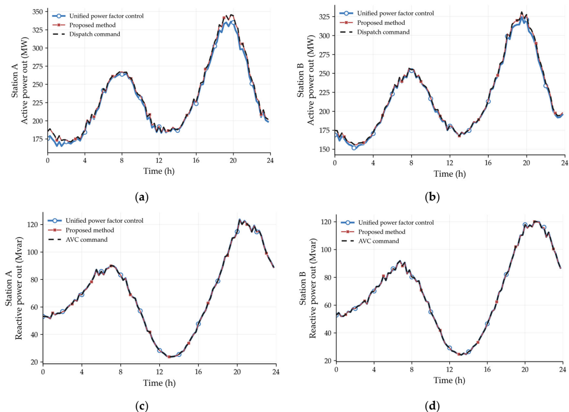
Figure 3. Delivery tracking curves of each station under the typical condition: (a) active power of Station A; (b) active power of Station B; (c) reactive power of Station A; (d) reactive power of Station B. In each panel, the blue, red, and black dashed lines denote unified power factor control, the proposed method, and the dispatch/AVC command, respectively.
