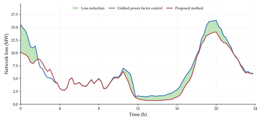
Figure 6. Time-series network loss of the base under the typical condition.
