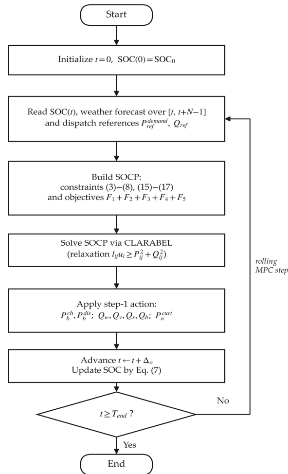
Figure 2. Flowchart of the rolling multi-period SOCP-MPC algorithm.
