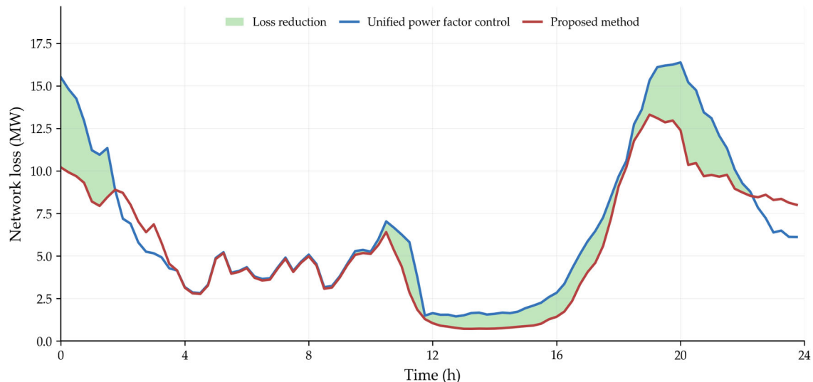
Figure 10. Time-series network loss of the base under the heavy condition.
