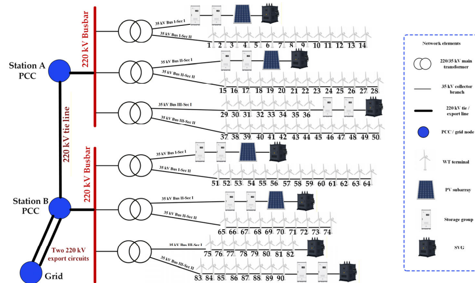
Figure 1. Wiring topology of the two series-coupled stations of the renewable energy base. The labels 1–90 denote the wind-turbine terminal numbers.
