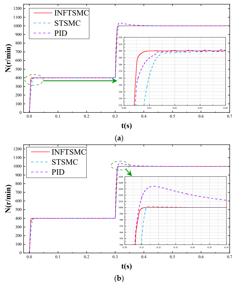
Figure 14. Speed–time curve under low torque and dynamic speed conditions: (a) start-up instant; (b) when the speed command suddenly increases.
