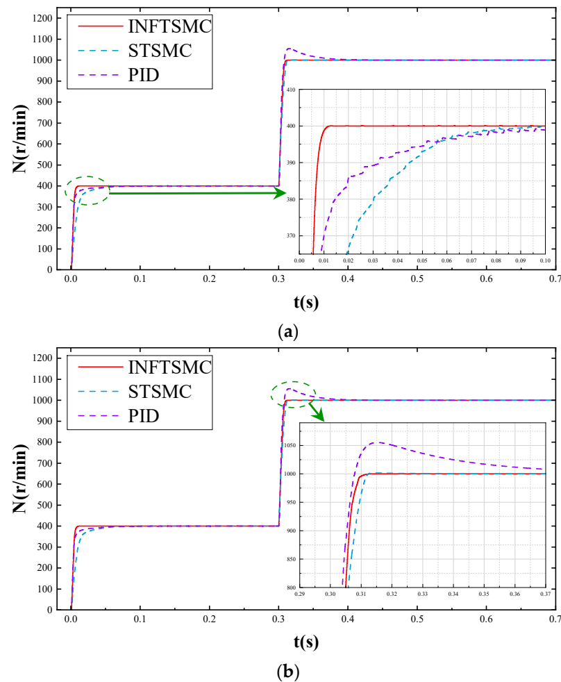
Figure 13. Speed–time curve under high torque and dynamic speed conditions: (a) start-up instant; (b) when the speed command suddenly increases.
