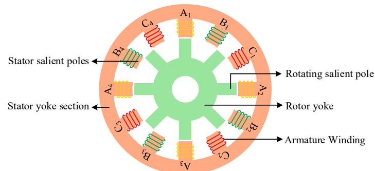
Figure 1. Structure of a typical 12/8-pole switched reluctance motor.
