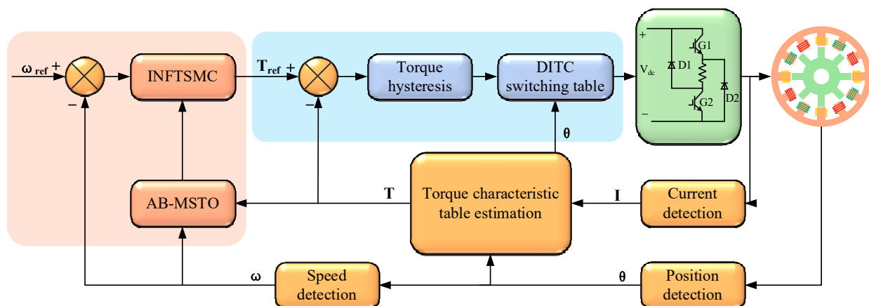
Figure 8. Overall block diagram of the INFTSMC and AB-MSTO.
