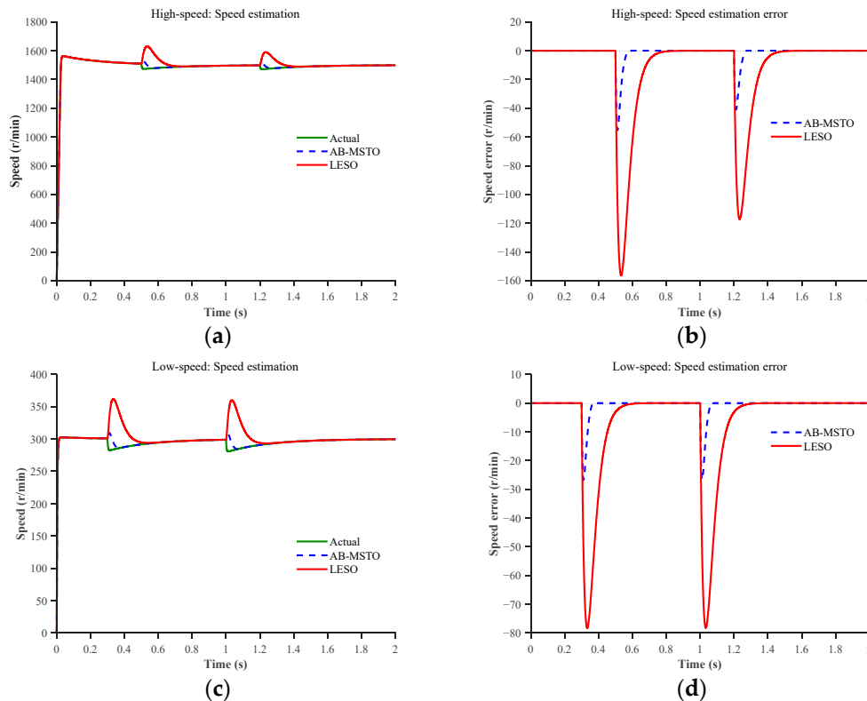
Figure 7. Estimation performance of AB-MSTO and LESO under different SRM operating conditions: (a) High-speed: Speed estimation; (b) High-speed: Speed estimation error; (c) Low-speed: Speed estimation; (d) Low-speed: Speed estimation error.
