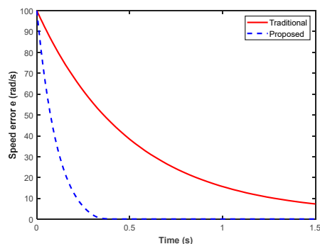
Figure 3. Comparison of the two sliding surfaces.
