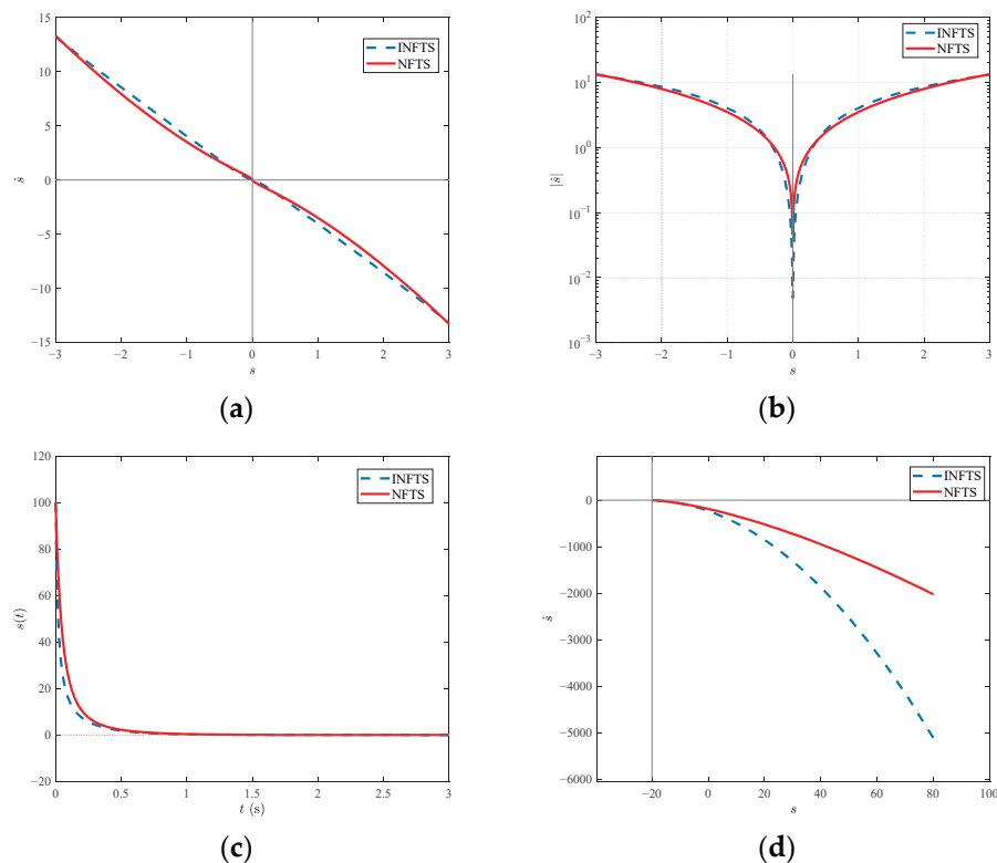
Figure 4. Comparison of INFTSMC and NFTSMC reaching laws in terms of (a) reaching law curves; (b) reaching speed; (c) sliding variable time response; (d) phase trajectory.
