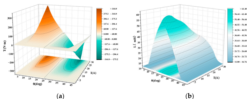
Figure 2. Characteristic curves: (a) torque characteristics; (b) inductance characteristics.
