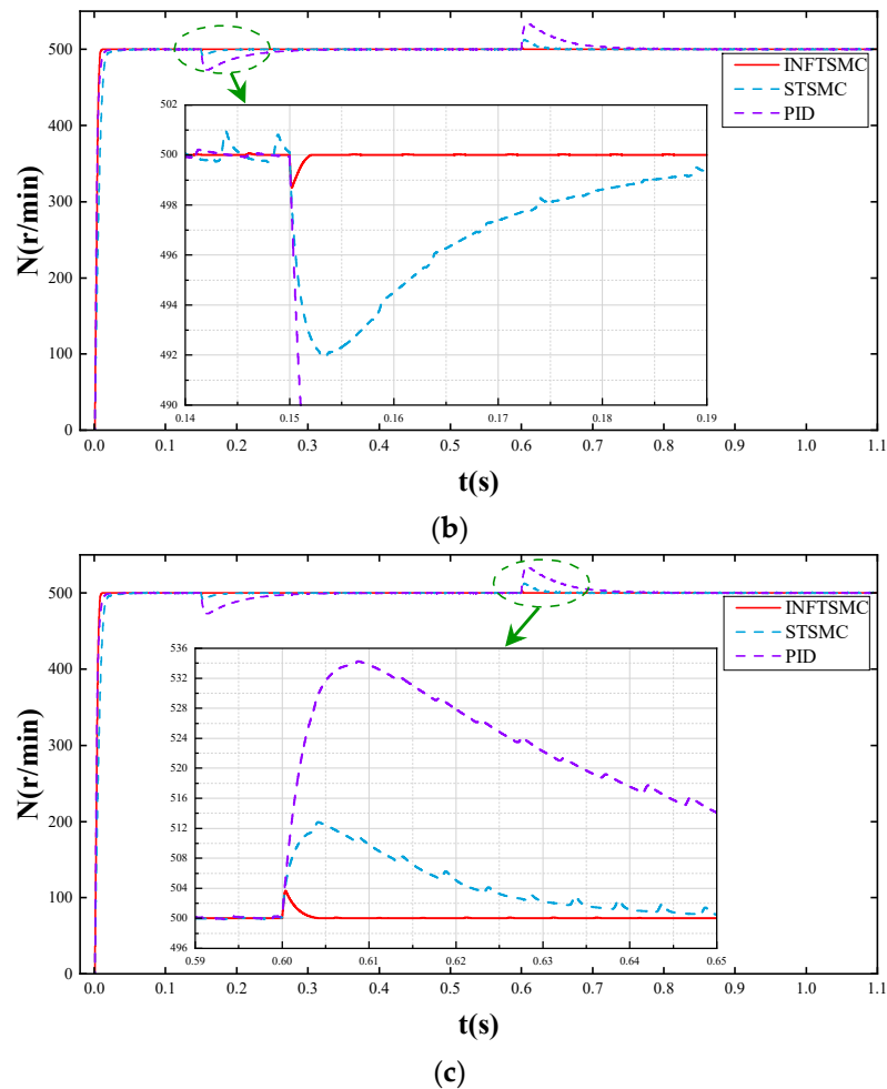
Figure 11. Speed–time curves under low-speed startup and dynamic load conditions: (a) start-up instant; (b) instant when the load torque suddenly increases; (c) instant when the load torque suddenly decreases.
