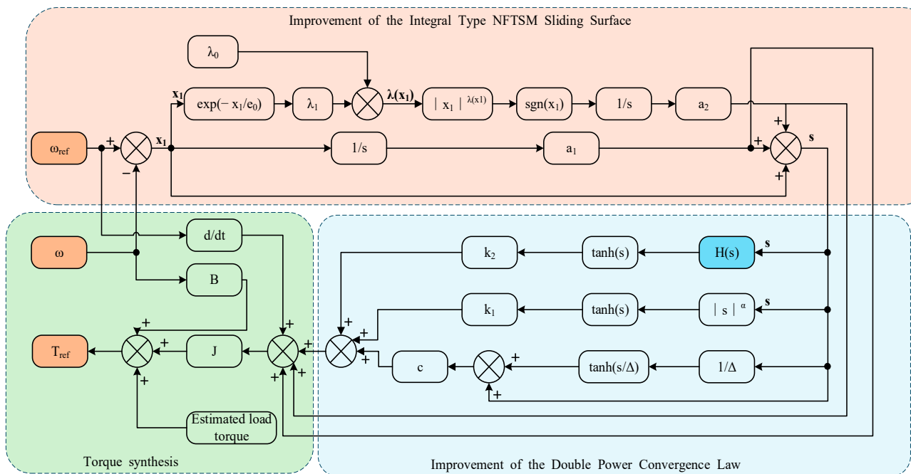
Figure 5. Block diagram of the improved nonsingular fast terminal sliding mode controller.
