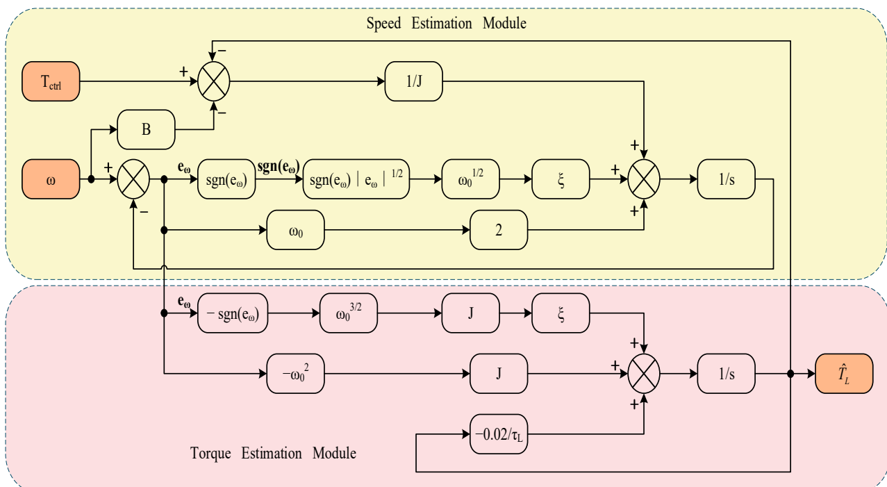
Figure 6. Structural diagram of the adaptive bandwidth modified super-twisting observer.
