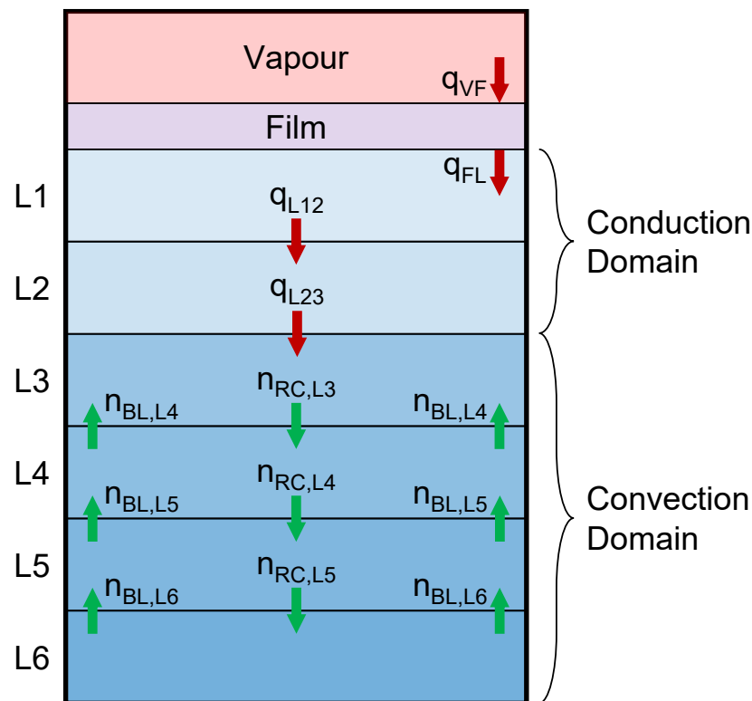
Figure 5. A tank containing a liquid phase divided into conduction and convection domains. Red arrows represent interlayer heat transfer, and green arrows represent liquid flows caused by convective circulation.
