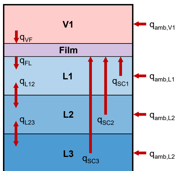
Figure 3. Categories of heat transfer considered in the model: ambient heat ingress into each layer (amb), interlayer heat transfer (VF, FL, L), and shortcut convection (SC).
