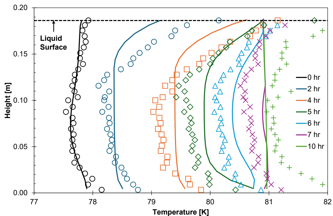
Figure 9. Liquid-phase temperature gradients for the first ten hours of LN 2 Experiment 1; the relief stage began at four hours. Symbols correspond to experimental data, and curves are model predictions.
