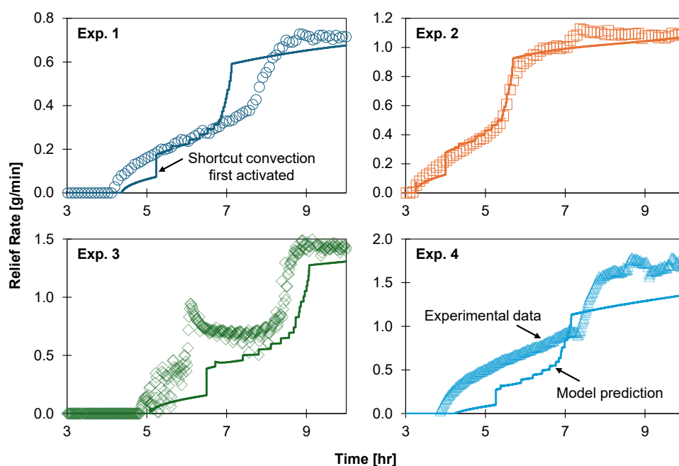
Figure 7. Relief rates during the transient relief stage for the LN 2 boil-off experiments. Symbols correspond to experimental data, and curves are model predictions.
