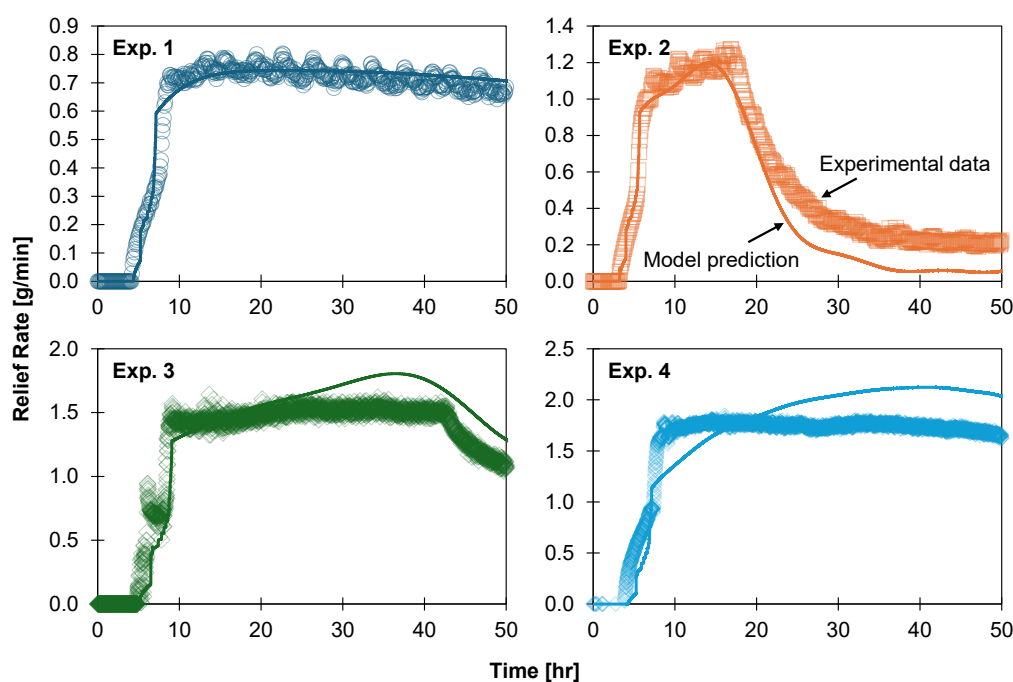
Figure 8. Relief rates for the LN 2 boil-off experiments. Symbols correspond to experimental data, and curves are model predictions.
