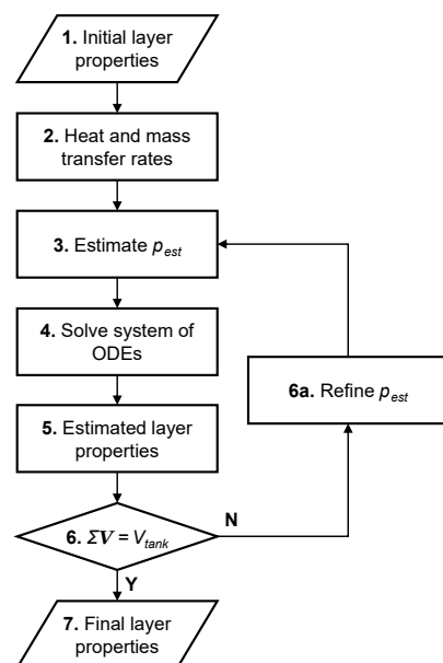
Figure 2. Simulation step algorithm used to calculate layer properties at the end of a timestep given the initial properties.
