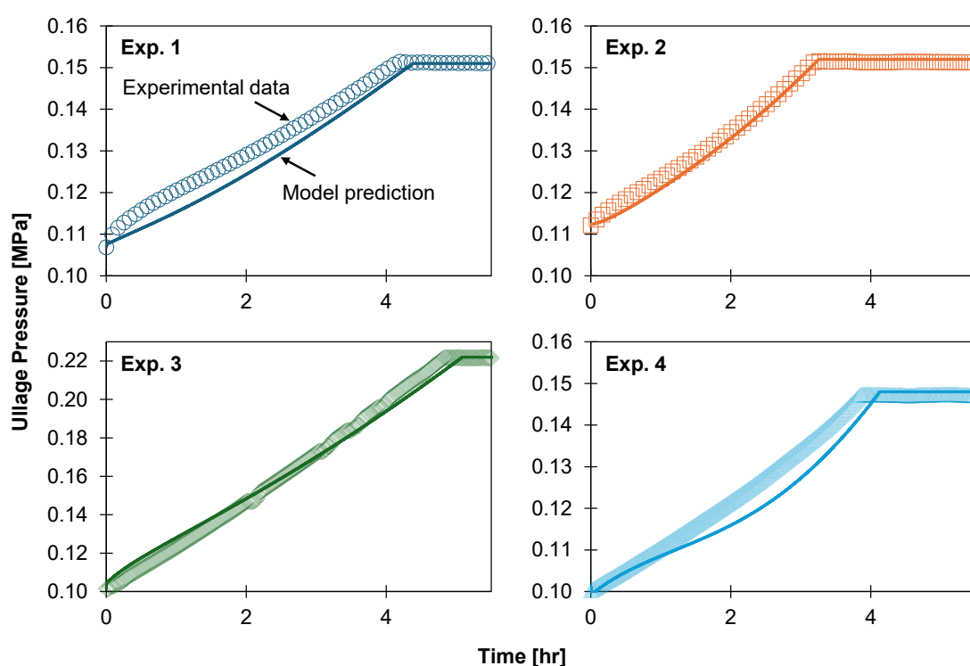
Figure 6. Ullage pressure during the pressurisation stage for the LN 2 boil-off experiments. Symbols correspond to experimental data, and curves are model predictions.
