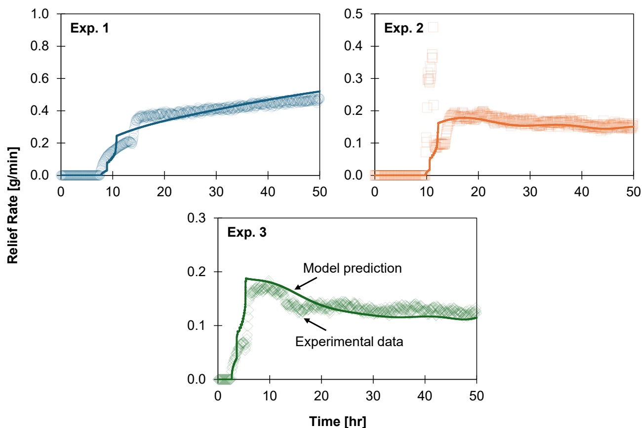
Figure 12. Relief rates for the LNG boil-off experiments. Symbols correspond to experimental data, and curves are model predictions.
