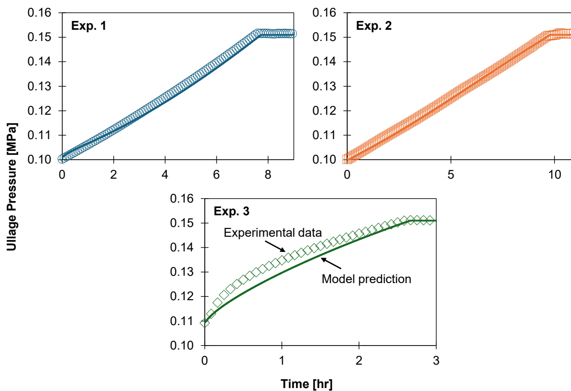
Figure 10. Ullage pressure during the pressurisation stage for the LNG boil-off experiments. Symbols correspond to experimental data, and curves are model predictions.
