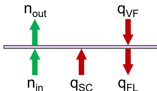
Figure 4. Energy balance on the film. Red arrows show heat transfer and green arrows show mass transfer: q_{VF} is heat entering the film from the vapour, q_{FL} is heat leaving the film for the liquid, and q_{SC} is the shortcut convection term.
