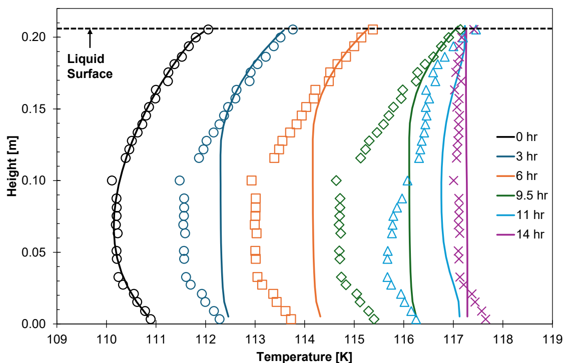
Figure 13. Liquid-phase temperature gradients for the first fourteen hours of LNG Experiment 2; the relief stage began at 9.5 h. Symbols correspond to experimental data, and curves are model predictions.
