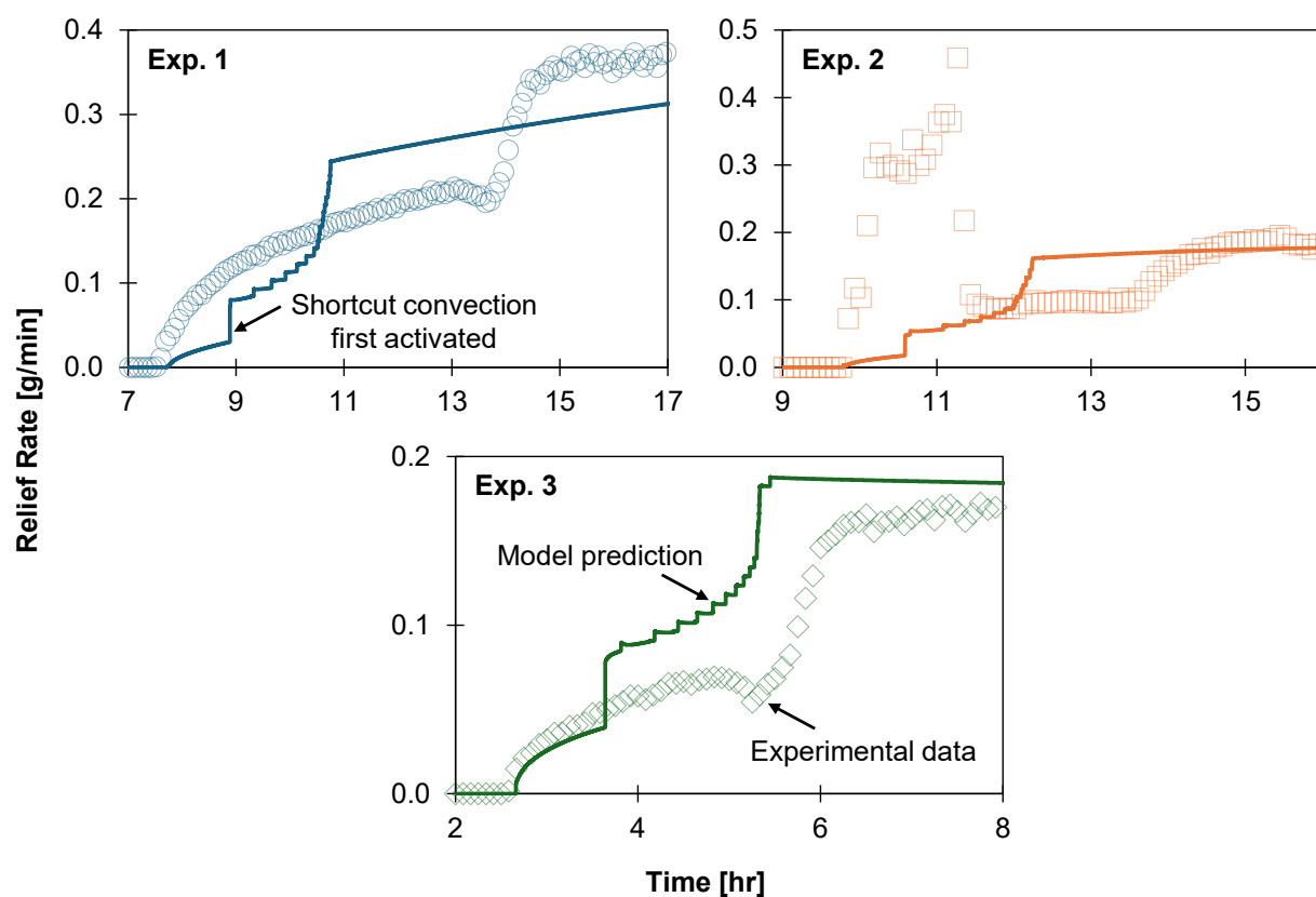
Figure 11. Relief rates during the transient relief stage for the LNG boil-off experiments. Symbols correspond to experimental data, and curves are model predictions.
