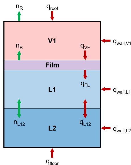
Figure 1. A tank containing vapour (in layer V1) and liquid (in layers L1, L2), with a film of saturated liquid located between them. This figure exaggerates film thickness: the model assumes it to be zero. Red arrows represent heat transfer, and green arrows represent mass transfer.
