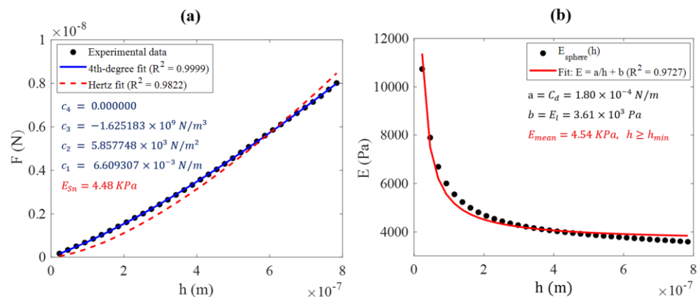
Figure 4. A representative force-indentation curve obtained from a H4 human glioma cell is shown in panel (a). The elastic modulus at each indentation depth was calculated using Equation (11), and the resulting depth-dependent modulus curve, E = f(h) , is presented in panel (b).
