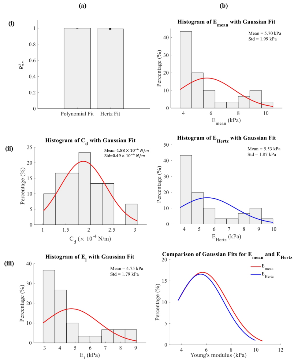
Figure 5. (ai) Bar charts of the R^2_{s.c.} for the fourth-degree polynomial and Hertzian fits, including error bars. The mean \pm standard deviation values were 0.99989 \pm 0.00008 for the polynomial fit and 0.99119 \pm 0.0055 for the Hertzian fit. (aii,aiii) Histograms of the stiffness coefficient C_d and limiting modulus E_l with Gaussian fits; the mean \pm standard deviation values are C_d = (1.88 \pm 0.49) \times 10^{-4} N/m and E_l = 4.75 \pm 1.79 kPa. (bi,bii) Distributions of E_{mean} and E_{Hertz} , corresponding to the mean modulus from the proposed model (Equation 17) and the Hertzian fit (Equation (18)), with mean \pm standard deviation values of E_{mean} = 5.70 \pm 1.99 kPa and E_{Hertz} = 5.53 \pm 1.87 kPa. (biii) Comparison of the Gaussian fits for E_{mean} and E_{Hertz} .
