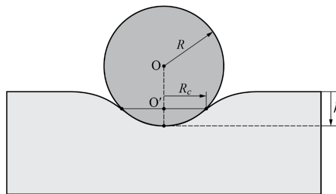
Figure A1. Deformation of elastic half space by a rigid sphere of radius R .
