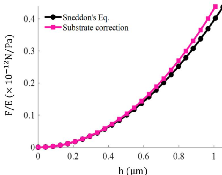
Figure 6. Comparison between the classic Sneddon equation for a perfect conical indenter acting on an elastic half-space and the Garcia and Garcia equation (Equation (19)), which accounts for the presence of a rigid substrate when testing a cell. The cell height was assumed to be 4.2\ \mu\text{m} , and the Poisson's ratio was \nu = 0.5 .
