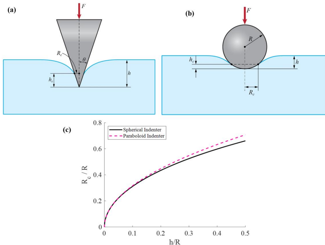
Figure 1. (a) Indentation using a conical indenter. (b) Indentation using a spherical indenter. The contact radius is presented in both cases. (c) Comparison of the normalized contact radius R_c/R as a function of the normalized indentation depth h/R for a spherical indenter (Equation (10)) and the parabolic approximation (Equation (12)). For small indentation depths ( h \ll R ), both approaches converge, yielding identical results as expected.
