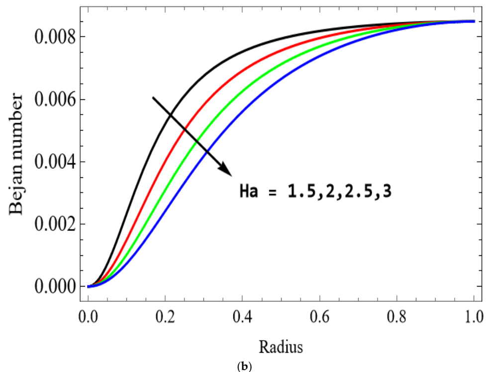
Figure 14. (a) Entropy generation for Ha . (b) Bejan number for Ha .
