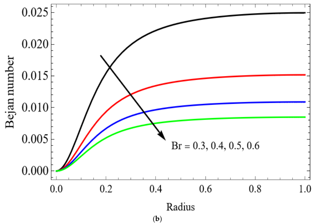
Figure 11. (a) Entropy generation for Br . (b) Bejan number for Br .
