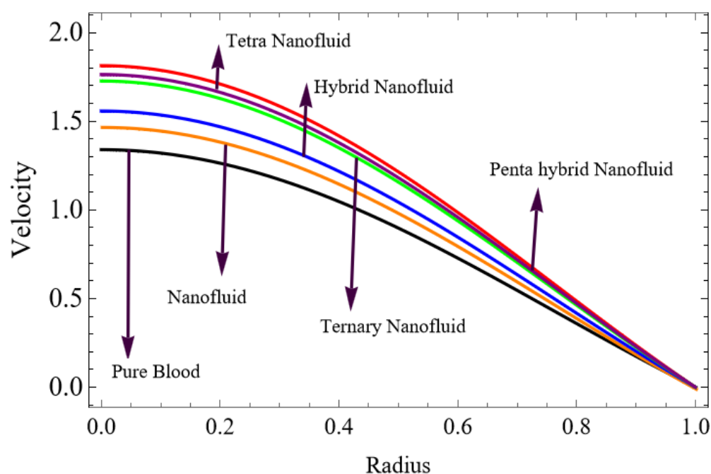
Figure 3. Velocity for Penta hybrid nanofluid.
