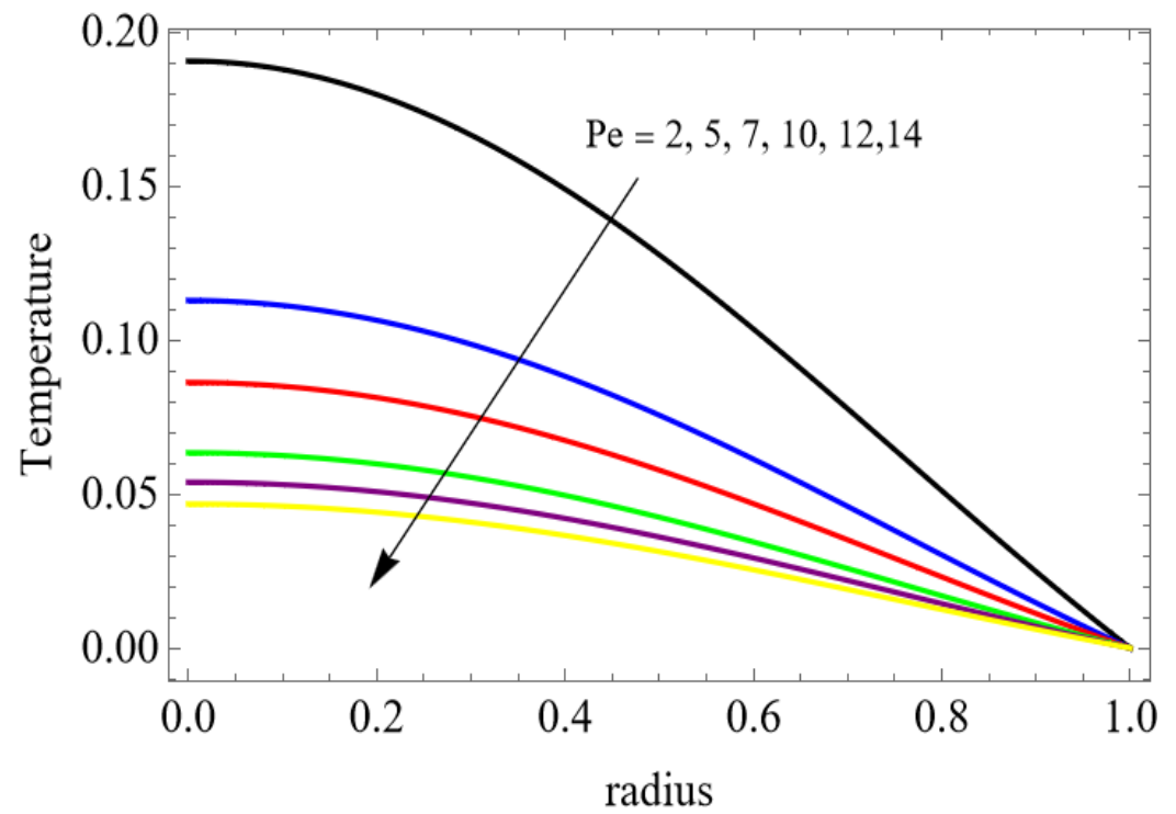
Figure 8. Temperature for Pe .
