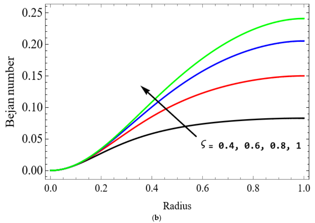
Figure 13. (a) Entropy generation for \zeta . (b) Bejan number for \zeta .
