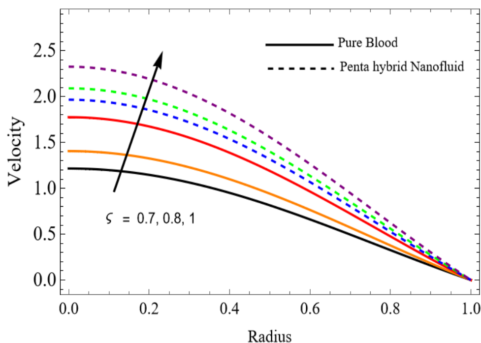
Figure 2. Velocity for \zeta .
