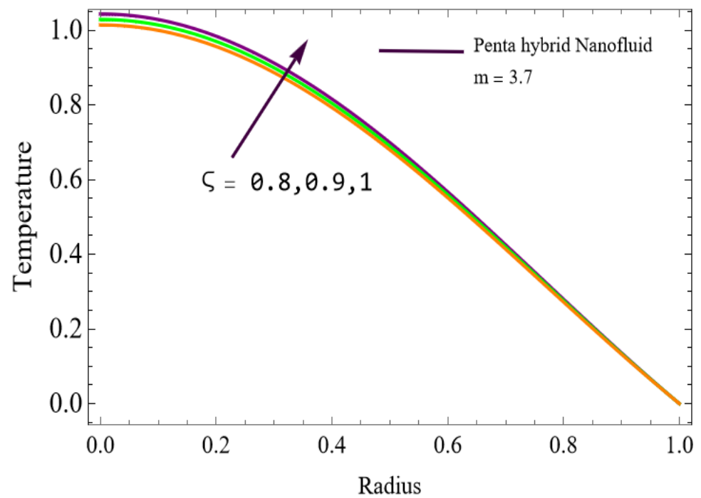
Figure 10. Temperature for \zeta .
