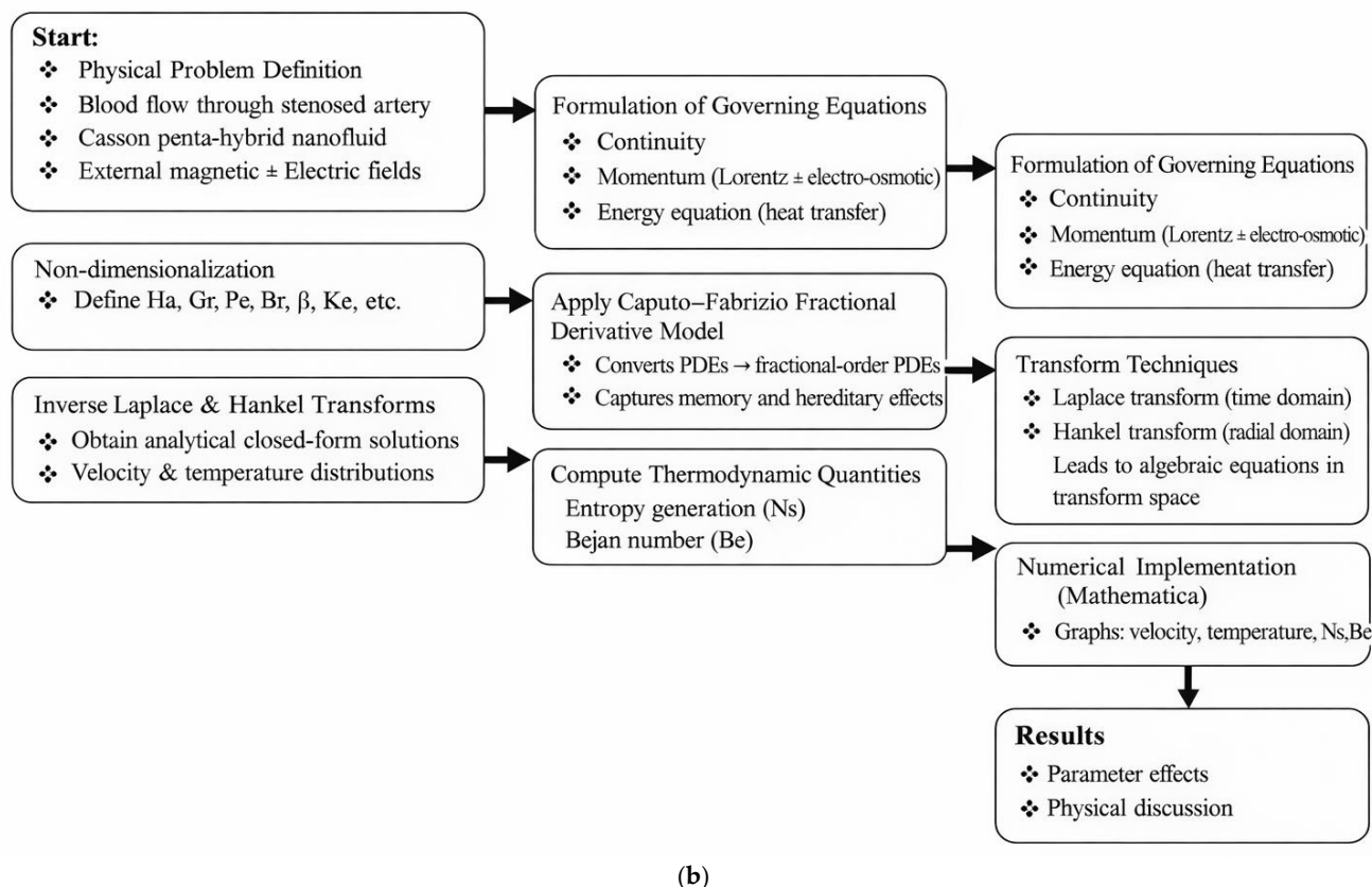
Figure 1. (a) Schematic of blood flow. (b) Flow chart.
