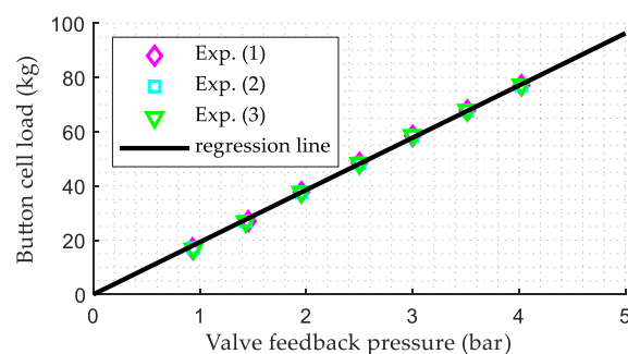
Figure 6. Calibration of the tread braking unit.
