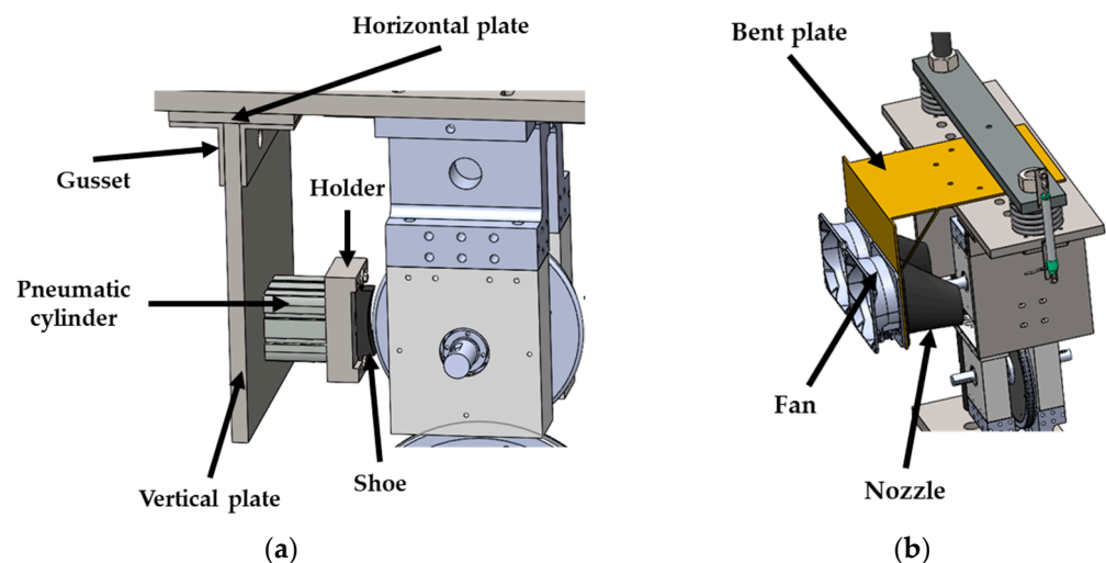
Figure 3. CAD model of the braking system: (a) braking unit; (b) cooling system.
