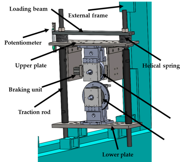
Figure 1. CAD model of the novel scaled twin-disc test rig.
