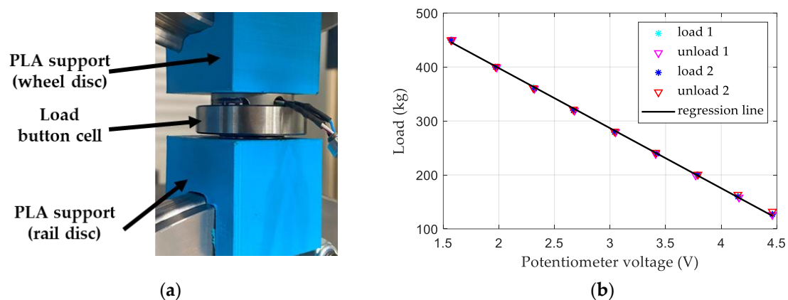
Figure 5. Calibration of the load application system: (a) positioning of the load button cell between PLA supports; (b) measured data with a regression curve.
