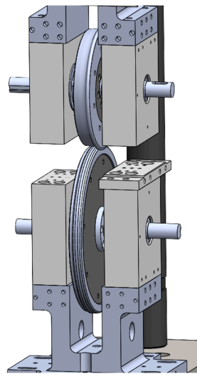
Figure 2. Detail of the contact between the rail ( lower ) and wheel ( upper ) rollers. See the hub and rim of each disc and the lateral profiles.
