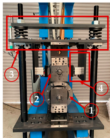
Figure 4. The 1:5-scale twin-disc test rig. (1) Rail disc, (2) wheel disc, (3) load application system, (4) braking unit.
