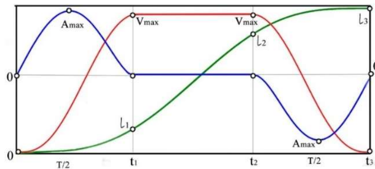
Figure 1. Polynomial-Based Motion Structure [11]. The blue, red, and green curves represent acceleration, velocity, and displacement, respectively.
