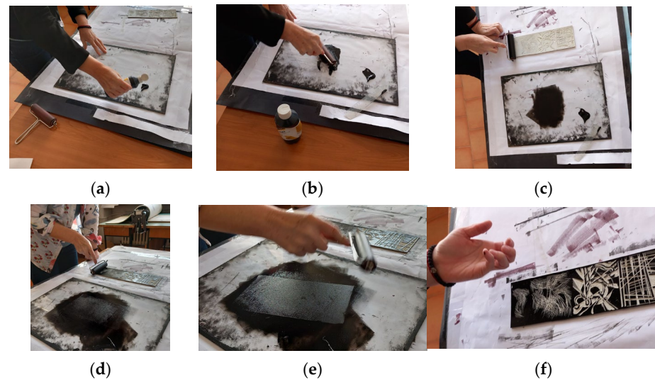
Figure 8. (a–f) Stages of the foundation inking workflow.
